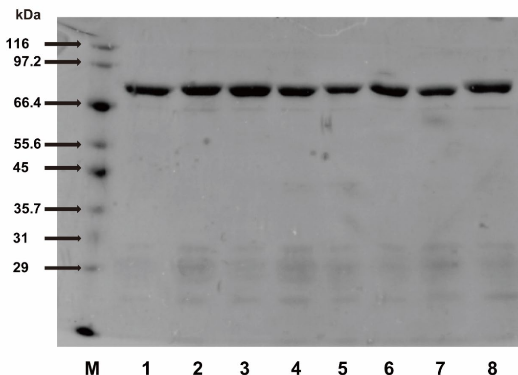
Fig. S1 SDS-PAGE of wild-type and chimeric IDHs. Five \mu g of proteins were applied into each lane. Lane M, marker proteins; lane 1, Pp WT; lane 2, Cm WT; lane 3, CPP; lane 4, PCC; lane 5, PCP; lane 6, CPC; lane 7, PPC; lane 8, CCP.
