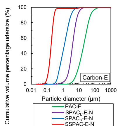
Fig. S1 – Particle size distributions of PACs, SPACs, and SSPACs.
