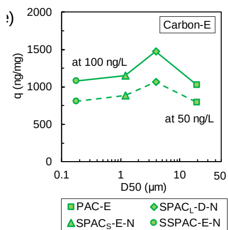
Fig. 3 – Plots of equilibrium MIB adsorption capacity versus AC particle size. Squares indicate PAC, diamonds indicate SPAC L , triangles indicate SPAC S , and circles indicate SSPAC. The adsorption capacities are given as solid-phase concentrations ( q ) at the equilibrium liquid-phase concentrations of 50 or 100 ng/L.
