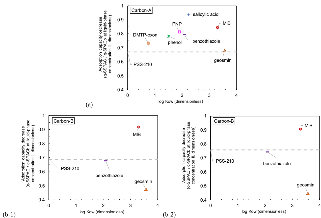
Fig. S9 – Plots of ratios of SPACs and SSPAC adsorption capacities versus adsorbate log Kow. Adsorbate concentrations I and II (panels b-1 and b-2, respectively): MIB and geosmin, 50 and 100 ng/L; DMTP-oxon, 5 and 10 µg/L; benzothiazole, phenol, para -nitrophenol (PNP), and salicylic acid, 0.5 and 1 mg/L; PSS-210, 2 and 4 mg/L. The ratios for PSS-210 are indicated by the dashed lines because the log Kow value is unavailable.
