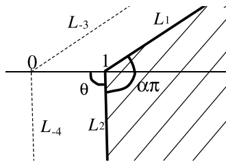
Figure 2. The image of \mathbb{C}_+ under the map z \mapsto 1 - s(-\frac{1}{z})^\alpha . L_1 and L_2 are half lines contained in the upper half-plane and the lower half-plane, respectively. L_{-3} and L_{-4} are preimages of L_3 and L_4 of Figure 3 for the map z \mapsto z^{1/r} , respectively.
