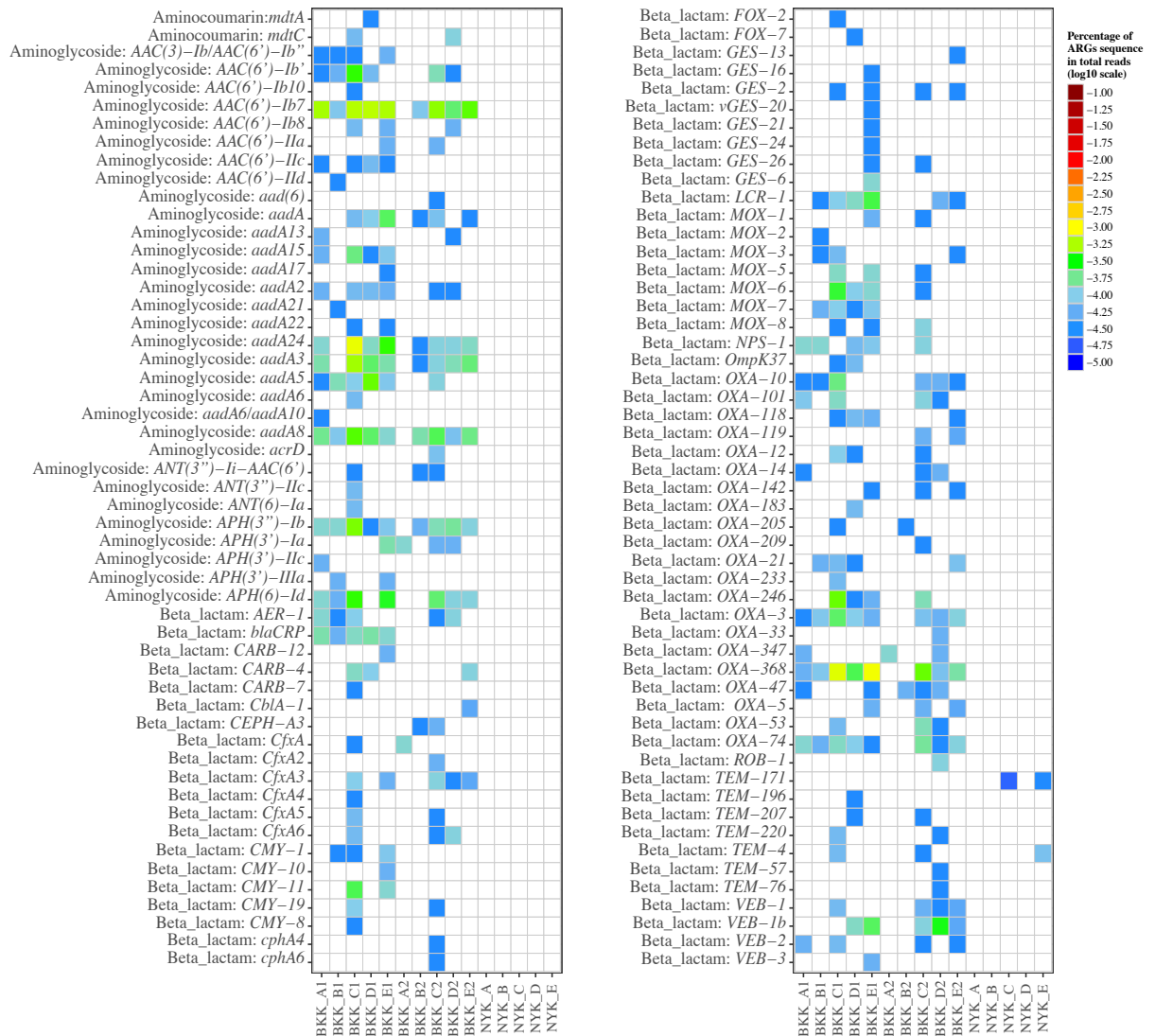
Figure 13. The abundance of ARGs classified by gene levels in samples collected from Phadungkrungkasem Canal and a rice field. BKK and NYK samples were collected from Phadungkrungkasem Canal (urban area) and a rice field (rural area). The ARGs were identified using a blastn search against the ARG database. The ARGs were grouped by the same gene and represented by colored squares. White squares represent no read of ARGs is detected.
