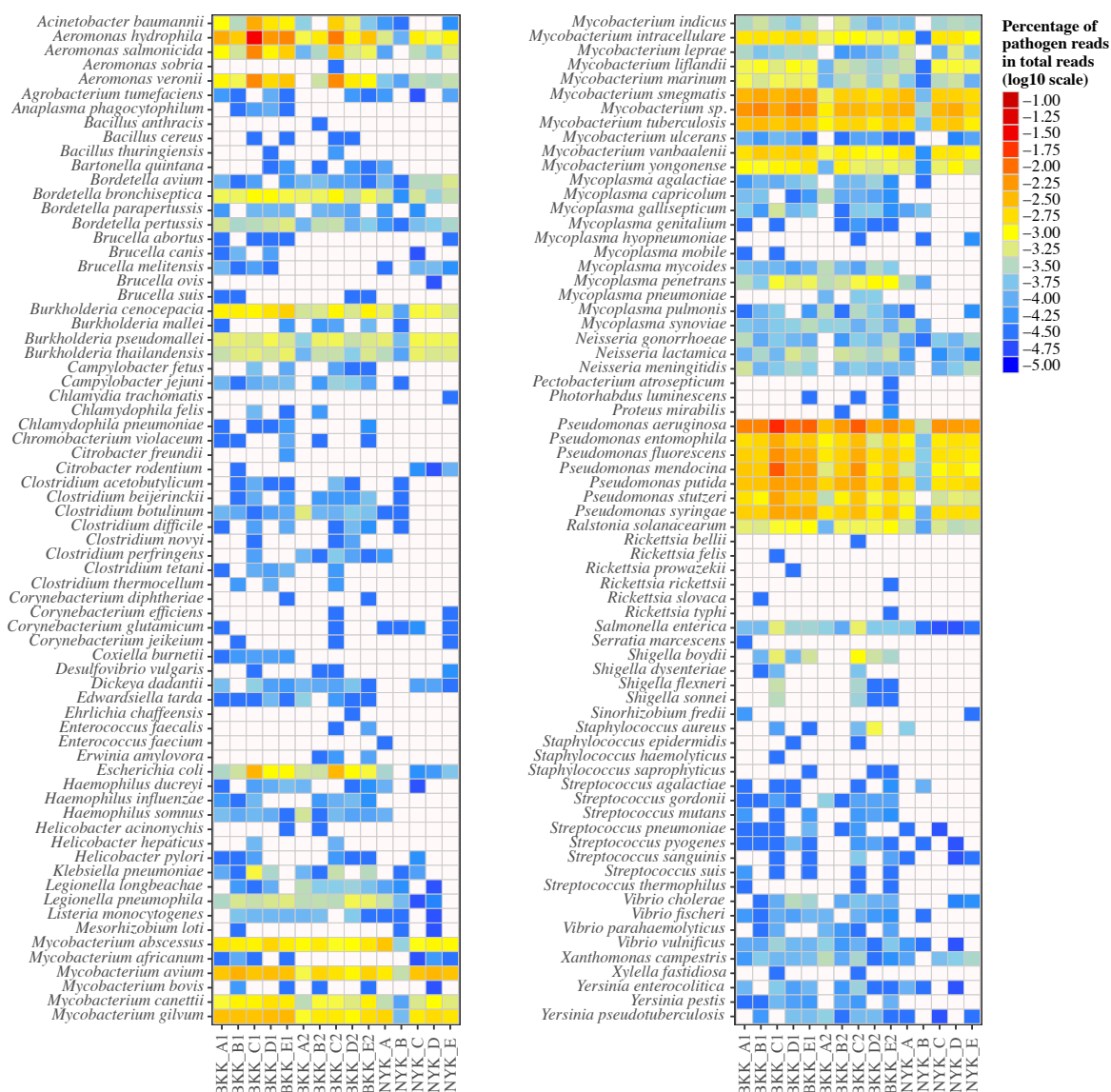
Figure 10. Potential pathogens in samples from Phadungkrungkasem Canal and a rice field detected by a blastn search against the VFDB database. BKK and NYK samples were collected from Phadungkrungkasem Canal (urban area) and a rice field (rural area). The proportion of potential pathogens was calculated using the number of reads identified as potential bacteria divided by the total number of reads generated by NGS. Color squares represent the abundance of reads identified as pathogenic bacteria ranging from -1.00 to -5.00 on a log 10 scale. White squares represent no read detected for each pathogen.
