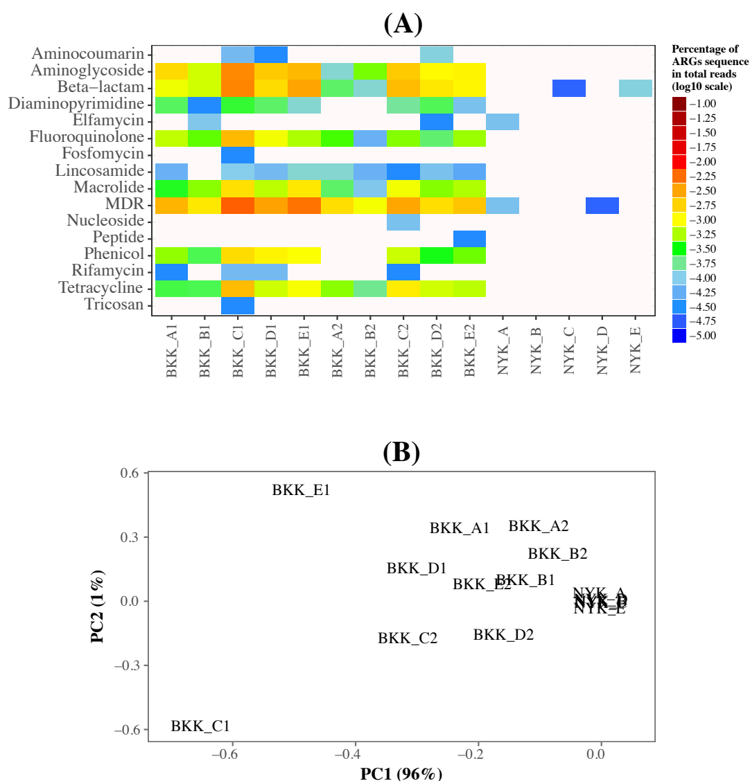
Figure 12. The abundance of ARGs classified by drug class in samples collected from Phadungkrungkasem Canal and a rice field. BKK and NYK samples were collected from Phadungkrungkasem Canal (urban area) and a rice field (rural area). The ARGs were identified using a blastn search against a CARD database. (A) Abundance of ARGs classified by antibiotic class. (B) PCA of ARGs classified by drug class. BKK samples were collected from an urban area, while NYK samples were collected from a rural area.
