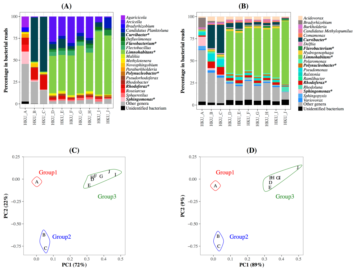
Figure 4. Bacterial communities at the genus level in water samples determined by the naïve LCA algorithm in MEGAN. (A) Bacterial communities based on the results of a blastn search of 16S rRNA amplicon reads against nucleotide sequences from the NCBI-16SMicrobial-NT database. (B) Bacterial communities based on the results of the blastn search of shotgun reads against nucleotide sequences from the NCBI-NT database. Color bars represent the top 20 abundant genera in all samples. Reads from other minor genera are represented in gray, and the reads with unidentified genera are represented in black. The genera ranked in top 20 in both 16S rRNA amplicon and shotgun metagenomic analyses are indicated with asterisks. Unclassified reads at genus level were presented as unidentified bacterium. The results of principal component analysis of the bacterial communities using 16S rRNA reads and shotgun reads are shown in panel (C) and (D), respectively.
