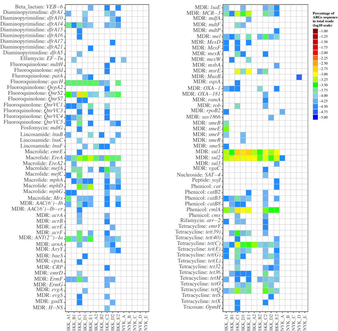
Figure 13. (continued) The abundance of ARGs classified by gene levels in samples collected from Phadungkrungkasem Canal and a rice field. BKK and NYK samples were collected from Phadungkrungkasem Canal (urban area) and a rice field (rural area). The ARGs were identified using a blastn search against the ARG database. The ARGs were grouped by the same gene and represented by colored squares. White squares represent no read of ARGs is detected.
