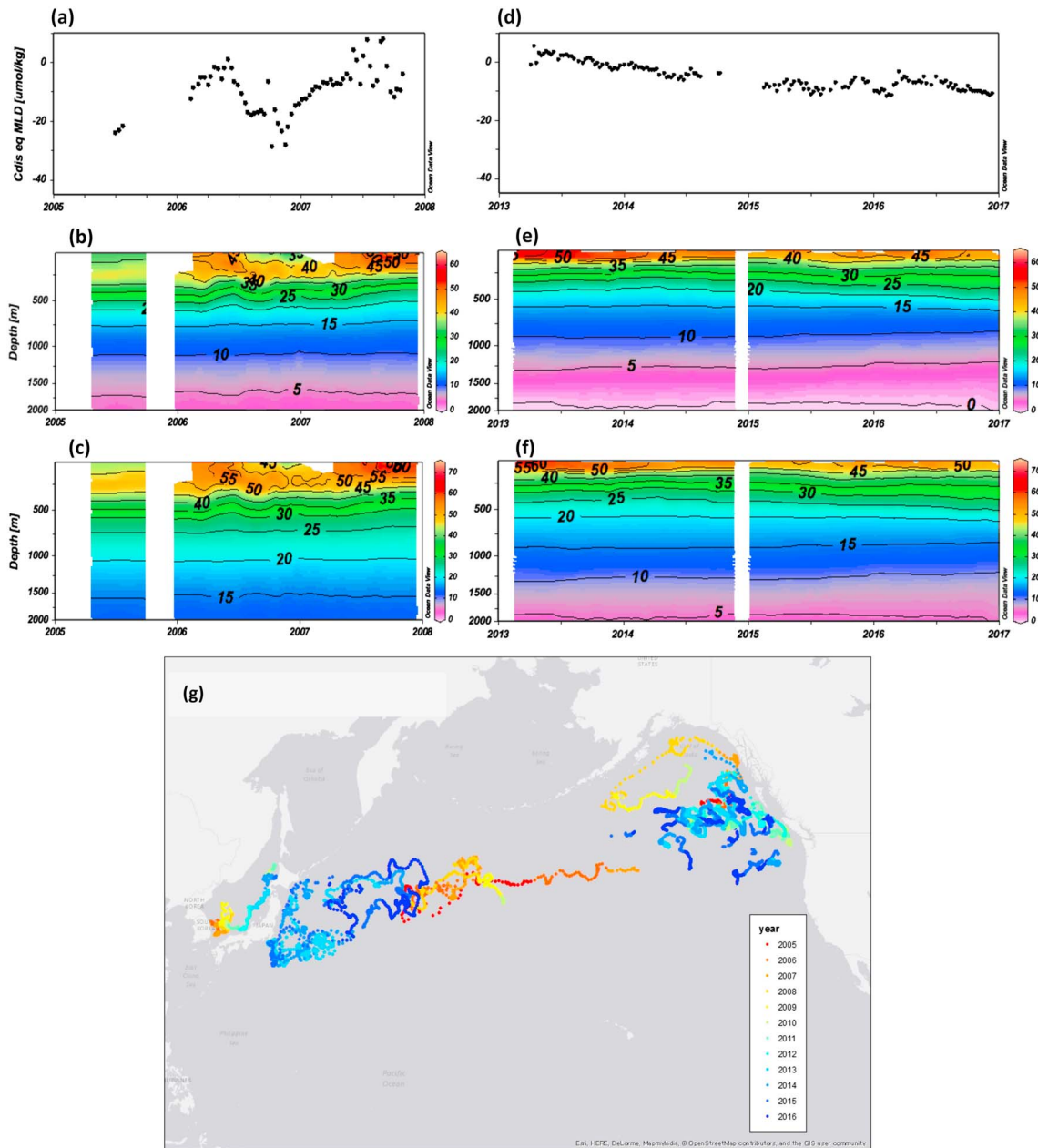
Figure 2. Vertical distributions of (a, d) C_{diseq, MLD} (μmol/kg), (b, e) C_{res} (μmol/kg), and (c, f) C_{ant} (μmol/kg) predicted by applying new parameterizations to DO, T, and S data from Argo profiling floats 2900540 and 5904106, respectively. The vertical axis of (b, e, c, f) has been stretched at the top part of each panel. Figures 2a–2f were drawn using Ocean Data View ( http://odv.awi.de ). (g) BGC-Argo float trajectories in the subarctic North Pacific with trajectories in different years shown by colored dots. MLD = mixed layer depth; BGC-Argo = biogeochemical Argo float.
