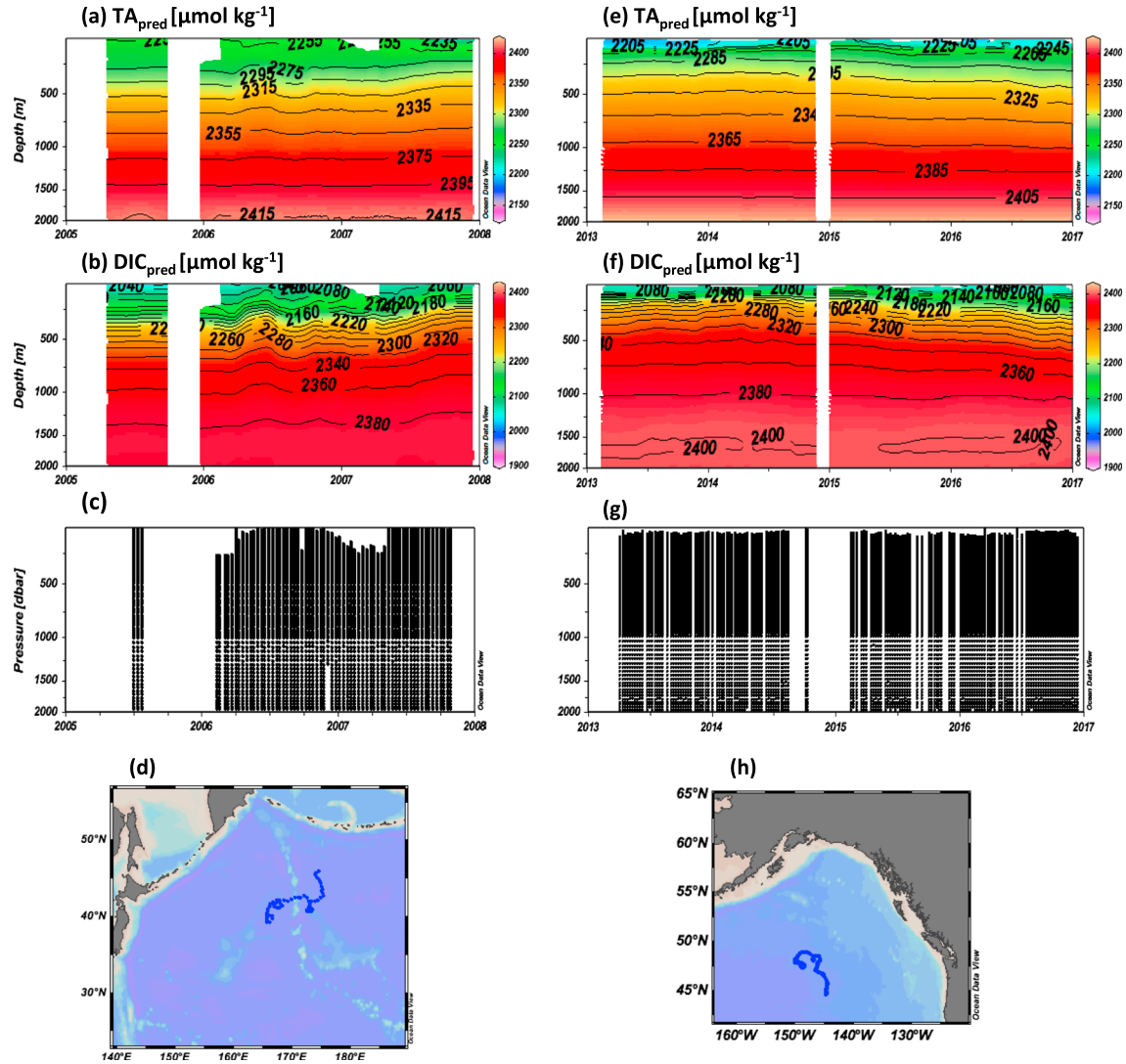
Figure 1. Vertical distributions of (a, e) TA_{pred} ( \mu\text{mol/kg} ) and (b, f) DIC_{pred} ( \mu\text{mol/kg} ) above 2,000-m depth predicted by applying new parameterizations to DO, T , and S data from Argo profiling floats 2900540 and 5904106, with (c, g) sampling profiles and (d, h) trajectory maps, respectively, drawn using Ocean Data View ( http://odv.awi.de ). DIC = dissolved inorganic carbon; TA = total alkalinity.
