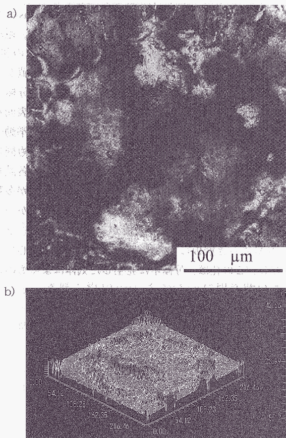
Fig. 6. CSLM images contrast, (a) and 3D, (b) of Zn-5mass%Al coated steel after laser irradiation at E_a = -650 \text{ mV} .
