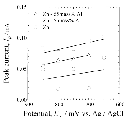
Fig. 8. Change in peak current with E_a after laser irradiation.
