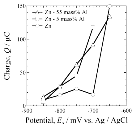
Fig. 7. Change in charge, Q with E_a .
