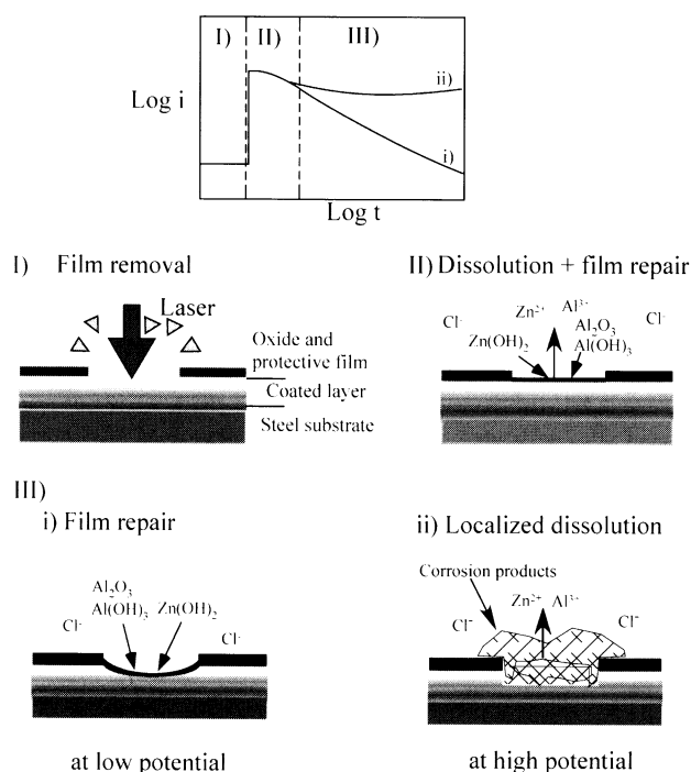
Fig. 11. Schematic model of film reformation or localized dissolution after oxide film was removed.
