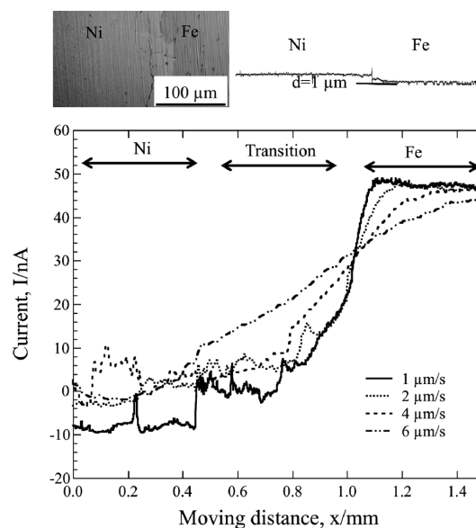
Fig. 7. Current profiles of a line scan from a nickel covered area to the iron substrate at different scanning rates, and surface image and height profile obtained by CSLM. The applied potential was -300 mV, and the solution was 0.5 \text{ kmol m}^{-3} \text{ H}_3\text{BO}_3/0.05 \text{ kmol m}^{-3} \text{ Na}_2\text{B}_4\text{O}_7 with 0.1 \text{ kmol m}^{-3} \text{ NaCl} . The deposited nickel thickness was 1 \mu\text{m} .
