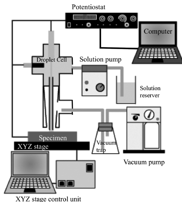
Fig. 4. Schematic view of the electrochemical measurement system used here.
