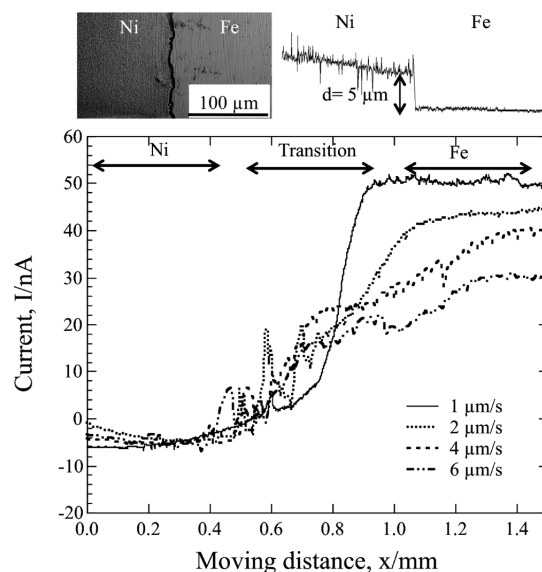
Fig. 8. Current profiles of a line scan across nickel deposited on iron and the iron substrate at different scanning rates, with surface image and height profile obtained by CSLM. The applied potential was -300 mV, and the solution was 0.5 \text{ kmol m}^{-3} \text{ H}_3\text{BO}_3/0.05 \text{ kmol m}^{-3} \text{ Na}_2\text{B}_4\text{O}_7 with 0.1 \text{ kmol m}^{-3} \text{ NaCl} . The deposited nickel thickness was 5 \mu\text{m} .
