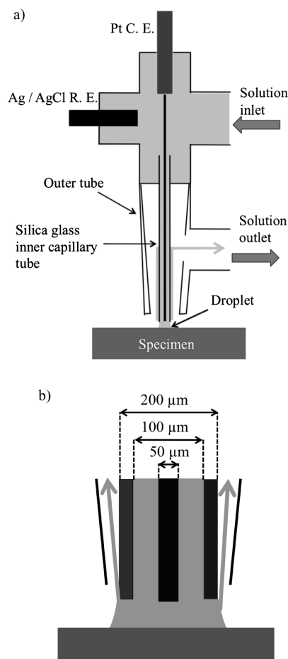
Fig. 1. Schematic outline of a) a cross section of the newly developed three electrode type droplet cell and b) an enlarged sketch of the tip of the cell.
