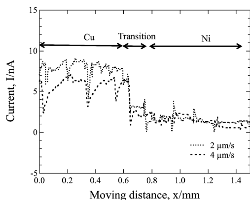
Fig. 6. Current profiles on a line scan from the surface of a copper substrate to a section with nickel deposited on the copper. Applied potential -120 mV, and in 0.5 \text{ kmol m}^{-3} \text{ H}_3\text{BO}_3/0.05 \text{ kmol m}^{-3} \text{ Na}_2\text{B}_4\text{O}_7 with 0.1 \text{ kmol m}^{-3} \text{ NaCl} .
