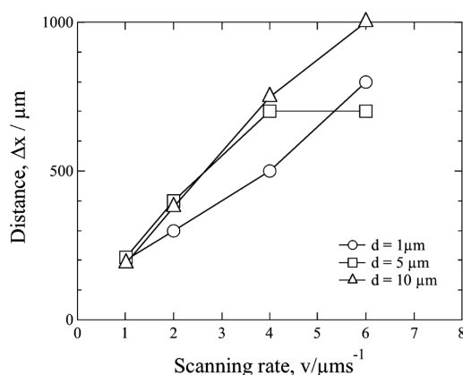
Fig. 10. The length of the transition (distance) between the two surface conditions, deposited nickel and iron substrate, for the droplet-cell in Figs. 7, 8, and 9 as a function of droplet cell scanning rate.
