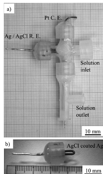
Fig. 3. Photograph of the developed droplet cell and the AgCl coated Ag reference electrode.
