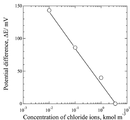
Fig. 2. Potential differences between the AgCl coated Ag wire and the Ag/AgCl sat. KCl reference electrode as a function of chloride ion concentration.
