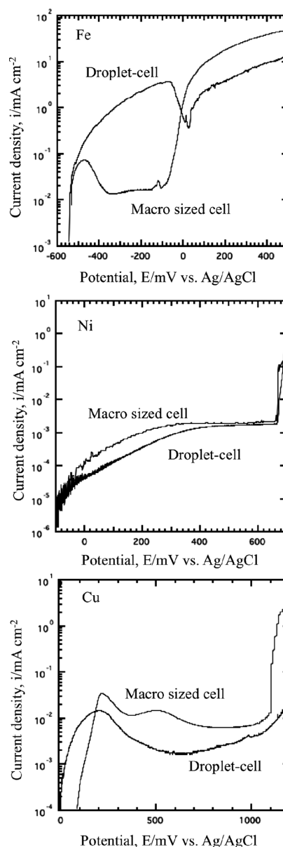
Fig. 5. Potentio-dynamic polarization curves iron, copper and nickel in 0.5 \text{ kmol m}^{-3} \text{ H}_3\text{BO}_3/0.05 \text{ kmol m}^{-3} \text{ Na}_2\text{B}_4\text{O}_7 with 0.01 \text{ kmol m}^{-3} \text{ NaCl} by the droplet cell and macro cell.
