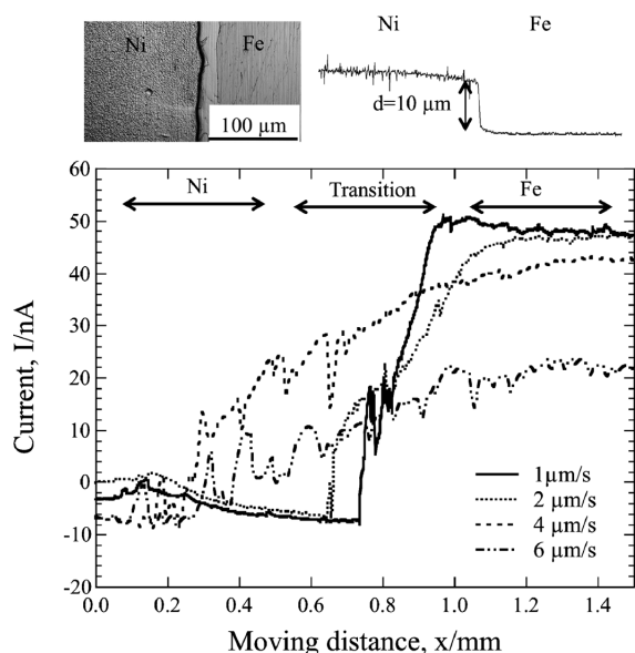
Fig. 9. Current profiles of a line scan across nickel deposited on iron and the iron substrate at different scanning rates, with a surface image and height profile obtained by CSLM. The applied potential was -300 mV, and the solution was 0.5 \text{ kmol m}^{-3} \text{ H}_3\text{BO}_3/0.05 \text{ kmol m}^{-3} \text{ Na}_2\text{B}_4\text{O}_7 with 0.1 \text{ kmol m}^{-3} \text{ NaCl} . The deposited nickel thickness was 10 \text{ μm} .
