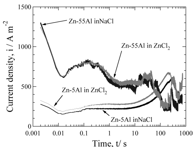
Fig. 10. Changes in current density of Zn-5Al or Zn-55Al alloy coated steels after laser irradiation up to 800 s at -600 mV in 0.5 \text{ kmol m}^{-3} \text{ H}_3\text{BO}_3 - 0.05 \text{ kmol m}^{-3} \text{ Na}_2\text{B}_4\text{O}_7 with 10 \text{ mol m}^{-3} \text{ NaCl} or with 5 \text{ mol m}^{-3} \text{ ZnCl}_2 .
