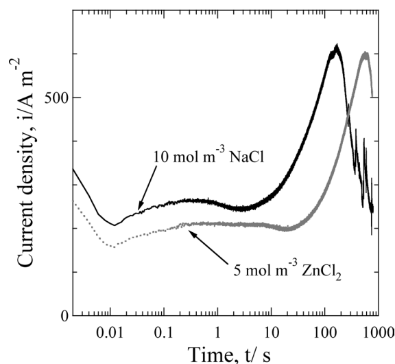
Fig. 7. Changes in current of Zn coated steels after laser irradiation up to 800 s at -400 mV in 0.5 \text{ kmol m}^{-3} \text{ H}_3\text{BO}_3 – 0.05 \text{ kmol m}^{-3} \text{ Na}_2\text{B}_4\text{O}_7 with 10 \text{ mol m}^{-3} \text{ NaCl} or with 5 \text{ mol m}^{-3} \text{ ZnCl}_2 .
