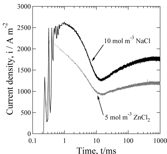
Fig. 6. Changes in current of Zn coated steels after laser irradiation up to 1 s at -400 mV in 0.5 \text{ kmol m}^{-3} \text{ H}_3\text{BO}_3 – 0.05 \text{ kmol m}^{-3} \text{ Na}_2\text{B}_4\text{O}_7 with 10 \text{ mol m}^{-3} \text{ NaCl} or with 5 \text{ mol m}^{-3} \text{ ZnCl}_2 .
