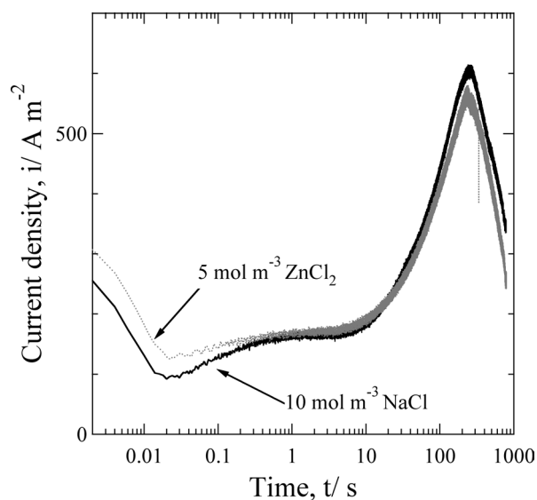
Fig. 4. Changes in currents of Zn coated steels after laser irradiation up to 800 s at -600 mV in 0.5 \text{ kmol m}^{-3} \text{ H}_3\text{BO}_3 – 0.05 \text{ kmol m}^{-3} \text{ Na}_2\text{B}_4\text{O}_7 with 10 \text{ mol m}^{-3} \text{ NaCl} or with 5 \text{ mol m}^{-3} \text{ ZnCl}_2 .
