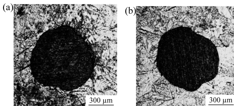
Fig. 8. CSLM contrast images after the experiments of Fig. 7, (a) in NaCl and (b) in \text{ZnCl}_2 . The corrosion products and nitrocellulose film were removed before the CSLM observation.
