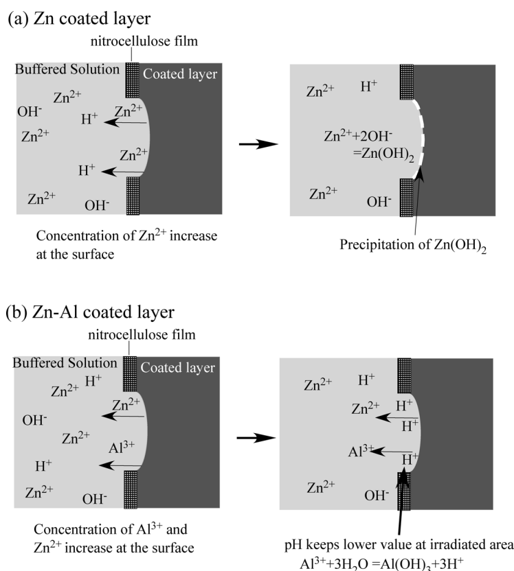
Fig. 11. Schematic representation of the effect of Zn ions on corrosion of the coated layer, (a) Zn coated layer and (b) Zn-Al alloy coated layer.
