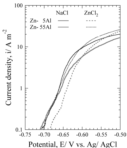
Fig. 2. Polarization curves of Zn–5Al and Zn–55Al coated steels in 0.5 \text{ kmol m}^{-3} \text{ H}_3\text{BO}_3 – 0.05 \text{ kmol m}^{-3} \text{ Na}_2\text{B}_4\text{O}_7 with 10 \text{ mol m}^{-3} \text{ NaCl} or with 5 \text{ mol m}^{-3} \text{ ZnCl}_2 .
