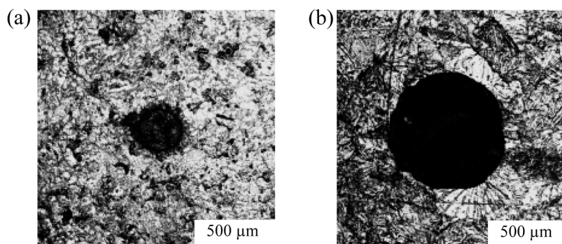
Fig. 5. CSLM contrast images of after the laser experiments in 0.5 \text{ kmol m}^{-3} \text{ H}_3\text{BO}_3 – 0.05 \text{ kmol m}^{-3} \text{ Na}_2\text{B}_4\text{O}_7 with 10 \text{ mol m}^{-3} \text{ NaCl} , after laser irradiation, (a) up to 1 s, and (b) up to 800 s. The corrosion products and nitrocellulose film were removed before the CSLM observation.
