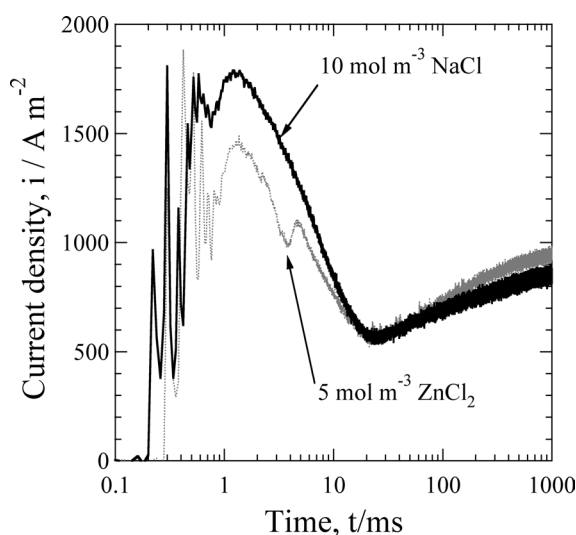
Fig. 3. Changes in current of Zn coated steels after laser irradiation up to 1 s at -600 mV in 0.5 \text{ kmol m}^{-3} \text{ H}_3\text{BO}_3 – 0.05 \text{ kmol m}^{-3} \text{ Na}_2\text{B}_4\text{O}_7 with 10 \text{ mol m}^{-3} \text{ NaCl} or with 5 \text{ mol m}^{-3} \text{ ZnCl}_2 .
