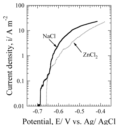
Fig. 1. Polarization curves of Zn coated steels in 0.5 \text{ kmol m}^{-3} \text{ H}_3\text{BO}_3 – 0.05 \text{ kmol m}^{-3} \text{ Na}_2\text{B}_4\text{O}_7 with 10 \text{ mol m}^{-3} \text{ NaCl} or with 5 \text{ mol m}^{-3} \text{ ZnCl}_2 .
