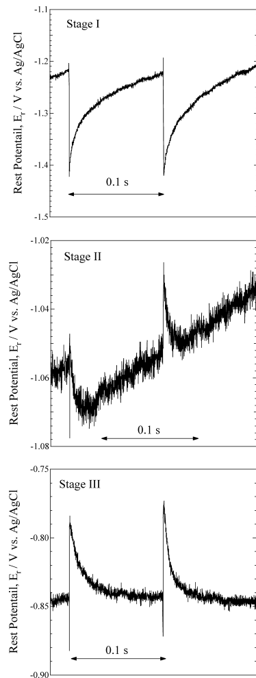
Fig. 6. Typical example of changes in the rest potential with time after laser irradiation at stage I, stage II and stage III in Fig. 5.
