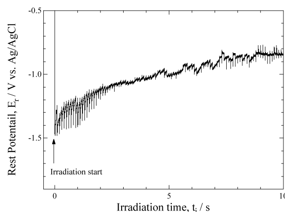
Fig. 5. Changes in the rest potential with time during continuous laser irradiation in 0.5 \text{ kmol m}^{-3} \text{H}_3\text{BO}_3 – 0.05 \text{ kmol m}^{-3} \text{Na}_2\text{B}_4\text{O}_7 with 0.01 \text{ kmol m}^{-3} \text{NaCl} solutions.
