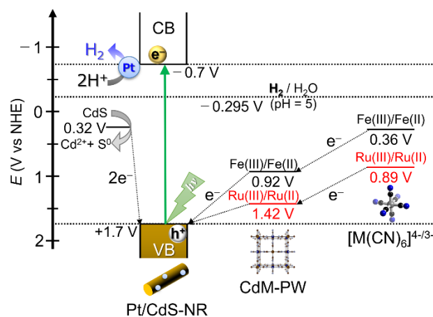
Scheme 1 Schematic energy diagram for the photocatalytic \text{H}_2 evolution reaction driven by Pt/CdS-NR in the presence of \text{K}_4[\text{M}(\text{CN})_6] ( \text{M} = \text{Fe}, \text{Ru} ) redox mediators.
