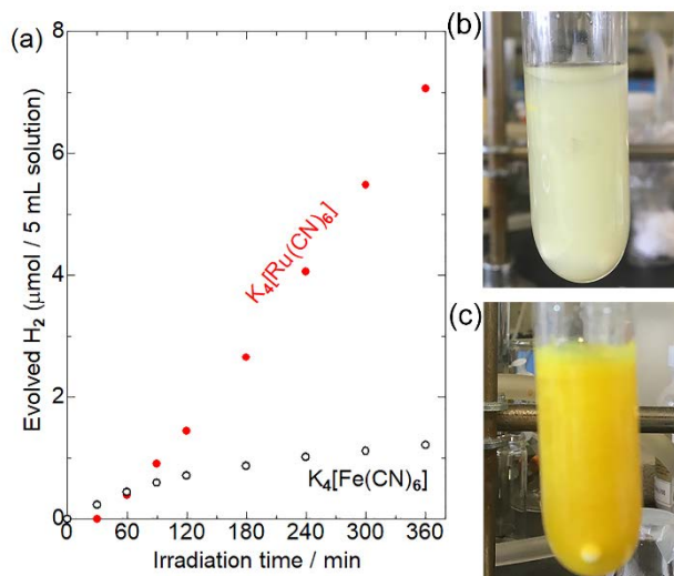
Fig. 3 (a) Photocatalytic hydrogen evolution reaction with Pt/CdS-NR (2.00 mg) in a 200 mM acetate buffer (pH=5.0) that contained 0.01 M \text{K}_4[\text{M}(\text{CN})_6] as the electron source (black open circles: \text{K}_4[\text{Fe}(\text{CN})_6] ; red closed circles: \text{K}_4[\text{Ru}(\text{CN})_6] ) under an Ar atmosphere. A blue LED ( \lambda = 470 \pm 10 nm) was used as the light source. Photographs of the reaction solutions of (b) \text{K}_4[\text{Ru}(\text{CN})_6] and (c) \text{K}_4[\text{Fe}(\text{CN})_6] after light irradiation for 6 h.
