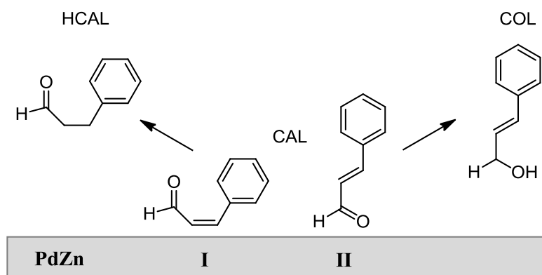
Scheme 3. Adsorption of CAL molecule in two different orientations I (side-on type) and II (end-on type) yielding HCAL and COL, respectively, on the surface of PdZn particles dispersed on ZnO
