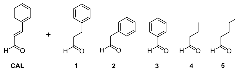
Scheme 2. Aldehydes 1 - 5 added to CAL hydrogenation (Table 2). 1 :
