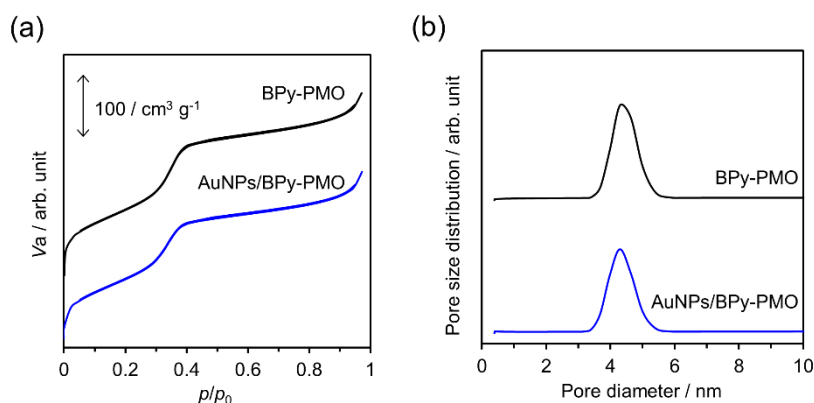
Fig. 2. (a) N 2 adsorption isotherms and (b) NLDT pore diameter distribution curves of BPy-PMO (black line) and AuNPs/BPy-PMO (blue line).
