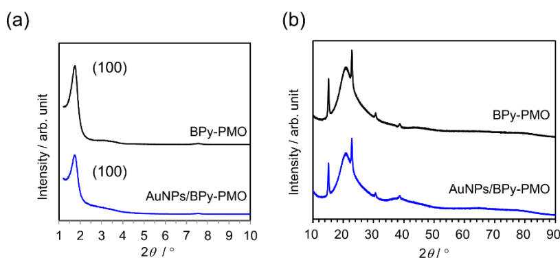
Fig. 3. XRD patterns of BPy-PMO (black line) and AuNPs/BPy-PMO (blue line) in (a) low and (b) high-angle region.
