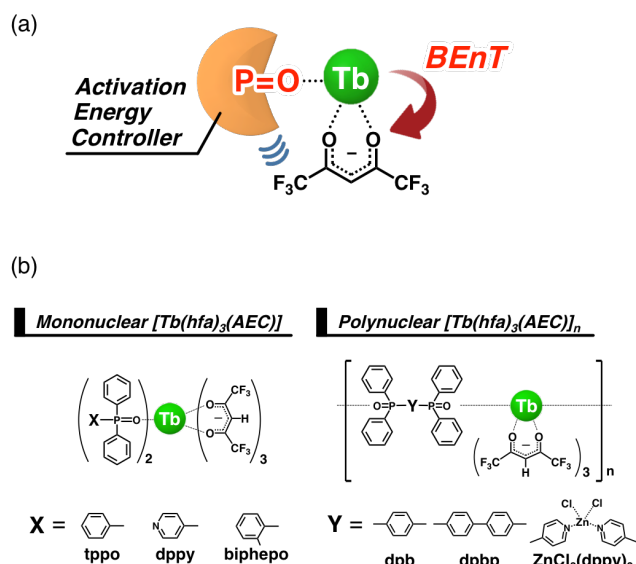
Figure 1. (a) Conceptual image of this study. (b) Chemical structure of Tb(hfa) 3 (phosphine oxide) complexes.
