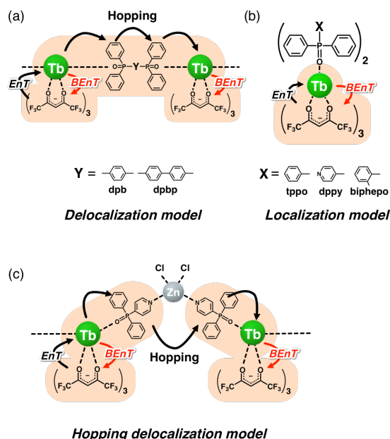
Figure 5. (a) Excited energy delocalization image of polynuclear [\text{Tb}(\text{hfa})_3(\text{dpb})]_n and [\text{Tb}(\text{hfa})_3(\text{dppb})]_n . (b) Excited energy localization image of mononuclear [\text{Tb}(\text{hfa})_3(\text{AEC})] . (c) Excited energy delocalization image of polynuclear [\text{Tb}(\text{hfa})_3\text{ZnCl}_2(\text{dppy})_2]_n .
