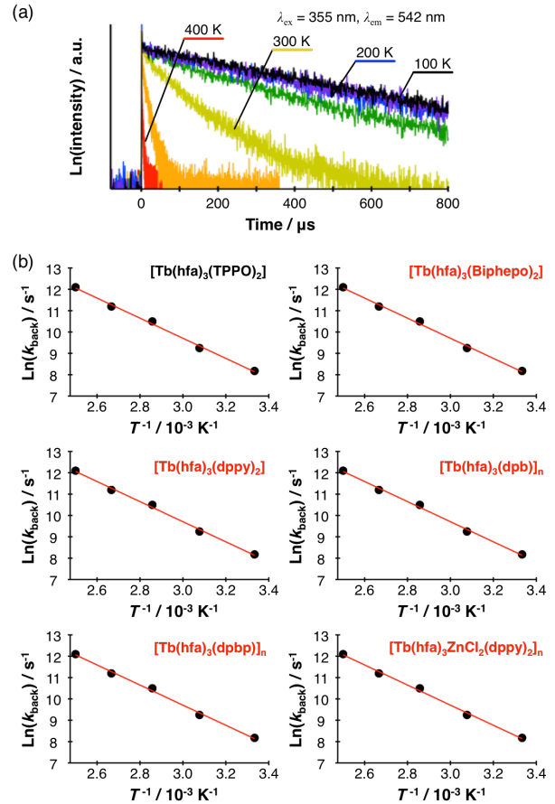
Figure 3. (a) Temperature-dependent emission lifetime decays of [\text{Tb}(\text{hfa})_3(\text{tpo})_2] in the solid state among 100–400 K. Excited at 355 nm (third harmonics of Q-switched Nd:YAG laser. fwhm = 5 ns, \lambda = 1064 nm, black line: 100 K, purple line: 150 K, blue line: 200 K, green line: 250 K, yellow line: 300 K, orange line: 350 K, red line 400 K). (b) Arrhenius plots of each each \text{Tb}(\text{hfa})_3 complex in the solid state.
