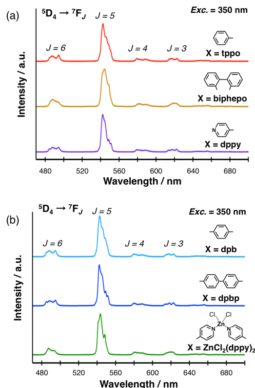
Figure 2. Emission spectra of (a) mononuclear [\text{Tb}(\text{hfa})_3(\text{AEC})] and (b) polynuclear [\text{Tb}(\text{hfa})_3(\text{AEC})]_n in the solid state at room temperature. Excited at 350 nm.
