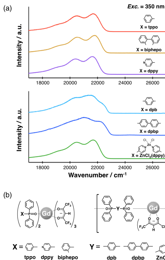
Figure 4. (a) Phosphorescence spectra of mononuclear [\text{Gd}(\text{hfa})_3(\text{AEC})] and polynuclear [\text{Gd}(\text{hfa})_3(\text{AEC})]_n in the solid state at 100 K. Excited at 350 nm (Time delay = 0 ms). (b) Chemical structure of \text{Gd}(\text{hfa})_3(\text{phosphine oxide}) complexes.
