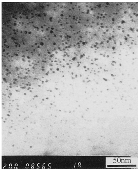
Fig. 11. Typical high-magnification transmission electron micrographs of oxide particles in M11 cladding.
