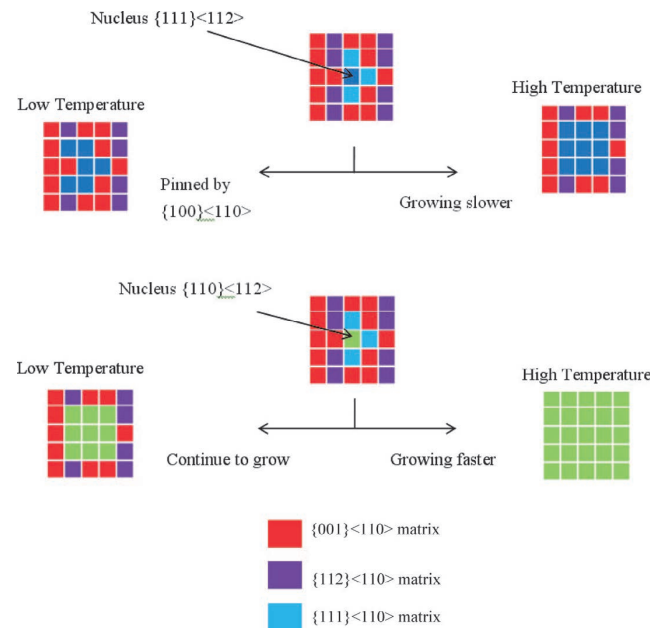
Fig. 7. Schematic view of nuclei growth at low and high temperature.
