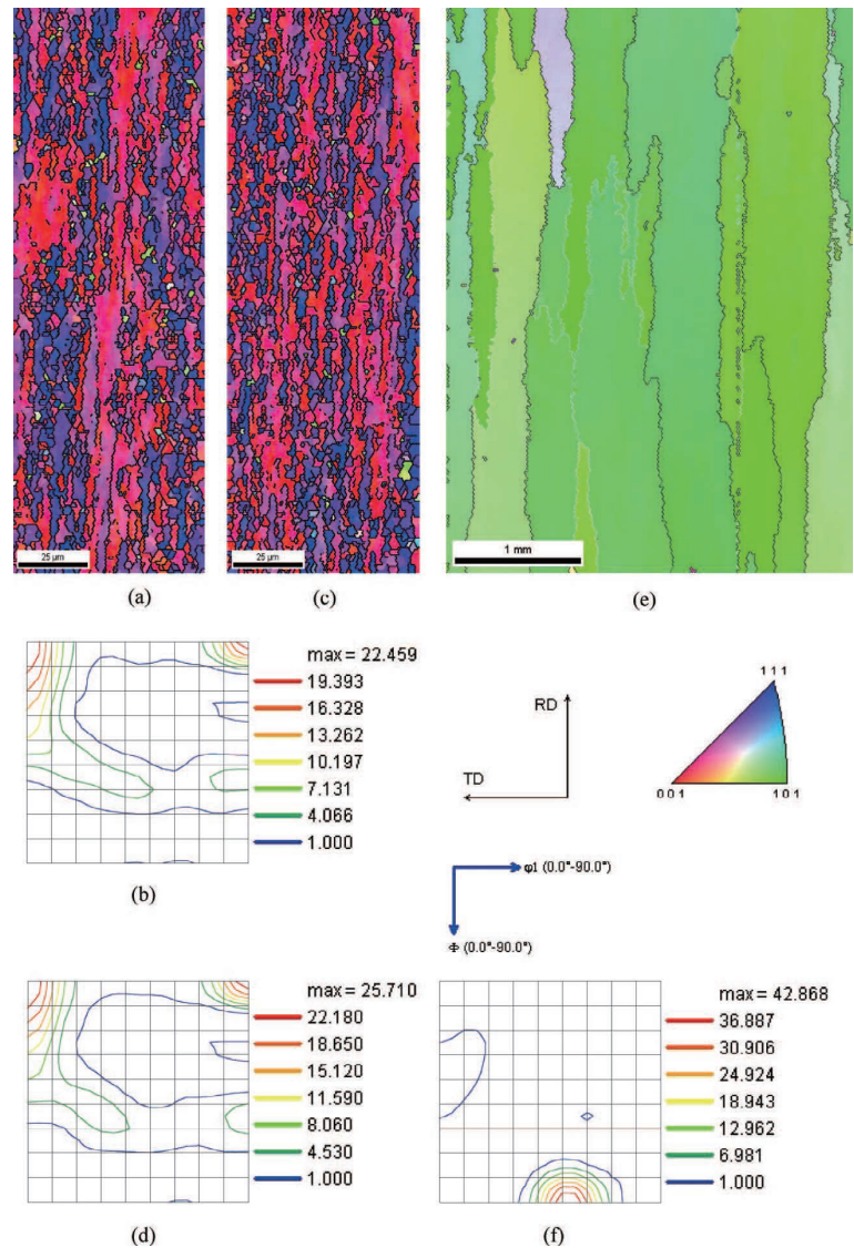
Fig. 5. Specimen underwent two step annealing, first recovery annealed at 900°C for 2 hrs: (a) IPF, (b) ODF then recrystallization annealed at 1 000°C for 24 hrs: (c) IPF, (d) \phi 2=45^\circ section of ODF and 1 300°C for 1 hr: (e) IPF, (f) \phi 2=45^\circ section of ODF.
