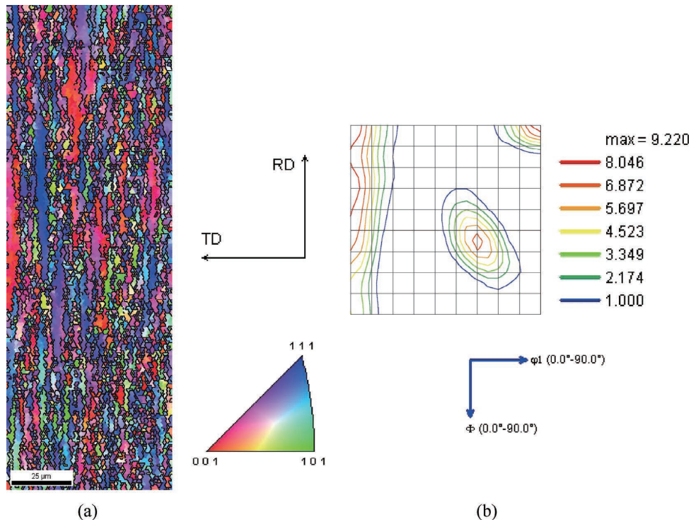
Fig. 1. Results of texture analyses before cold-rolling: (a) Inverse pole figure (IPF), (b) \varphi_2=45^\circ section of ODF (Orientation distribution function).
