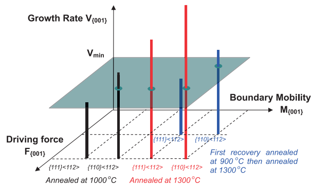
Fig. 6. Schematic of growth rate of two kinds of nuclei overcome \{001\}<110> under different heat-treatment conditions.
