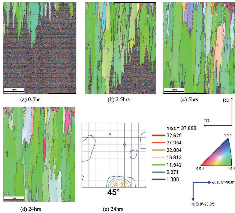
Fig. 3. Inverse pole figure of specimen annealed at 1 000°C for (a) 0.5 hr, (b) 2.5 hrs, (c) 5 hrs, (d) 24 hrs and (e) \phi_2 = 45^\circ section of ODF of specimen annealed at 1 000°C for 24 hrs.
