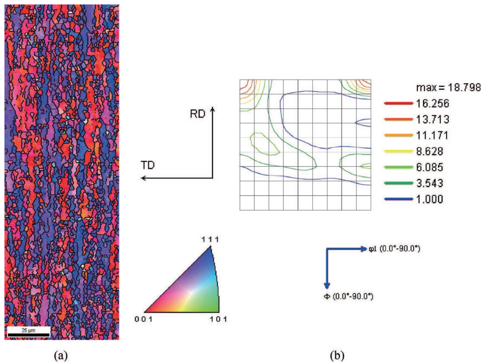
Fig. 2. Results of texture analyses after cold-rolling: (a) IPF of as-cold-rolled specimen, (b) \varphi_2=45^\circ section of ODF.
