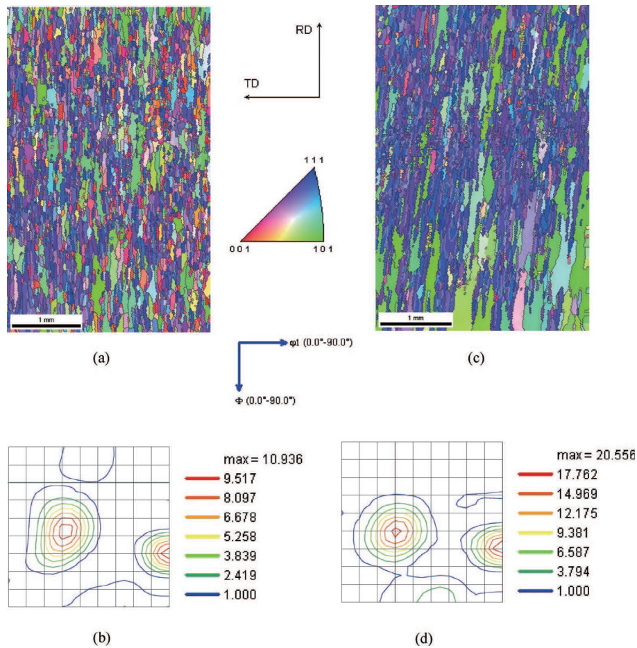
Fig. 4. Specimen annealed at 1 150°C for 5 mins: (a) IPF, (b) \phi_2 = 45^\circ section of ODF and annealed at 1 300°C for 5 mins: (c) IPF, (d) \phi_2 = 45^\circ section of ODF.
