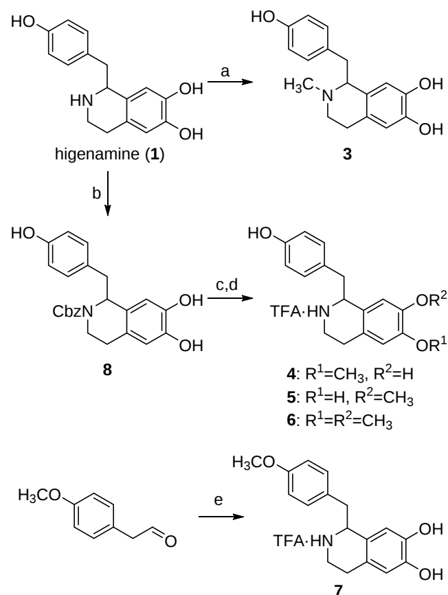
Scheme 1. Synthesis of compounds 3–7 . a) formaldehyde, \text{NaBH}_4 , MeOH; b) \text{CbzCl} , 1,4-dioxane, water, \text{NaHCO}_3 ; c) MeI, \text{K}_2\text{CO}_3 , DMF; d) 10% Pd-C, \text{H}_2 , EtOAc and then HPLC purification; e) dopamine hydrochloride, MeCN, 0.1 M phosphate buffer (pH6.0), 50°C and then HPLC purification. See materials and method section for HPLC condition.
