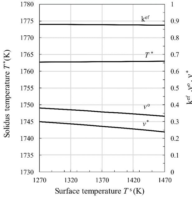
Fig. 8 Influence of the surface temperature T^s on the solidus temperature T^* , the effective partition ratio k^{ef} and the solidification constants v^* and v^0 . (0.15% C, k = 0.225 , and the others properties are listed in Table 1).
