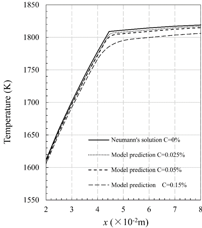
Fig. 4 Transitions of temperature predicted by the model and the Neumann' solution ( C=0\% ) of a continuously cast steel. ( C=0\%-0.15\% , T^s = 1423 \text{ K} (1150 °C), \Delta T = 15 \text{ K} (15 °C), t = 240 \text{ s} , slab thickness = 0.22 m).
