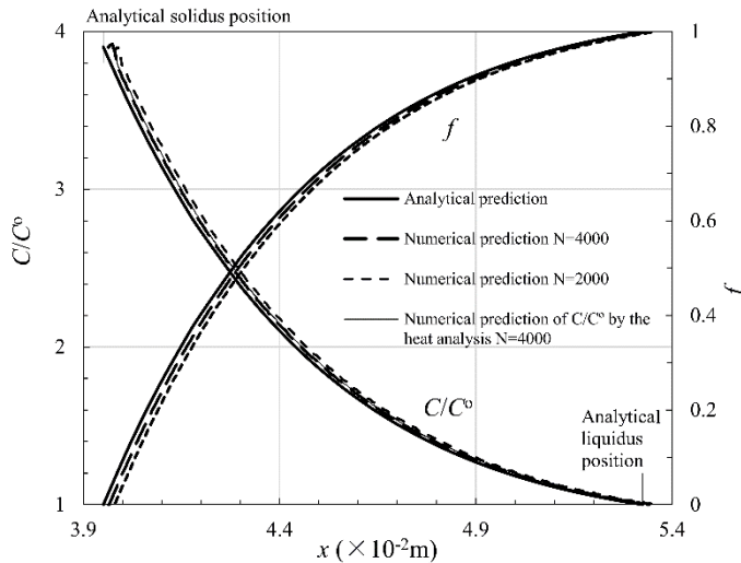
Fig. 3 Solute concentration C/C^0 and liquid fraction predicted by the model and numerical analysis of a continuously cast steel. (0.15% C, T^s = 1423 \text{ K} (1150 °C), \Delta T = 15 \text{ K} (15 °C), t = 240 \text{ s} , slab thickness = 0.22 m, N = partitioning number of the half thickness of a slab).
