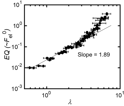
Figure 4. Dependence of EQ on \lambda (=Q^{1/3}) of the St-tetra-PEG gels with varying C_{stent} and C_{PEG} . The solid line represents the power-law relationship shown in Eq. (10a).
