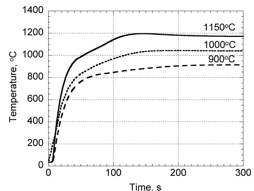
Fig. 2. Temperature profiles near the sample surface during heating.
