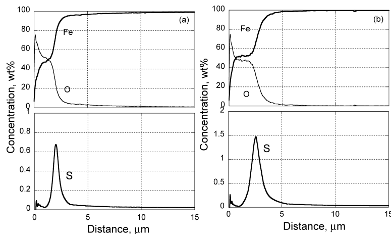
Fig. 9. GD-OES profiles of the surface after scale spallation of (a) 30S and (b) 100S steels at 1 150°C for 120 s.
