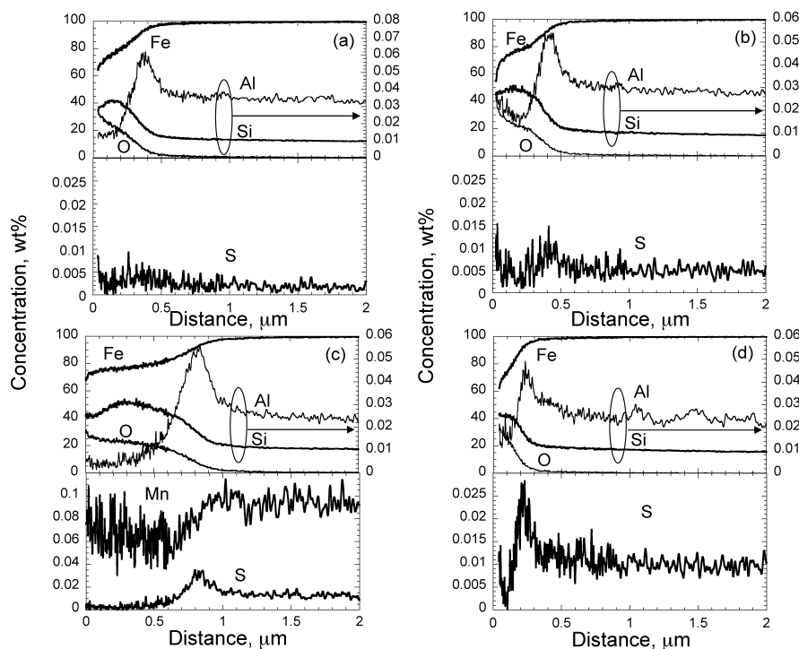
Fig. 7. GD-OES profiles of each element at 1150^\circ\text{C} for 30 s. (a) Base, (b) 30S, (c) 100SM, and (d) 100S.
