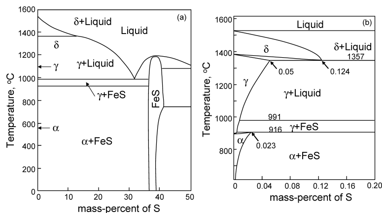
Fig. 10. Fe-S binary phase diagram. (b) is low sulfur region up to 0.2 mass% sulfur.
