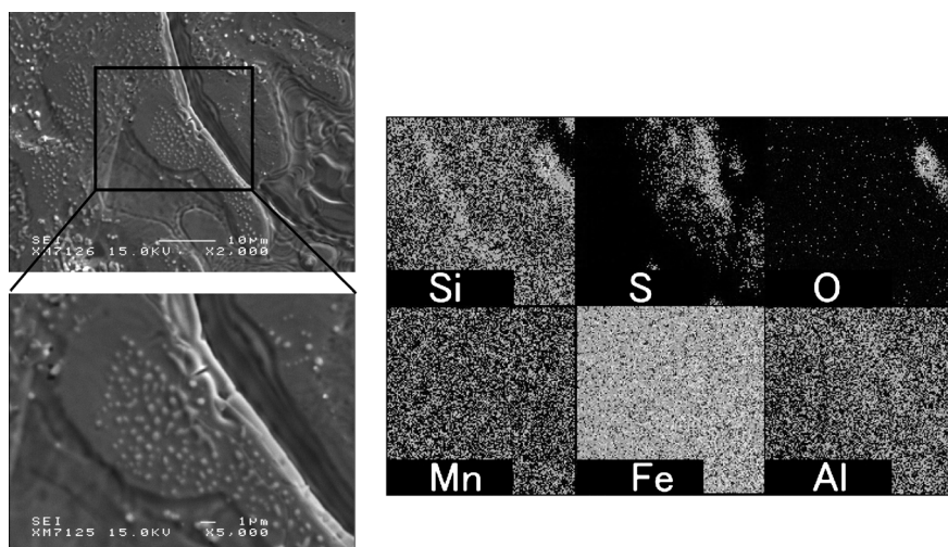
Fig. 11. Surface morphologies and elemental map of the steel surface of 100S after oxidation at 1150°C for 120 s followed by scale spallation in liquied nitrogen.
