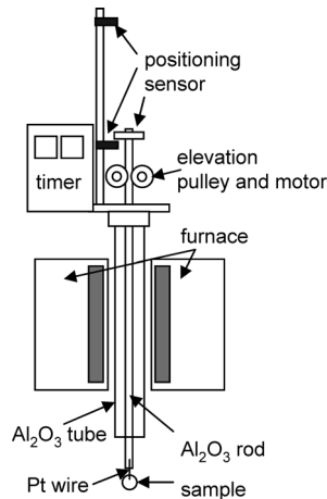
Fig. 1. Oxidation apparatus used in this study.
