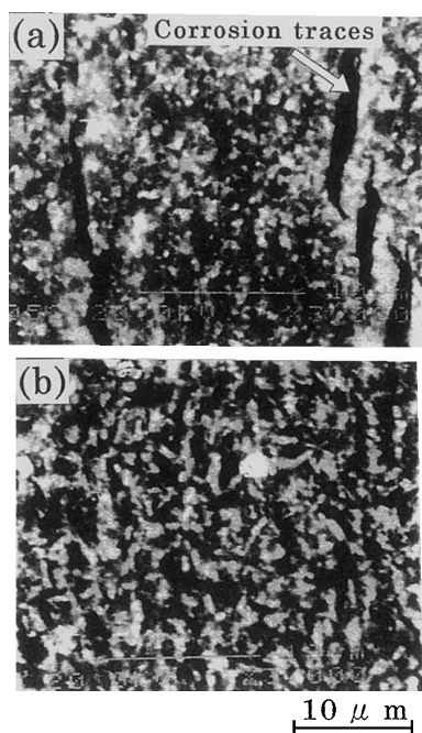
Fig. 11. Magnified SEM photographs of the cross-sections of the inner, alloy layer in (a) the Zn-6Al coat and (b) the Zn-6Al-0.5Mg-0.1Si coated film after corrosion in a 5% NaCl solution at room temperature for 1.8 ks.
