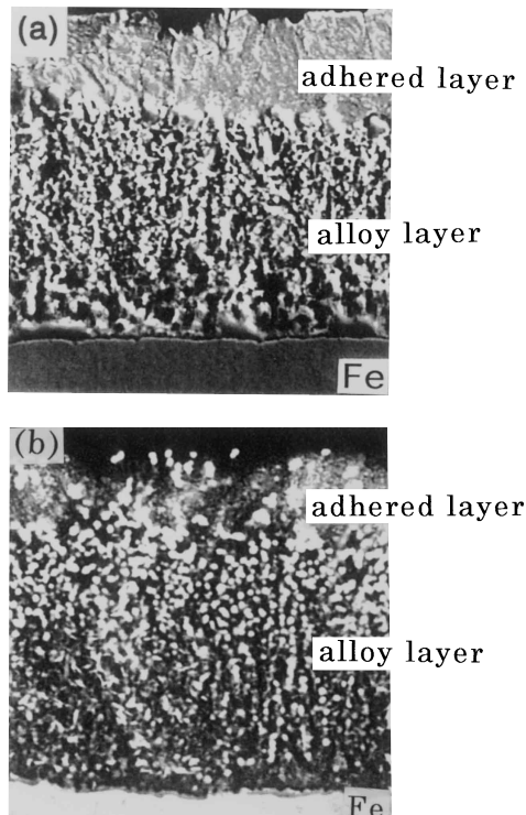
Fig. 4. Cross sectional microstructures of (a) the Zn-6Al coated and (b) the Zn-6Al-0.5Mg-0.1Si coated films.
