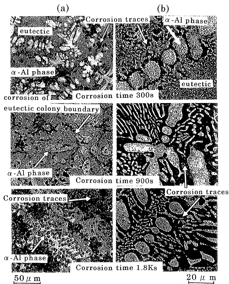
Fig. 9. Microstructures of the surface internal, adhered layer in (a) the Zn-6Al coated and (b) the Zn-6Al-0.5Mg-0.1Si coated films for different corrosion times in a 5% NaCl solution at room temperature.
