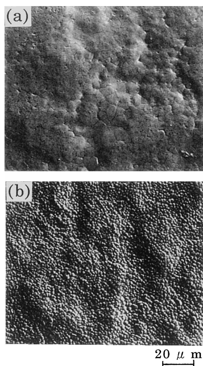
Fig. 1. Surface morphologies of the coatings formed on a low carbon steel by the two-step hot dipping. The secondary baths are (a) Zn–6Al alloy and (b) Zn–6Al–0.5Mg–0.1Si alloy.
