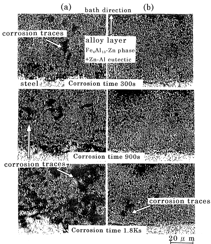
Fig. 10. Microstructures of cross-sections of the inner, alloy layer in (a) the Zn-6Al coated and the (b) Zn-6Al-0.5Mg-0.1Si coated films for different corrosion times in a 5%NaCl solution at room temperature.
