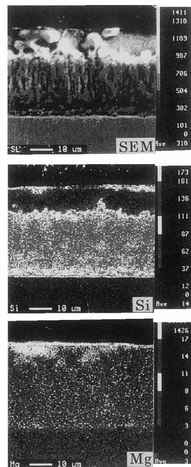
Fig. 6. X-ray images of Si and Mg in the cross-sections of the outer, adhered and alloy layers of the Zn-6Al-0.5Mg-0.1Si dipped film.
