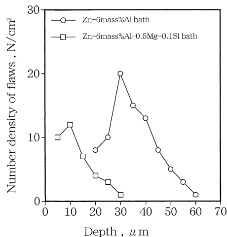
Fig. 3. Changes in number density of flaws as a function of depth of the flaws in the Zn–6Al and Zn–6Al–0.5Mg–0.1Si coated surfaces.
