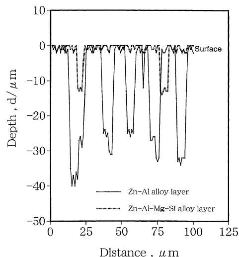
Fig. 2. Surface contour profiles measured using a laser scanning microscope for the Zn–6Al coating (a) and the Zn–6Al–0.5Mg–0.1Si coating (b) in Fig. 1 .
