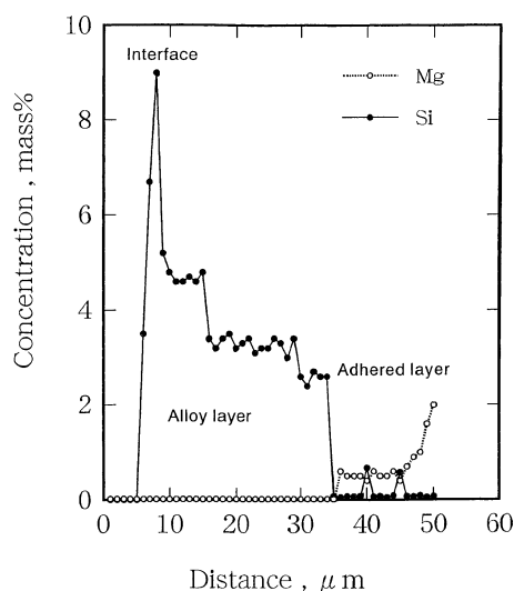
Fig. 12. Concentration profiles of Mg and Si in the Zn-6Al-0.5Mg-0.1Si coated film.
