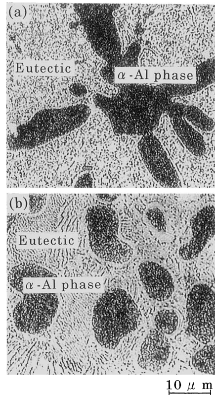
Fig. 5. Microstructures of the outer, adhered layer of (a) the Zn-6Al coated and (b) the Zn-6Al-0.5Mg-0.1Si coated films.
