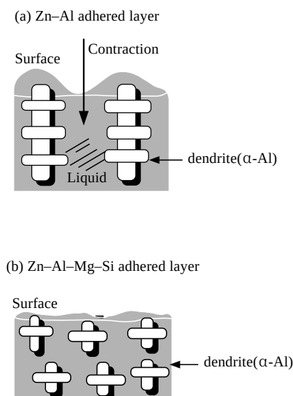
Fig. 7. Schematic representation of the solidification process in the outer layer in (a) the Zn-6Al coated and (b) the Zn-6Al-0.5Mg-0.1Si coated films.
