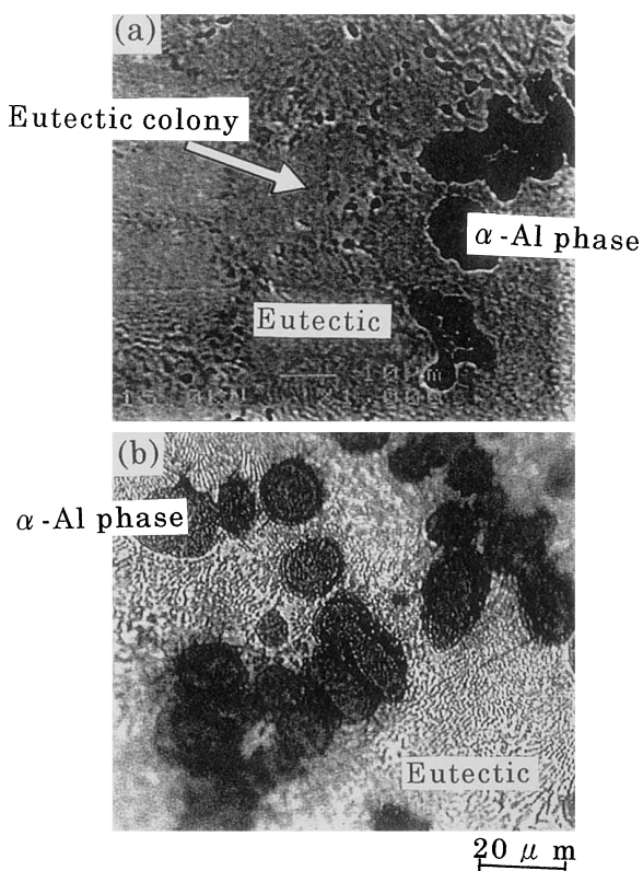
Fig. 8. Microstructures of the surface internal, adhered layer in (a) the Zn-6Al coated and (b) Zn-6Al-0.5Mg-0.1Si coated Films after corrosion in a 5% NaCl solution for 60 s at room temperature.
