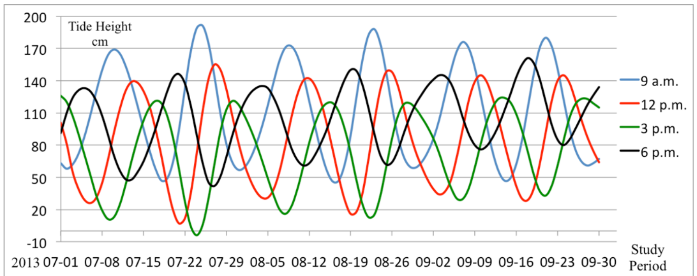
Figure 3.2 Time series of tidal condition at Sarahama Harbor of Irabu Island from 1 st July to 30 st September, 2013.
