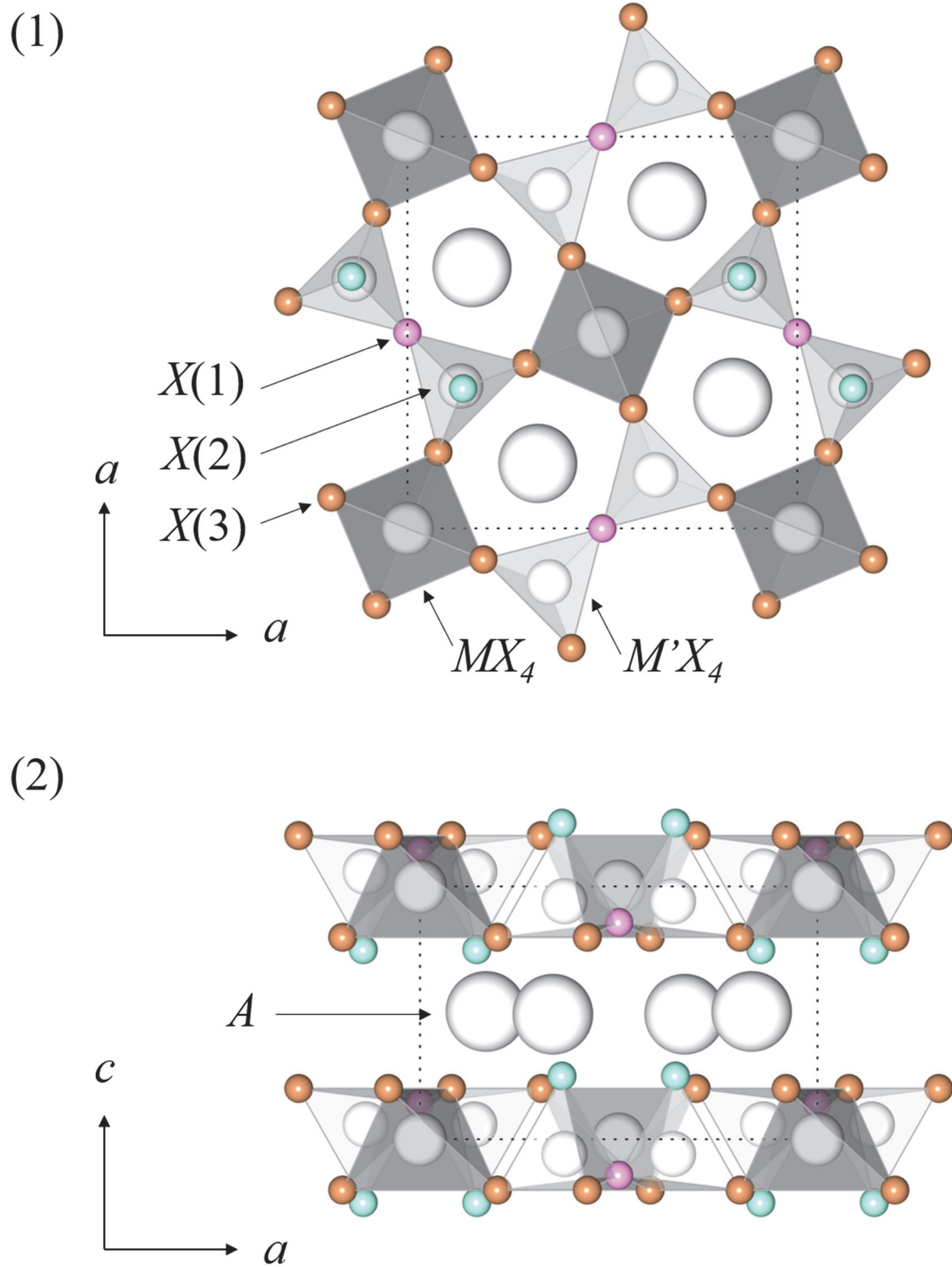
Figure 1.1. Schematic crystal structures of melilite-type compounds A_2MM'X_7 : (1) viewed from the c axis, (2) projection of the structure in ac plane.
