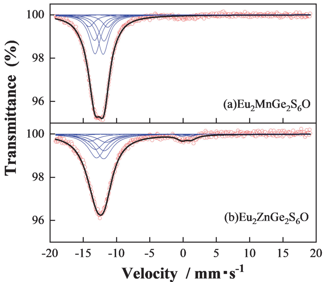
Figure 6.4 Mössbauer spectra for (a) \text{Eu}_2\text{MnGe}_2\text{S}_6\text{O} and (b) \text{Eu}_2\text{ZnGe}_2\text{S}_6\text{O} . The observed spectra are shown on the red circles.
