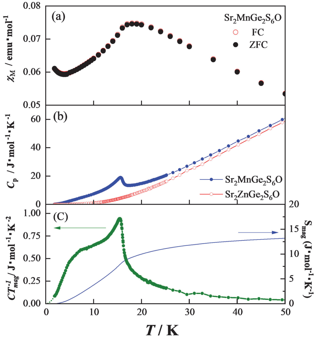
Figure 5.7 Temperature dependence of (a) magnetic susceptibility, (b) specific heat ( C_p ), (c) magnetic specific heat divided by temperature ( C_{mag}/T ), and magnetic entropy of \text{Sr}_2\text{MnGe}_2\text{S}_6\text{O} .
