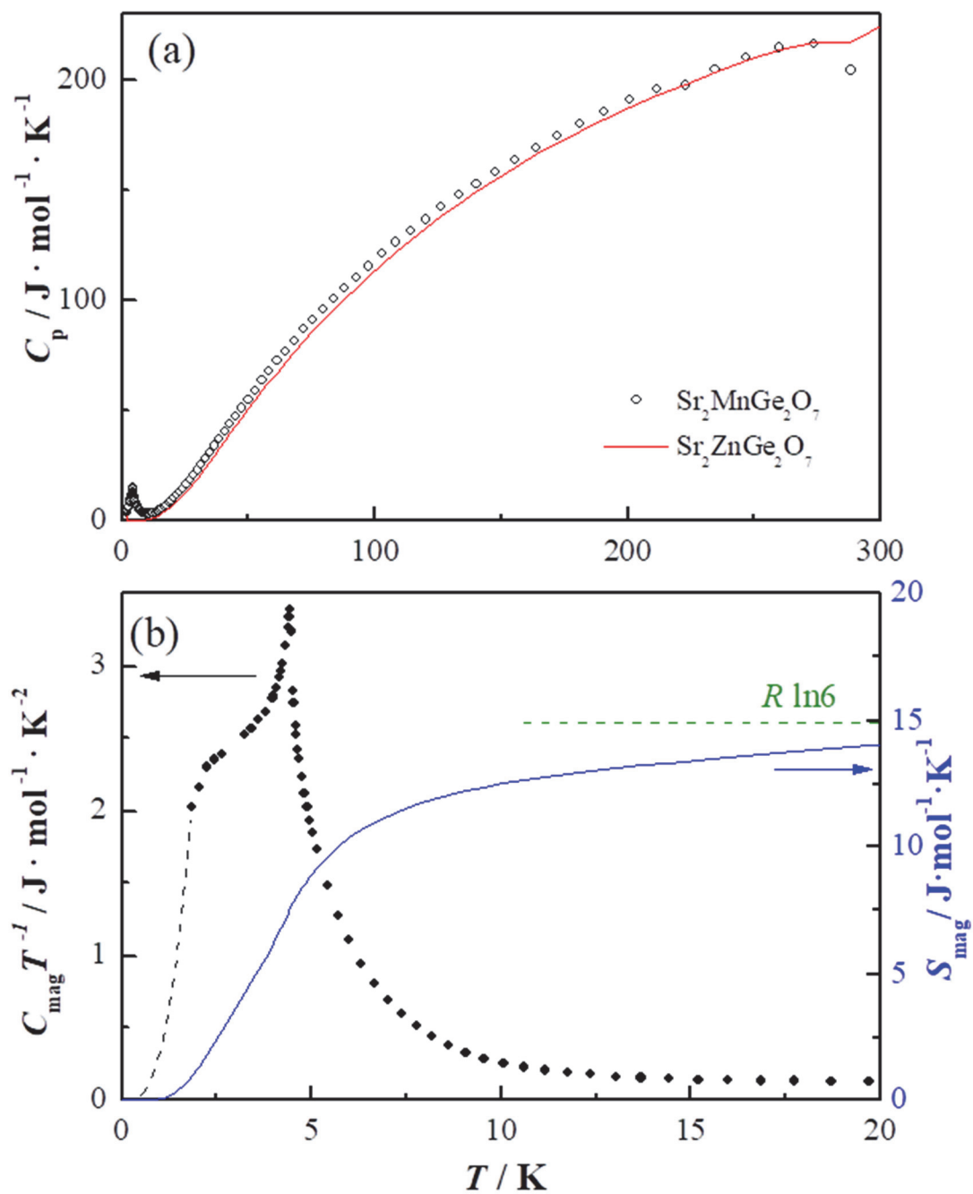
Figure 3.7 Temperature dependence of (a) specific heat ( C_p ), and (b) magnetic specific heat divided by temperature ( C_{\text{mag}} T^{-1} ) and magnetic entropy ( S_{\text{mag}} ) for \text{Sr}_2\text{MnGe}_2\text{O}_7 .
