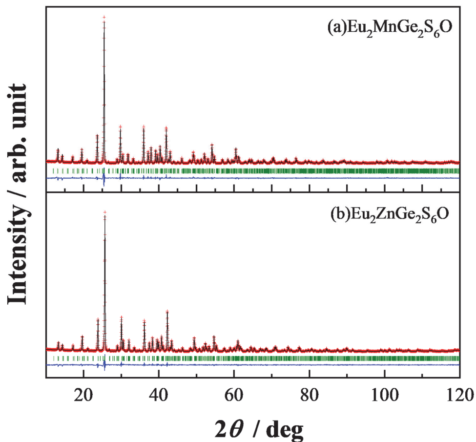
Figure 6.2 Powder XRD profiles for (a) \text{Eu}_2\text{MnGe}_2\text{S}_6\text{O} and (b) \text{Eu}_2\text{ZnGe}_2\text{S}_6\text{O} . The calculated and observed profiles are shown as the top black solid line and red markers, respectively. The vertical marks in the middle show positions calculated for Bragg reflection. The lower trace is a plot of the difference between calculated and observed intensities.
