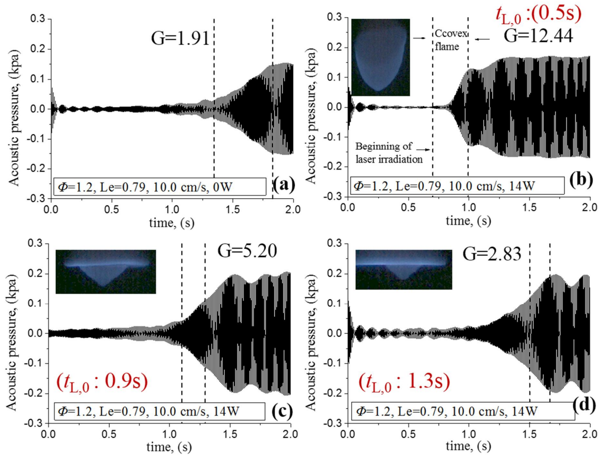
Fig. 3.8 Controlled flame shapes and acoustic pressure with various beginning timing of laser irradiation at the bottom of the tube as function of time for Le < 1 (a) 0 W (b) 14 W, 0.5 s, (c) 14 W, 0.9 s, (d) 14 W, 1.3 s.
