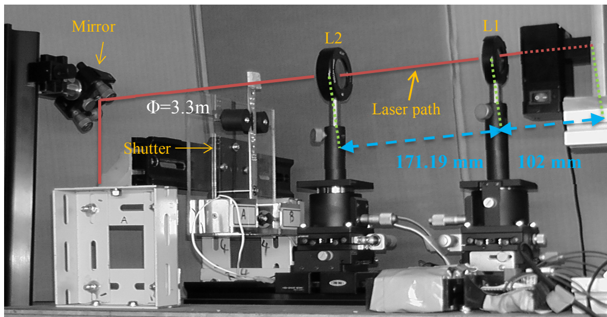
Fig. 2.3 Direct photo of optical setup.
