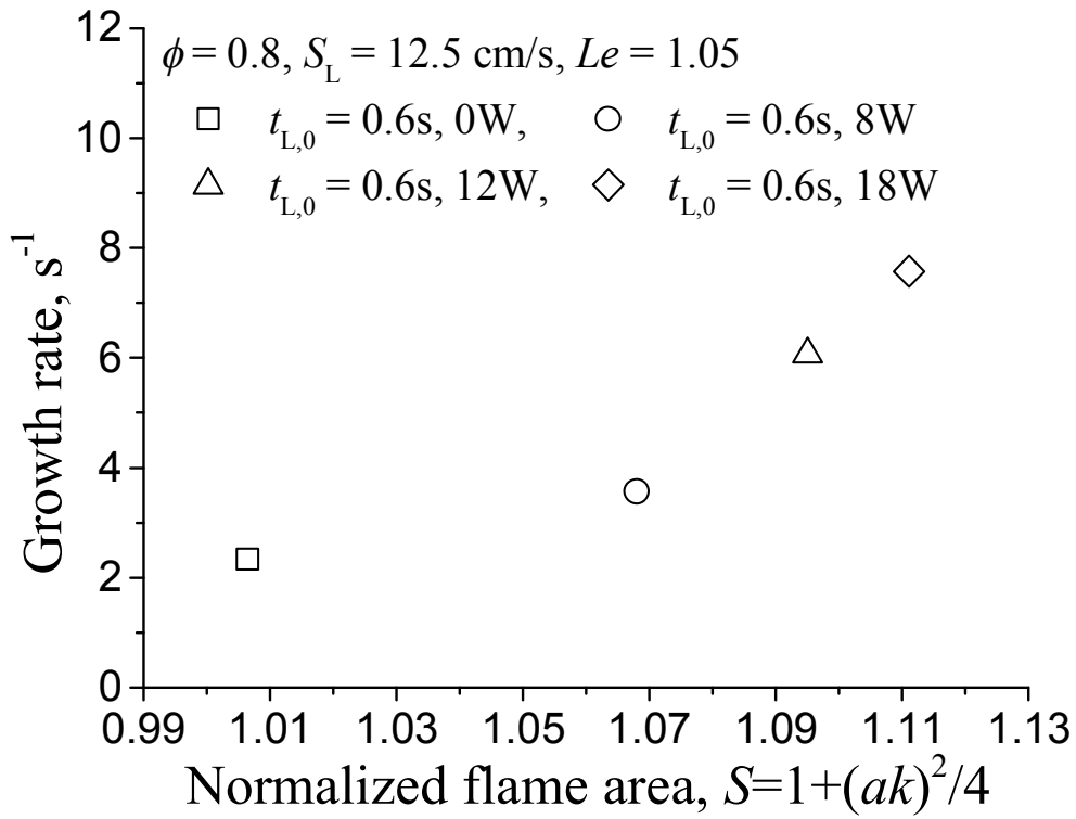
Fig. 3.13 Variation of growth rate of primary acoustic instability with concave flame surface change for Le > 1 .
