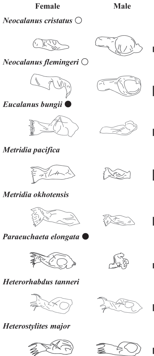
Fig. 5. Diagrams on gnathopod base of mandible of adult females and males of Neocalanus cristatus , N. flemingeri , Eucalanus bungii , Metridia pacifica , M. okhotsensis , Paraeuchaeta elongata , Heterorhabdus tanneri , and Heterostylites major in the southern Okhotsk Sea during 11 June 2011. ○: degeneration of teeth was seen for both females and males, ●: degeneration of teeth was seen only for males. Scale bars = 100 \mu m.
