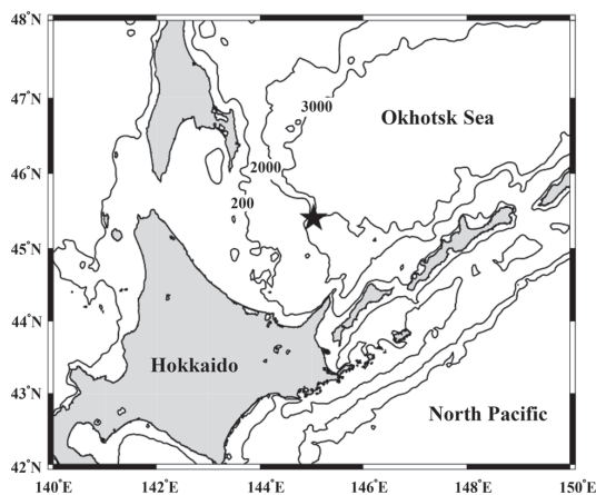
Fig. 1. Location of sampling station (star) in the southern Okhotsk Sea. Depth contours (200, 2,000 and 3,000 m) are superimposed.
