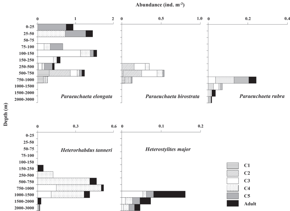
Fig. 4. Vertical distribution of carnivorous large-sized calanoid copepods : Paraeuchaeta elongata , P. birostrata , P. rubra , Heterorhabdus tanneri , and Heterostylites major in the southern Okhotsk Sea during 11 June 2011.
