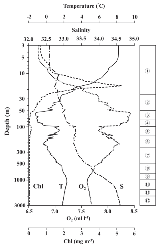
Fig. 2. Vertical profiles of temperature (T, °C), salinity (S), dissolved oxygen ( \text{O}_2 , \text{ml l}^{-1} ) and chlorophyll a (Chl, \text{mg m}^{-3} ) plotted on a log depth scale at sampling station in the southern Okhotsk Sea during 11 June 2011. Circled numbers in the right column indicate depth strata of the zooplankton samplings.
