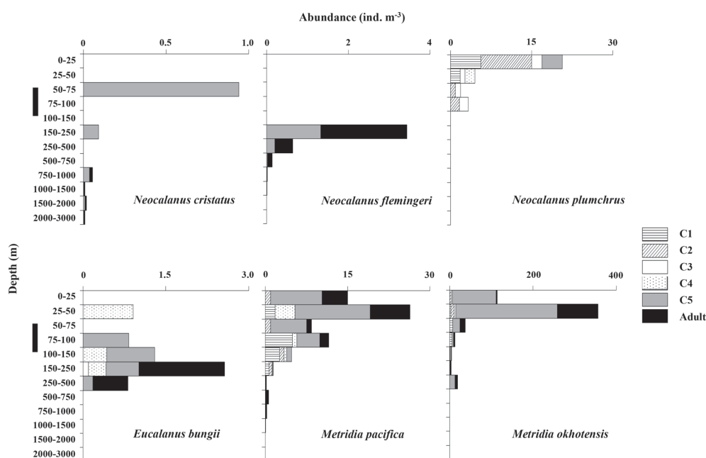
Fig. 3. Vertical distribution of suspension feeding large-sized calanoid copepods: Neocalanus cristatus , N. flemingeri , N. plumchris , Eucalanus bungii , Metridia pacifica , and M. okhotensis in the southern Okhotsk Sea during 11 June 2011. Black bars at left column indicate depth ranges of intermediate cold water were observed.
