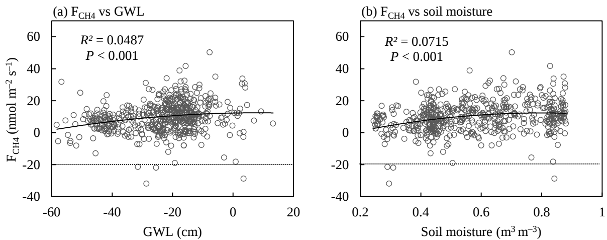
Figure 4.6 Responses of net ecosystem CH_4 exchange ( F_{CH_4} ) to (a) groundwater level (GWL) and (b) soil moisture on a daily basis. The relationships were determined using measured data and regression curves were drawn.
