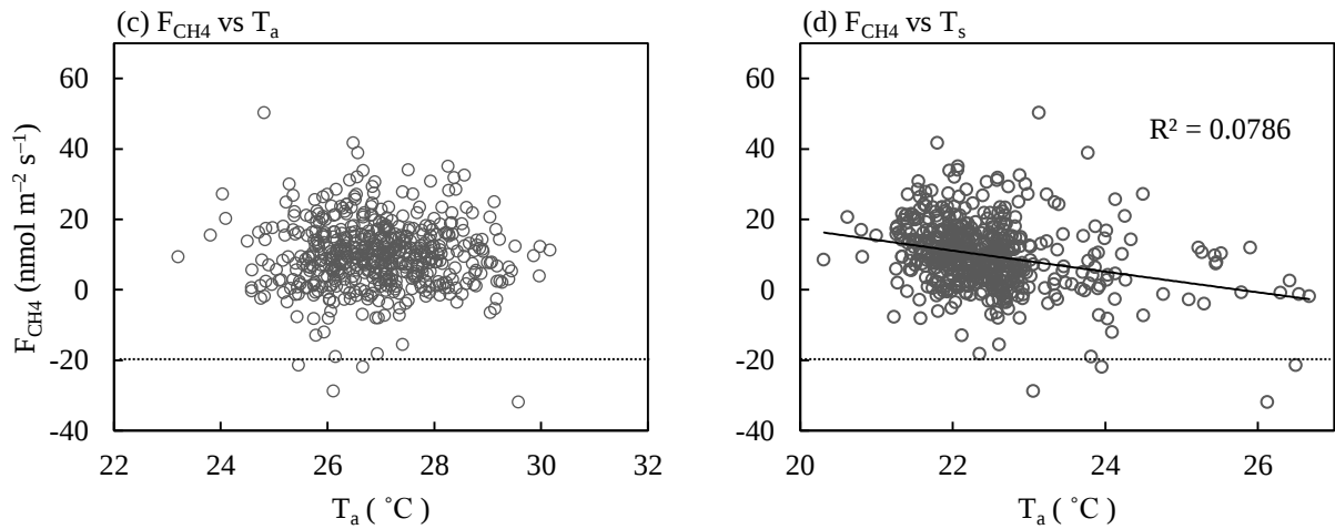
Figure 4.6 (continued) Responses of net ecosystem CH 4 exchange ( F_{CH_4} ) to (c) air temperature ( T_a ) and (d) soil temperature ( T_s ) on a daily basis. The relationships were determined using measured data and regression curves were drawn.
