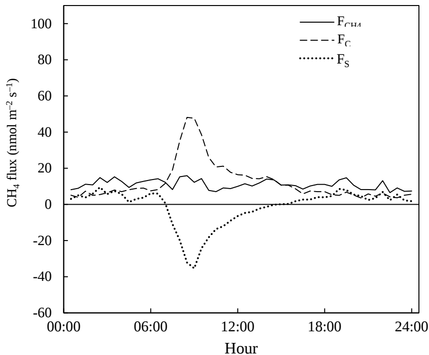
Figure 4.4 Ensemble mean diurnal variations in net ecosystem CH 4 exchange ( F_{CH_4} ), eddy CH 4 flux ( F_C ) and CH 4 storage change ( F_S ) from February 2014 to January 2017.
