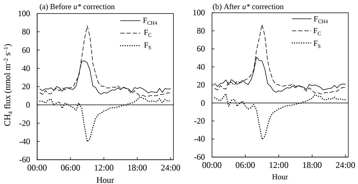
Figure 3.4 Ensemble mean diurnal variations in net ecosystem CH 4 exchange ( F_{CH_4} ), eddy CH 4 flux ( F_C ) and CH 4 storage change ( F_S ) from February 2014 to January 2017 (a) before friction velocity ( u^* ) correction and (b) after u^* correction.
