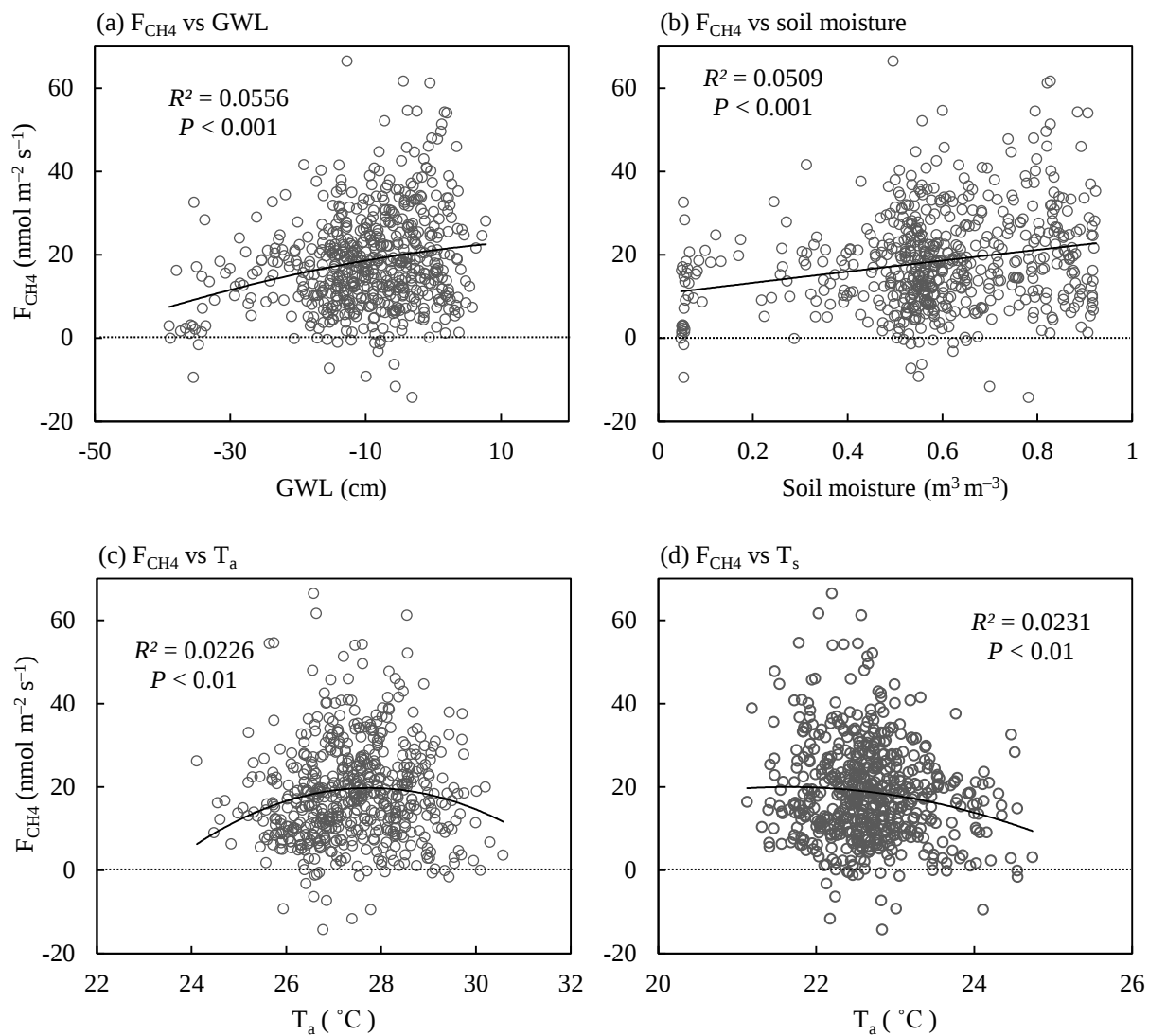
Figure 3.6 Responses of net ecosystem \text{CH}_4 exchange ( F_{\text{CH}_4} ) to (a) groundwater level (GWL), (b) soil moisture, (c) air temperature ( T_a ) and (d) soil temperature ( T_s ) on a daily basis. The relationships were determined using measured data and regression curves were drawn.
