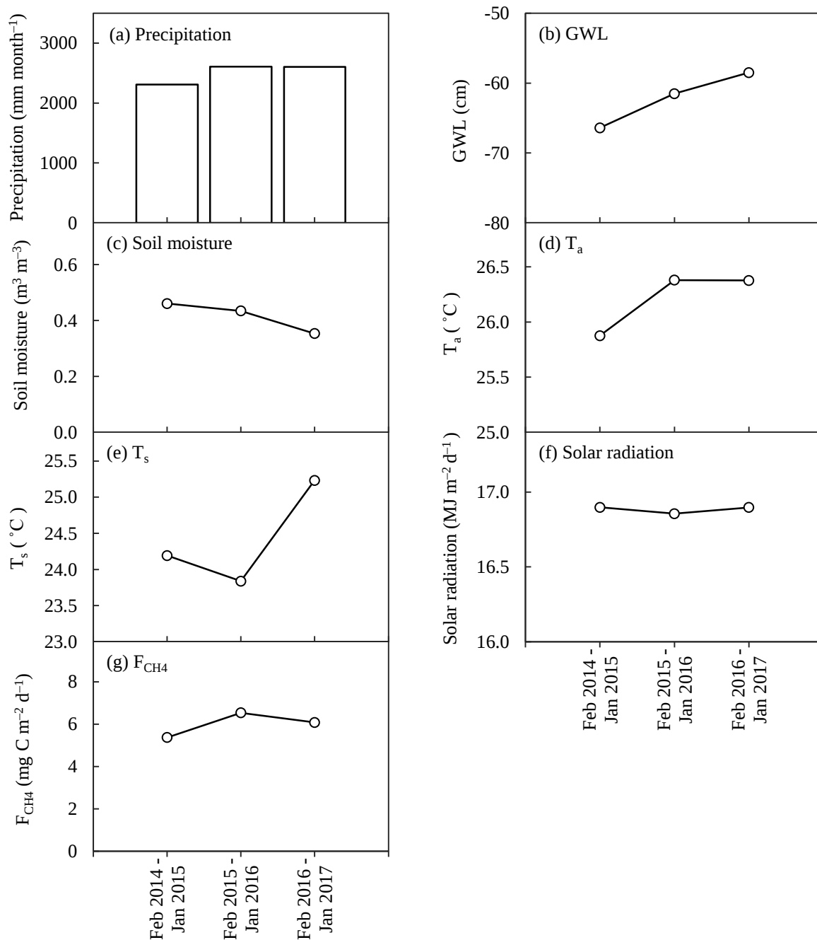
Figure 5.3 Variations in annual (a) precipitation (b) groundwater level (GWL), (c) soil moisture, (d) air temperature (T a ), (e) soil temperature (T s ), (f) solar radiation and (g) gap-filled daily net ecosystem CH 4 exchange (F CH4 ) from February (Feb) 2014 to January (Jan) 2017.
