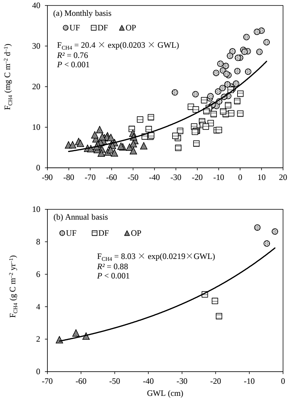
Figure 6.2 Relationships between gap-filled net ecosystem CH_4 exchange ( F_{CH_4} ) and groundwater level (GWL) on (a) monthly basis and (b) annual bases. An exponential curve was significantly fitted.
