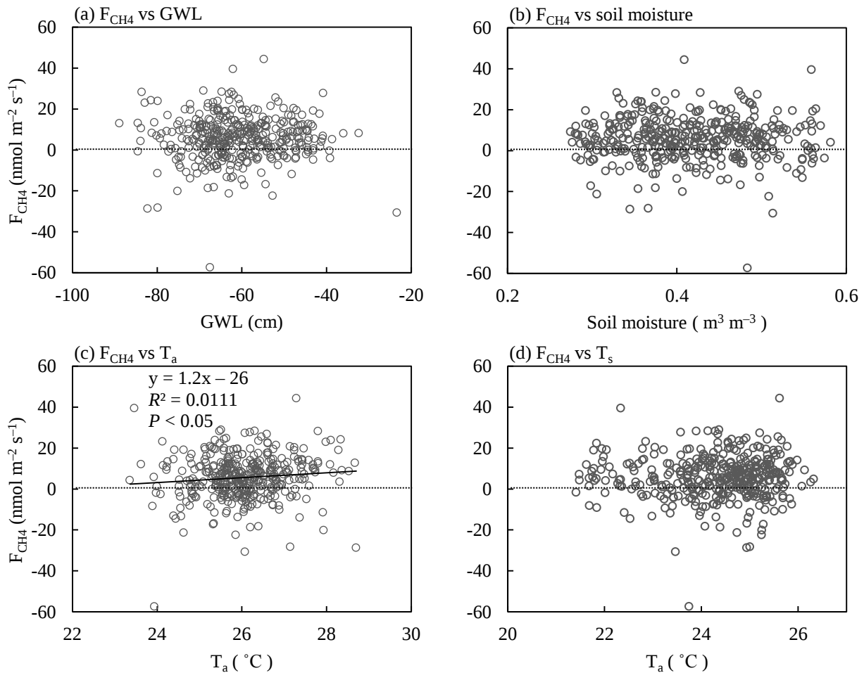
Figure 5.6 Responses of net ecosystem CH_4 exchange ( F_{CH_4} ) to (a) groundwater level (GWL), (b) soil moisture, (c) air temperature ( T_a ) and (d) soil temperature ( T_s ) on a daily basis. The relationships were determined using measured data and regression line was drawn.
