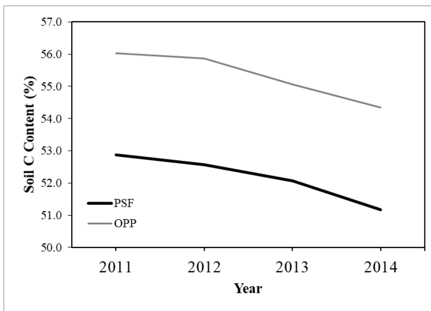
Figure 20. Total soil C content of PSF and OPP from 2011 to 2014
