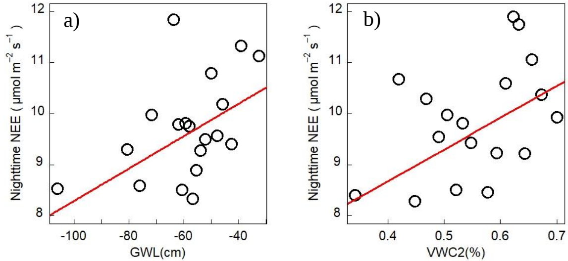
Figure 14. Relationship between nighttime NEE and GWL (a) or VWC (b). Red lines are drawn for significant correlation ( P < 0.05 ).
