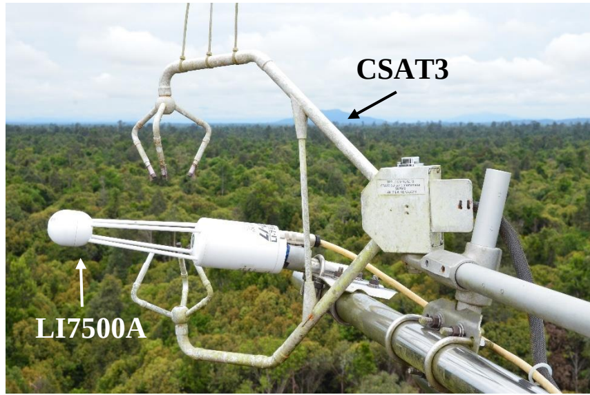
Figure 3. open-path \text{CO}_2/\text{H}_2\text{O} analyzer (LI7500A, Li-Cor Inc.) and a sonic anemometer/thermometer (CSAT3, Campbell Scientific Inc., Logan, UT, USA).
