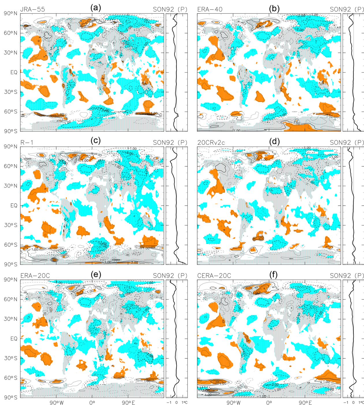
Figure 6. As for Fig. 2, but based on the 1958–2001 MLR analysis for each of six reanalysis data sets. The contour interval is 0.5 K, without 0.0 K lines. Coloured shading denotes anomalies that are positive (orange) or negative (blue) with magnitudes exceeding 1 SD of the 3-month mean R(t) at that location.
