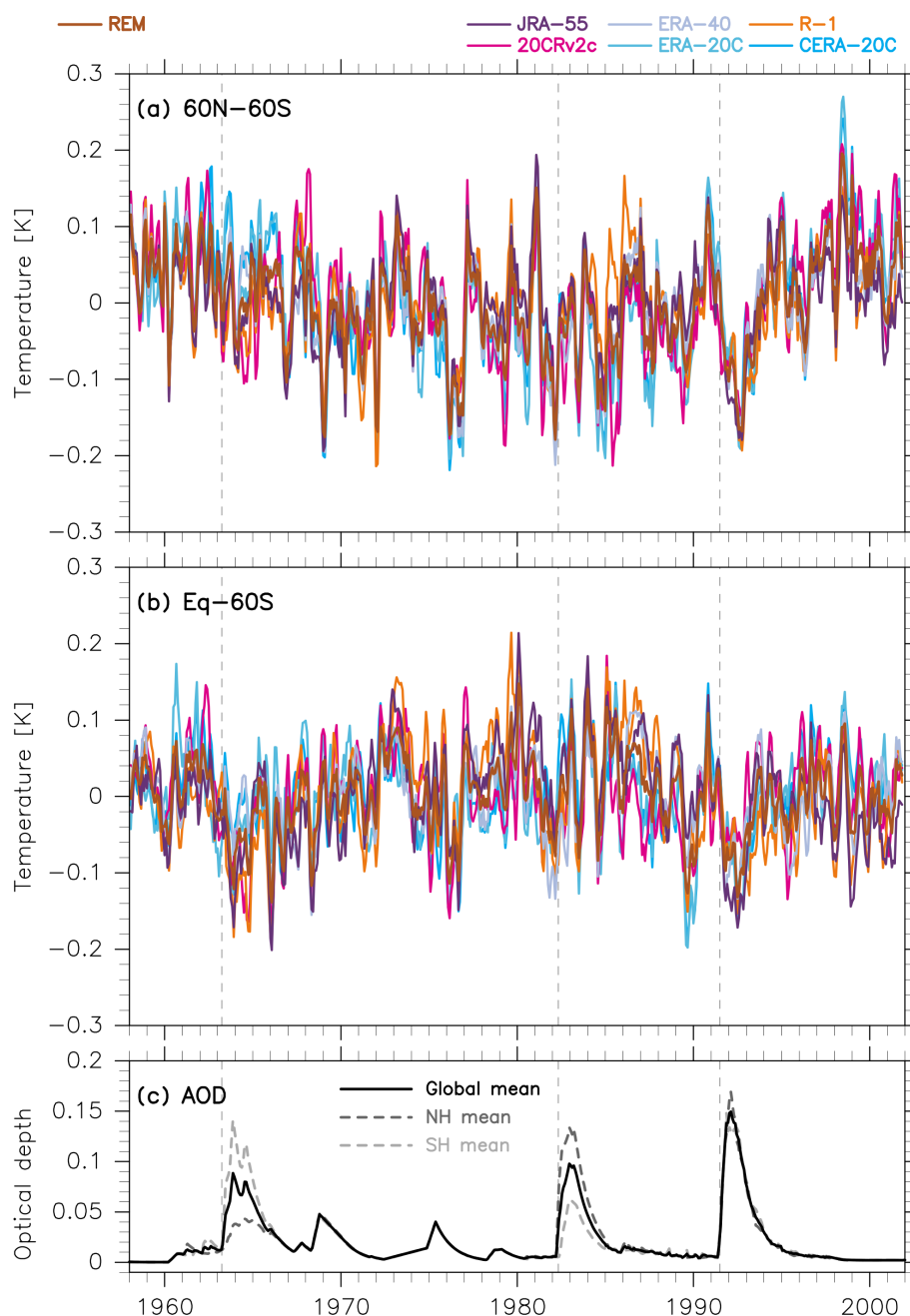
Figure 5. As for Fig. 1, but based on the 1958–2001 MLR analyses for six reanalysis data sets; averages for Equator–60° S are shown in panel (b). For all panels, vertical dashed lines indicate the starting date of the three volcanic eruptions.
