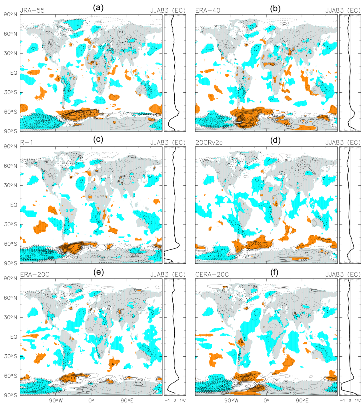
Figure 7. As for Fig. 4, but based on the 1958–2001 MLR analysis for each of six reanalysis data sets. The contour interval is 0.5 K, without 0.0 K lines. Coloured shading denotes anomalies that are positive (orange) or negative (blue) with magnitudes exceeding 1 SD of the 3-month mean R(t) at that location.
