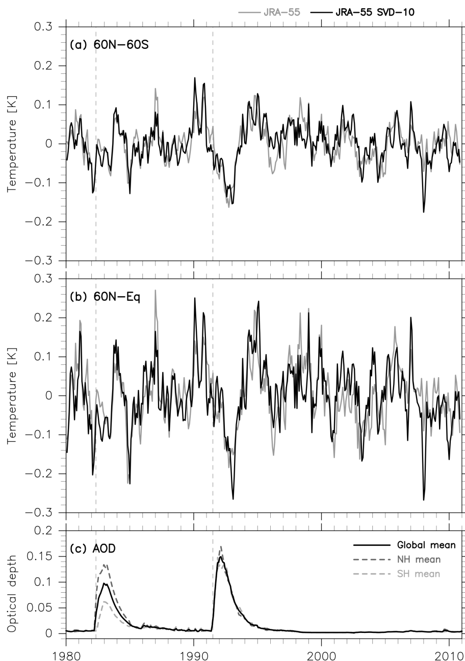
Figure A3. As for Fig. 1, but showing results for the primary method (i.e. as shown in Fig. 1; grey) versus results for the SVD method with the first 10 cross-covariance components (black) using JRA-55 data.
