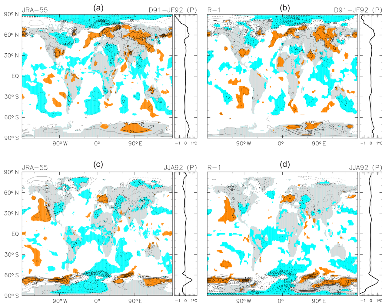
Figure 3. As for Fig. 2, but for the anomalies averaged from December 1991 to February 1992 (a, b) and from June to August 1992 (c, d) following the Mount Pinatubo eruption as calculated using JRA-55 (a, c) and R-1 (b, d). The contour interval is 0.5 K, without 0.0 K lines. Coloured shading denotes anomalies that are positive (orange) or negative (blue) with magnitudes exceeding 1 SD of the 3-month mean R(t) at that location.
