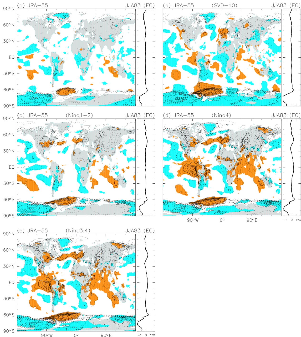
Figure A2. As for Fig. A1, but for the JJA 1983 anomalies following the El Chichón eruption in April 1982. The contour interval is 0.5 K, without 0.0 K lines. Coloured shading denotes anomalies that are positive (orange) or negative (blue) with magnitudes exceeding 1 SD of the 3-month mean R(t) at that location
