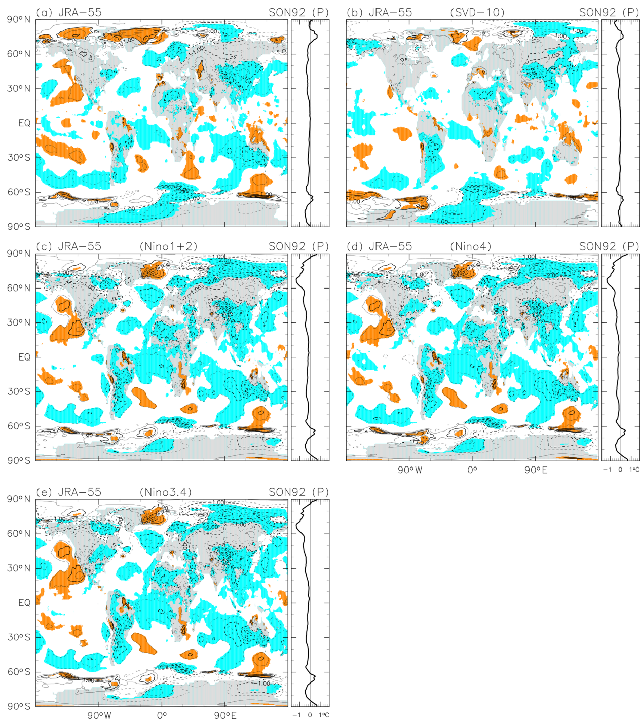
Figure A1. As for Fig. 2, but comparing different methods to obtain the 2 m temperature anomalies in SON 1992 following the Mount Pinatubo eruption. Only the JRA-55 reanalysis data set is used, with (a) the primary method, as in Fig. 2a, (b) the SVD method with the first 10 cross-covariance components, (c) the single-Niño method with the Niño 1 + 2 index, (d) the single-Niño method with the Niño 4 index, and (e) the single-Niño method with the Niño 3.4 index. See text for the details of each method. The contour interval is 0.5 K, without 0.0 K lines. Coloured shading denotes that anomalies are positive (orange) or negative (blue) with absolute magnitudes larger than 1 SD of the 3-month mean R(t) at that location.
