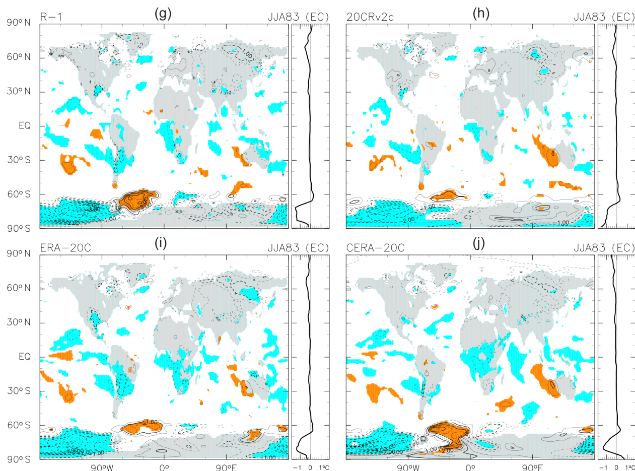
Figure 4. As for Fig. 2, but for the anomalies averaged over June to August 1983 following the El Chichón eruption in April 1982. The contour interval is 0.5 K, without 0.0 K lines. Coloured shading denotes anomalies that are positive (orange) or negative (blue) with magnitudes exceeding 1 SD of the 3-month mean R(t) at that location.
