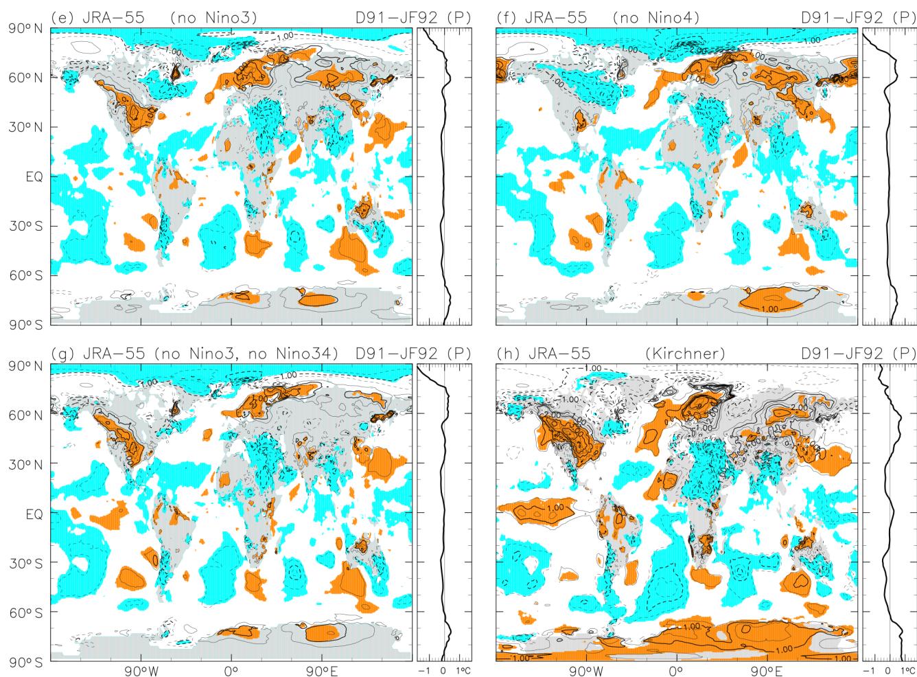
Figure B1. Similar to Fig. A1, but for the anomalies averaged from December 1991 to February 1992 following the Mount Pinatubo eruption using JRA-55 and with changes to panels (b)–(e) and with additions of panels (f)–(h). (a) The primary result as in Fig. 3a, (b) the result using the primary method but without the El Niño Modoki index, (c) the result using the primary method but without the Niño 1 + 2 index, (d) the result using the primary method but without the Niño 3.4 index, (e) the result using the primary method but without the Niño 3 index, (f) the result using the primary method but without the Niño 4 index, (g) the result using the primary method but without the Niño 3 and Niño 3.4 indices, and (h) the anomalies with respect to the 1979–1993 means (for the same months of year) following Plate 1c of Kirchner et al. (1999). See text for the details of each method. The contour interval is 0.5 K, without 0.0 K lines. Coloured shading in (a)–(g) denotes anomalies that are positive (orange) or negative (blue) with absolute magnitudes larger than 1 SD of the 3-month mean R(t) . Coloured shading in (h) has a similar meaning but with anomalies evaluated against the SD of December–January–February (DJF)-mean data during 1979–1993.
