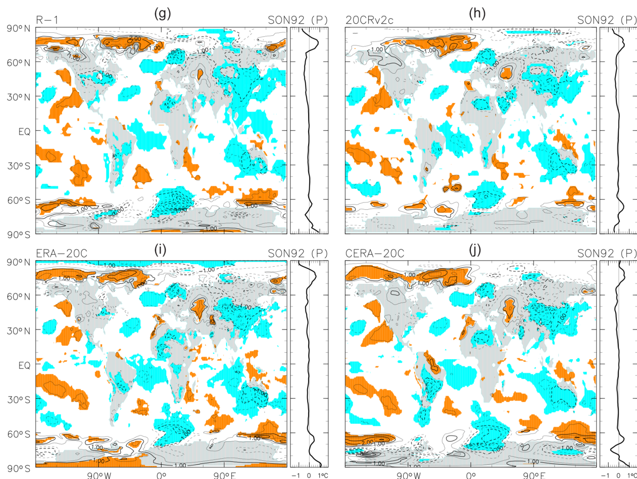
Figure 2. Geographical and zonal-mean distributions of the 2 m temperature anomalies averaged for September to November 1992 following the Mount Pinatubo eruption in June 1991. Results are based on the 1980–2010 MLR analyses for each of 10 reanalysis data sets (see the legend at the top of each panel). Solid and dashed contours denote positive and negative anomalies, respectively. The contour interval is 0.5 K, without 0.0 K lines. Coloured shading denotes anomalies that are positive (orange) or negative (blue) with magnitudes exceeding 1 standard deviation (SD) of the 3-month mean R(t) at that location.
