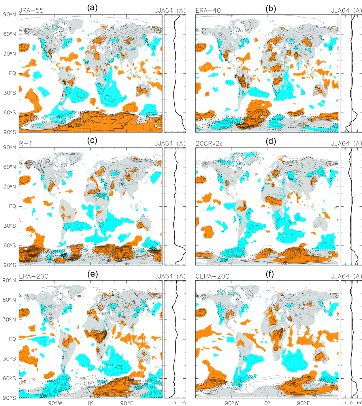
Figure 8. As for Fig. 7, but for the anomalies averaged over June to August 1964 following the Mount Agung eruption in March 1963. The contour interval is 0.5 K, without 0.0 K lines. Coloured shading denotes anomalies that are positive (orange) or negative (blue) with magnitudes exceeding 1 SD of the 3-month mean R(t) at that location.
