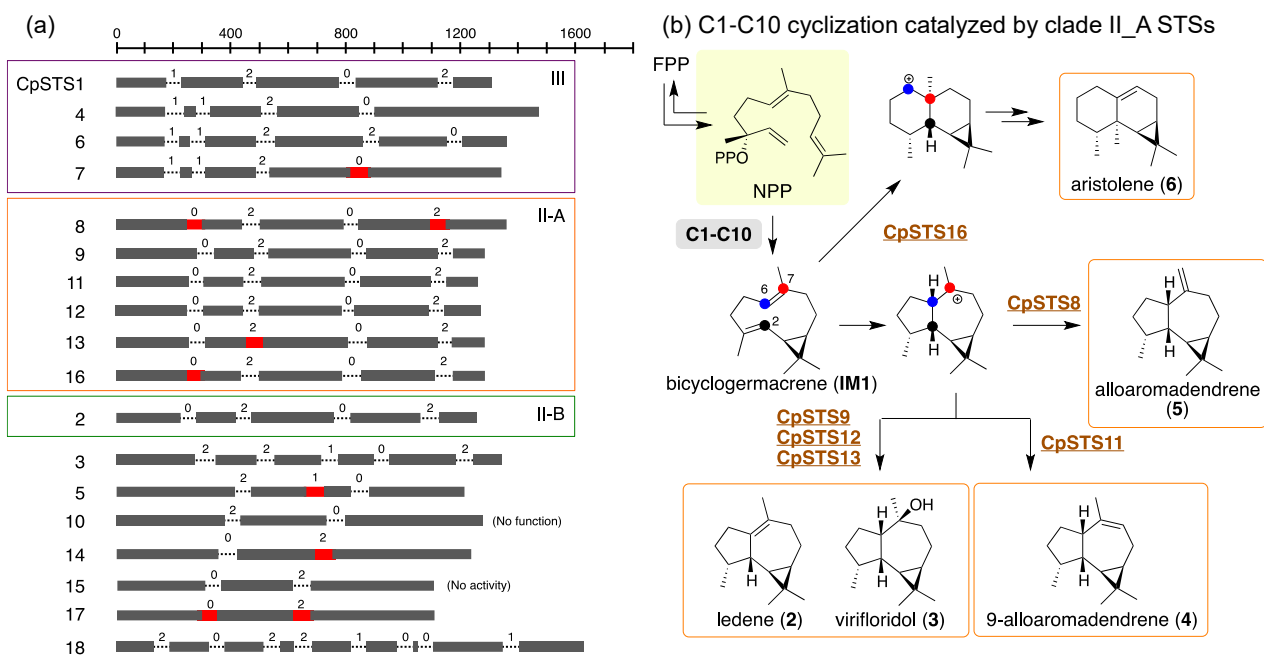
(c) C1-C11 cyclization catalyzed by clade III STSs
