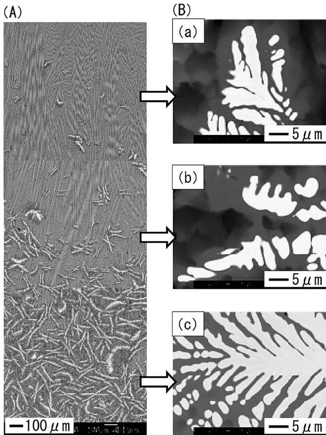
Fig. 2 Cross sectional microstructures for the as-melted sample #1 (Re-35 at%-45 at%Ni). (A) macrostructure and (B) microstructure, (a) upper position, (b) middle position, and (c) lower position.
