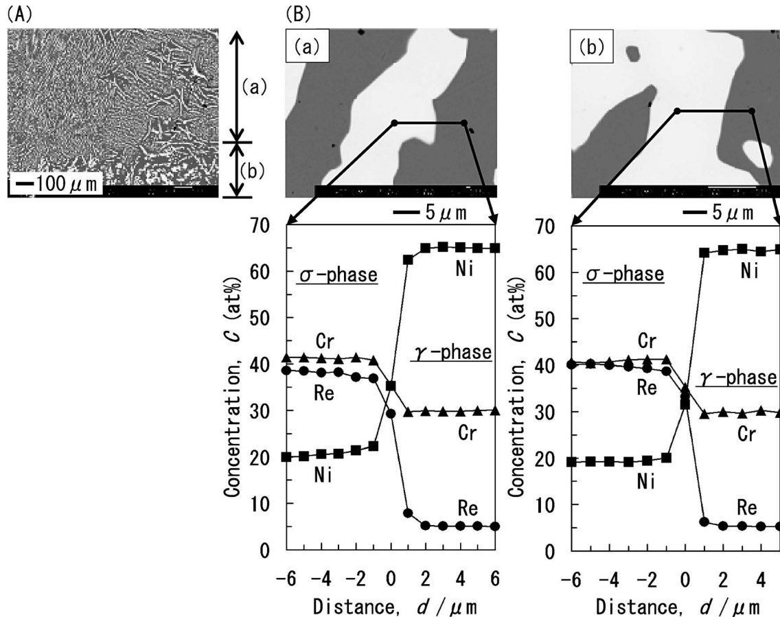
Fig. 4 Cross sectional microstructures and concentration profiles of Re, Cr and Ni measured lines for the sample #1 (Re-35 at%Cr-45 at%Ni). (A) macrostructure, and (B) microstructures of (a) and (b) in (A) after a heat-treatment at 1423 K for 8640 ks.
