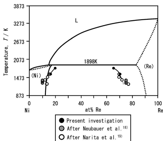
Fig. 11 Compositions of the \gamma and \delta phases of a binary Re-Ni system in contrast to those reported by Nash et al., Narita, and Neubauer et al.
