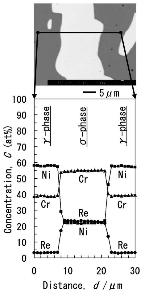
Fig. 5 Cross sectional microstructure and concentration profiles of Re, Cr and Ni measured lines for the sample #2 (Re-54.2 at%Cr-34 at%Ni) after a heat-treatment at 1423 K for 8640 ks.
