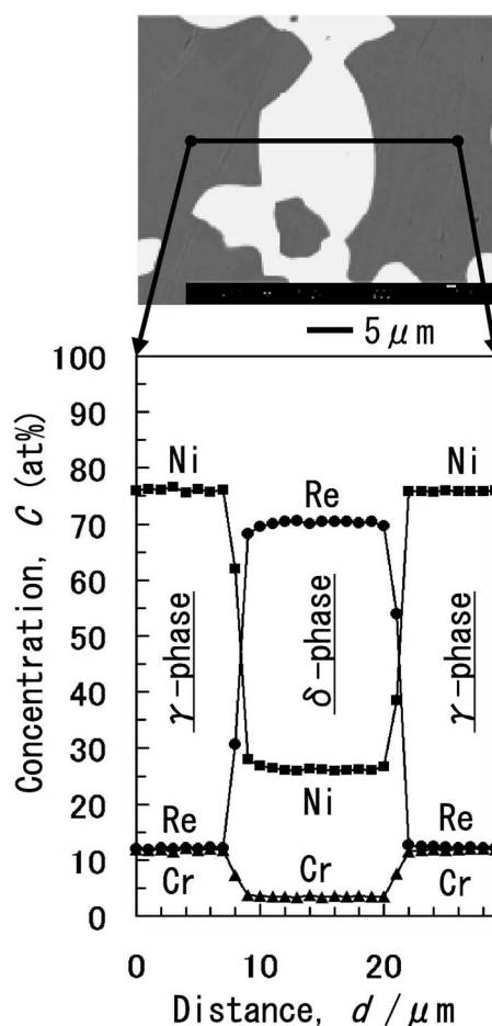
Fig. 7 Cross sectional microstructure and concentration profiles of Re, Cr and Ni measured lines for the sample #7 (Re-13.3 at%Cr-63.7 at%Ni) after a heat-treatment at 1423 K for 6840 ks.
