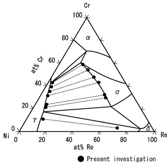
Fig. 9 Tie lines obtained in the present investigation plotted on the phase diagram of Re-Cr-Ni ternary system reported by Huang et al.
