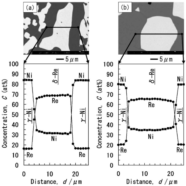
Fig. 10 Cross sectional microstructures and concentration profiles of Re and Ni measured along lines for the Re-40Ni alloy after heat-treatments. (a) for 7560 ks at 1573 K and (b) for 86.4 ks at 1773 K.
