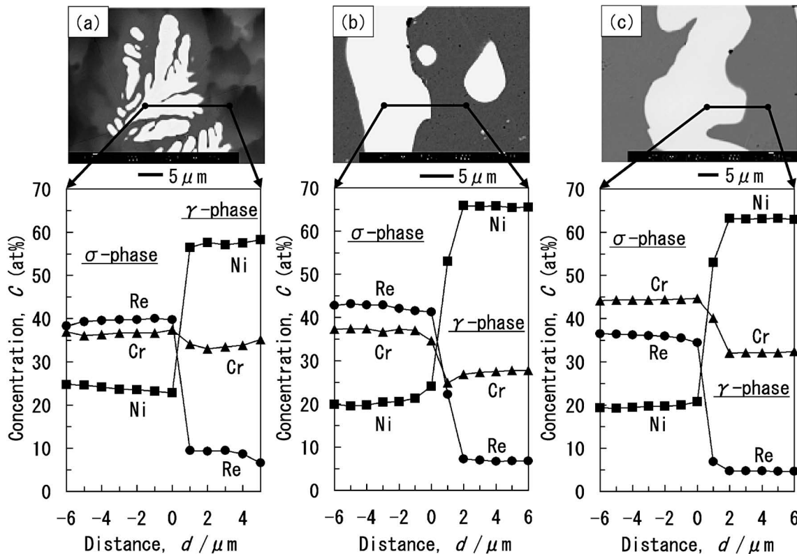
Fig. 3 Cross sectional microstructures and concentration profiles of Re, Cr and Ni measured lines for the sample #1 (Re-35 at%-45 at%Ni). (a) as-melted alloy, (b) and (c) after heat-treatment at 1423 K for 3600 ks and 8640 ks.
