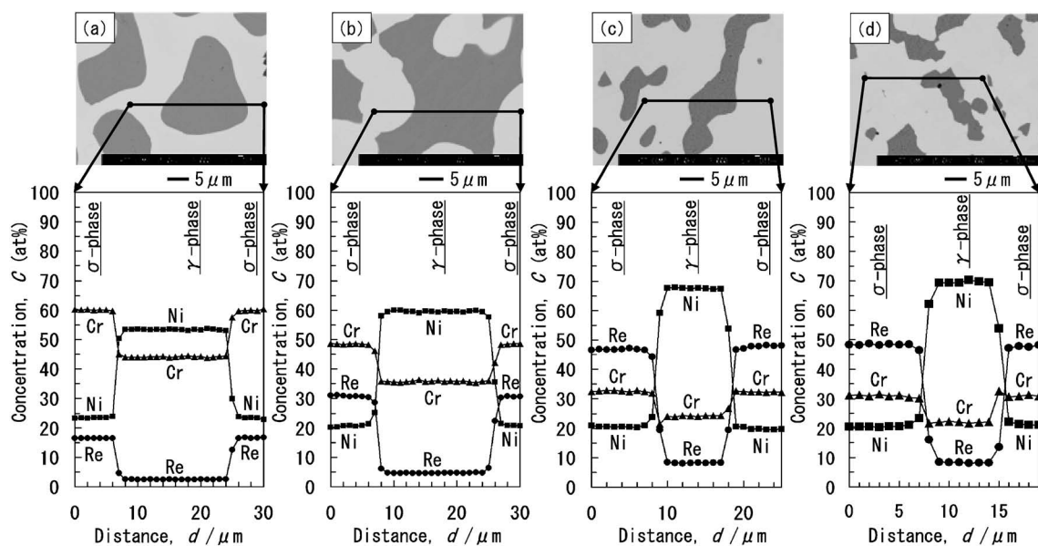
Fig. 6 Cross sectional microstructures and concentration profiles of Re, Cr and Ni measured lines for the alloys after heat-treatment at 1423 K for 5400 ks.
