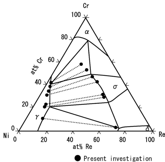
Fig. 8 Tie lines obtained in the present investigation plotted on the phase diagram of Re-Cr-Ni ternary system reported by Slyusarenko et al.
