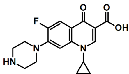
Ciprofloxacin
