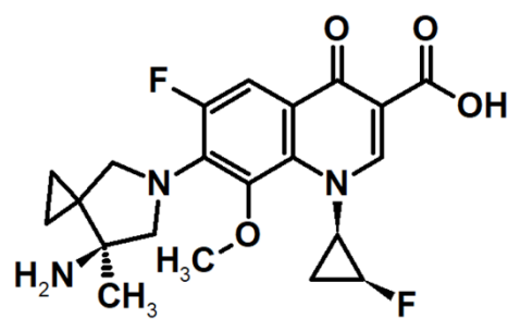
DC-159a
