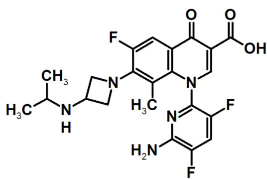
WQ-3810
