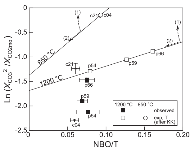
Fig. 8. \text{CO}_3^{2-}/\text{CO}_{2\text{mol}} ratios and NBO/T values observed in quenched glass samples and those estimated for high temperature melts. The NBO/T values were calculated based on Zotov et al. (1992), according to the assumption that OH serves as a network modifier while \text{H}_2\text{O}_{\text{mol}} does not. For estimation of the NBO/T values at experimental temperatures, we calculated the OH concentration before re-equilibration (Reaction (3)) based on the model of Ihinger et al. (1999), and used it to calculate the NBO/T values. Equilibrium \text{CO}_3^{2-}/\text{CO}_{2\text{mol}} ratios were estimated using the model proposed by Korschak and Keppler (2014): \ln(X_{\text{CO}_3^{2-}}/X_{\text{CO}_2}) = a + b/T , where a = -2.69 - 21.38 \times (\text{NBO/T}) , b = 1480 + 38810 \times (\text{NBO/T}) , and T is temperature in Kelvin. Arrow (1) indicates the increase in the \text{CO}_3^{2-}/\text{CO}_{2\text{mol}} ratio and the slight decrease in the NBO/T value as a result of low-temperature re-equilibration (the reaction (4) shifts to the right). Arrow (2) indicates the decrease in the \text{CO}_3^{2-}/\text{CO}_{2\text{mol}} ratio as a result of the decrease in NBO/T values caused by \text{H}_2\text{O} re-equilibration at low temperatures.
