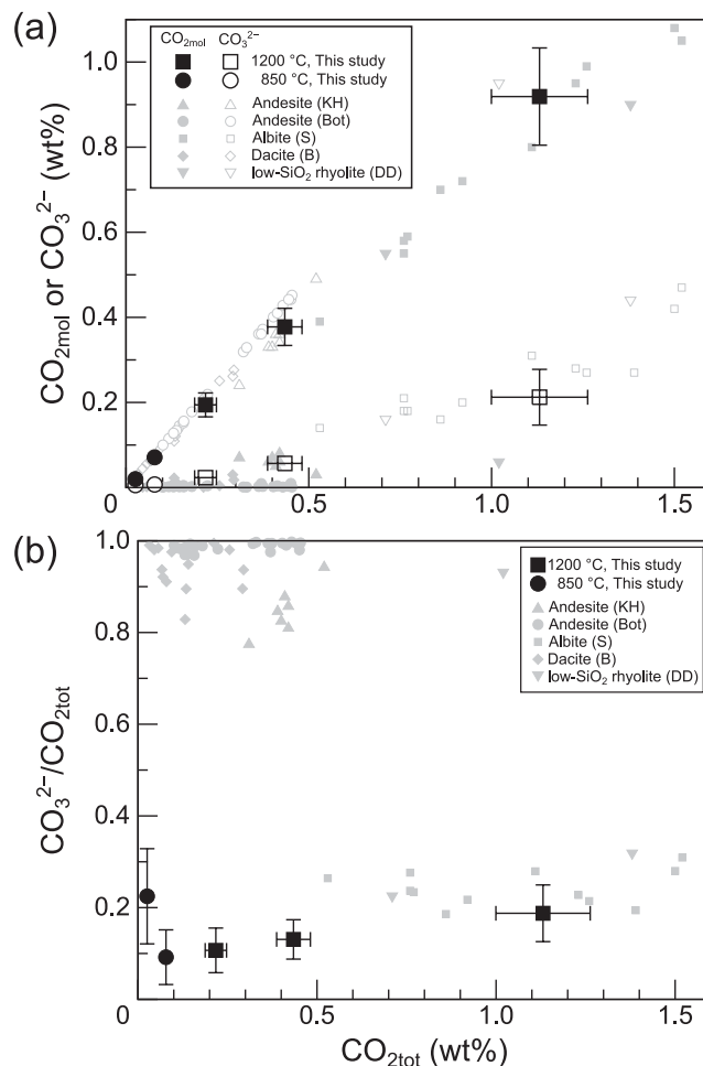
Fig. 4. (a) Concentrations of \text{CO}_{2\text{mol}} and \text{CO}_3^{2-} in rhyolitic glass as a function of total \text{CO}_2 content. Black squares: 1200 °C experiments; Black circles: 850 °C experiments. Solid symbols represent \text{CO}_{2\text{mol}} and open symbols represent \text{CO}_3^{2-} . Grey symbols represent data from previous studies, including albite melt (squares: 1.5–3 GPa, 1450–1625 °C, Stolper et al., 1987 (S)), andesite melt (triangles: King and Holloway, 2002 (KH); circles: Botcharnikov et al., 2006 (Bot)), dacite melt (diamonds: Behrens et al., 2004a (B)) and low-SiO 2 rhyolite (upside-down triangles: Duncan and Dasgupta, 2015 (DD)). (b) Fraction of \text{CO}_3^{2-} as a function of total \text{CO}_2 content. Run c21 (at 0.1 GPa) was accompanied by large error due to an insufficient content of \text{CO}_3^{2-} , and was not used in the thermodynamic calculations in Subsection “Thermodynamics of \text{CO}_{2\text{mol}} and \text{CO}_3^{2-} speciation and solubilities for rhyolitic melt”. Note that the \text{CO}_{2\text{mol}} content is higher than the \text{CO}_3^{2-} content for rhyolitic and albite melts while it is opposite for dacite and andesite melts.
