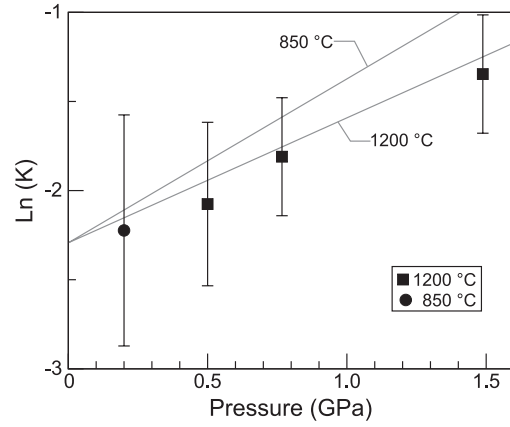
Fig. 10. Variation in equilibrium constant of reaction (6) ( K = X_{\text{CO}_3^{2-}}^{\text{melt}}/(X_{\text{CO}_2\text{mol}}^{\text{melt}}X_{\text{O}^{2-}}^{\text{melt}}) ) as a function of pressure. The symbols denote the following: ■, 1200 °C experiments; ●, 850 °C experiments. Lines are the best-fit isotherms at 850 and 1200 °C, described by Eq. (6). Parameters were calculated to be \Delta_rV = -8.6 \pm 0.9 \text{ cm}^3/\text{mol} and \Delta_rH = +1.1 \pm 4.4 \text{ kJ/mol} . Note that run c21 was not used in the fitting calculation and is not shown in this diagram.
