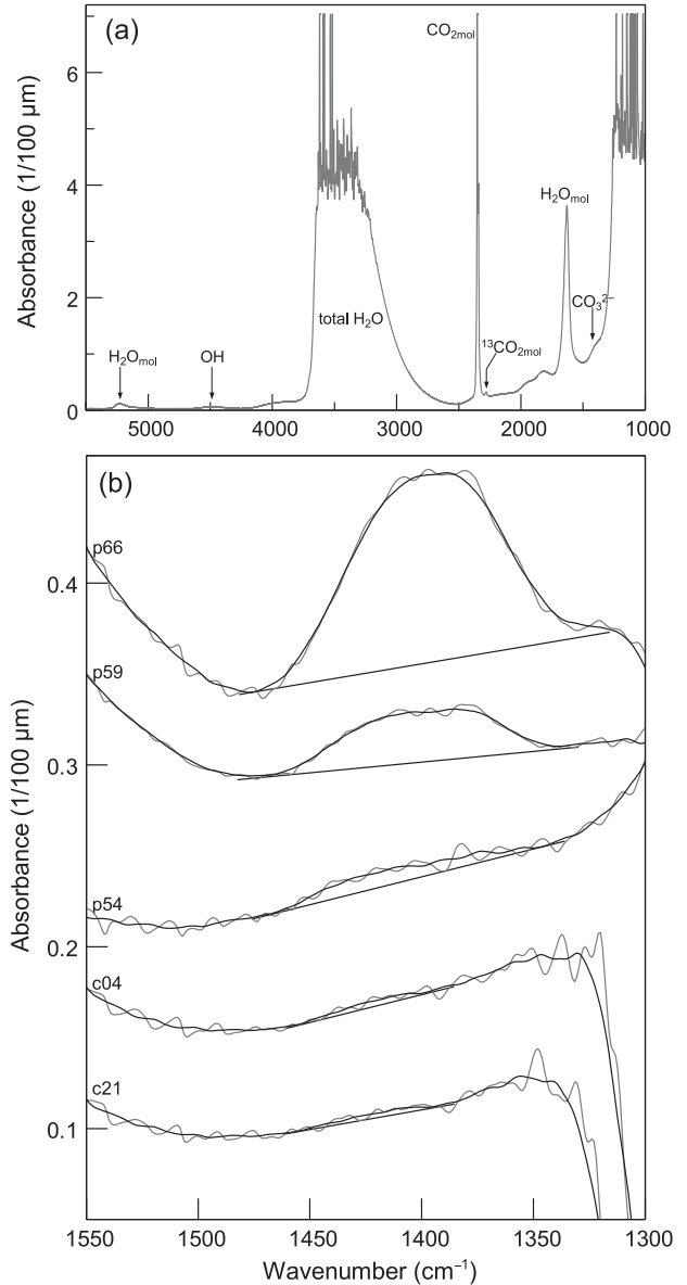
Fig. 2. (a) Typical IR spectrum of our experimental rhyolitic glass (run# p66). Peaks are observed at 1410\text{ cm}^{-1} (carbonate anions; \text{CO}_3^{2-} ), 1630\text{ cm}^{-1} ( \text{H}_2\text{O} molecules; \text{H}_2\text{O}_{\text{mol}} ), 2280\text{ cm}^{-1} ( ^{13}\text{CO}_2 molecules), 2350\text{ cm}^{-1} ( ^{12}\text{CO}_2 molecules; \text{CO}_{2\text{mol}} ), 3550\text{ cm}^{-1} (total \text{H}_2\text{O} ), 4500\text{ cm}^{-1} (hydroxyl groups, OH), and 5250\text{ cm}^{-1} ( \text{H}_2\text{O}_{\text{mol}} ). Spectra were normalised to wafer thickness of 100\text{ }\mu\text{m} . (b) Background-subtracted spectra of the experimental glasses, produced by subtracting the spectrum of \text{CO}_2 -free glass (starting obsidian) from each spectrum of experimental samples. Grey and black lines indicate original and smoothed (moving point averaged) spectra, respectively.
