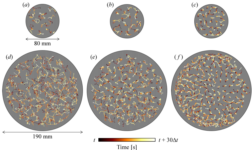
FIGURE 15. Path lines for advections of the columnar vortices for 90 s; (a) Ta = 1.0 \times 10^7 , (b) 3.0 \times 10^7 , and (c) 1.0 \times 10^8 with \Gamma = 2.00 , and (d) Ta = 1.0 \times 10^7 , (e) 3.0 \times 10^7 , and (f) 1.0 \times 10^8 with \Gamma = 4.75 , where the evolution of the path lines is displayed using colour coding. Backgrounds are grey for better visibility.
