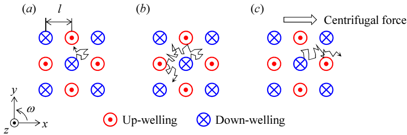
FIGURE 18. Conceptual diagram of the vortex motion without centrifugal force effects (a) t_{\text{life}} < \tau and (b) t_{\text{life}} \geq \tau , and with centrifugal force effects (c) t_{\text{life}} \gg \tau .
