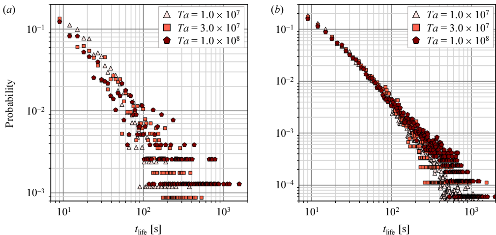
FIGURE 14. Probability distributions of lifetimes, t_{\text{life}} of columnar vortices for (a) \Gamma = 2.00 , and (b) \Gamma = 4.75 .
