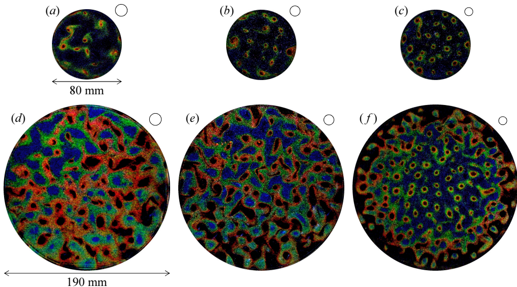
FIGURE 9. Examples of horizontal temperature fields visualized using encapsulated TLCs at z = 0.75H for (a) Ta = 1.0 \times 10^7 , (b) 3.0 \times 10^7 , and (c) 1.0 \times 10^8 with \Gamma = 2.00 , and (d) Ta = 1.0 \times 10^7 , (e) 3.0 \times 10^7 , and (f) 1.0 \times 10^8 with \Gamma = 4.75 . Open circles appearing on the upper right of each image indicate the horizontal scale of the columnar vortices predicted by Sakai (1997).
