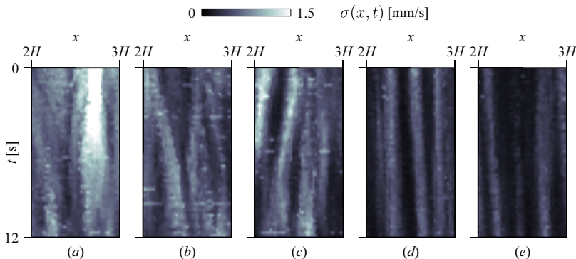
FIGURE 7. Time series of the standard deviations for the vertical velocity component at horizontal positions 2H < x < 3H : (a) Ta = 1.0 \times 10^6 ( Ro = 1.20 ), (b) Ta = 6.0 \times 10^6 (0.49), (c) 1.0 \times 10^7 (0.38), (d) 6.0 \times 10^7 (0.15), and (e) 1.0 \times 10^8 (0.12).
