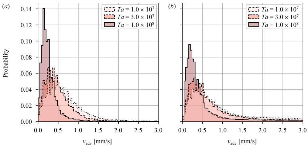
FIGURE 10. Probability distributions of horizontal advection speeds of columnar vortices v_{\text{adv}} for three different values of Ta ; (a) \Gamma = 2.00 , and (b) \Gamma = 4.75 .
