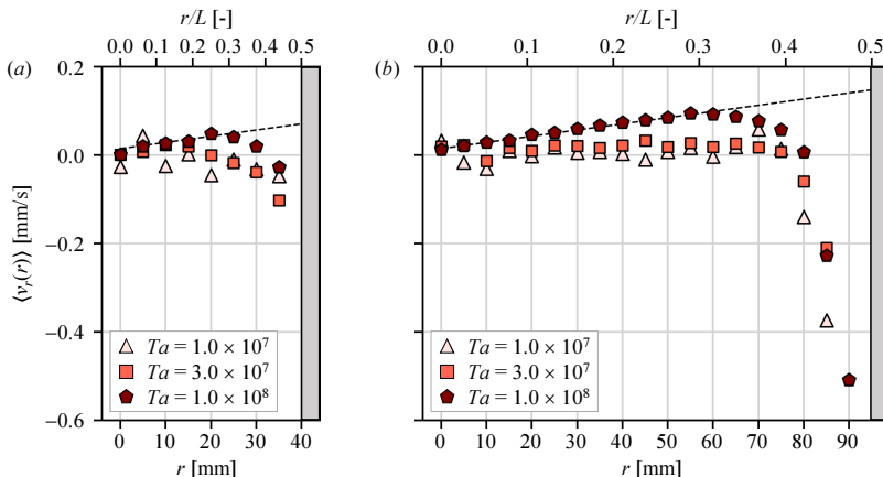
FIGURE 12. Radial position dependence of ensemble averaged radial advection velocity \langle v_r \rangle ; (a) \Gamma = 2.00 , and (b) \Gamma = 4.75 . Each plot is an average of 5 mm domains. Dashed line drawn in the panels is \langle v_r(r) \rangle = 0.0014r + 0.0143 obtained by a least-squares fit.
