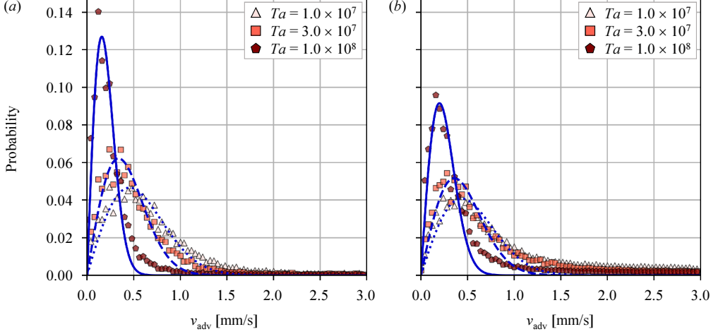
FIGURE 13. PDFs fitted by the Maxwell distribution; the original PDF data are from figure 10 for the three different Ta settings with (a) \Gamma = 2.00 , and (b) \Gamma = 4.75 vessels.
