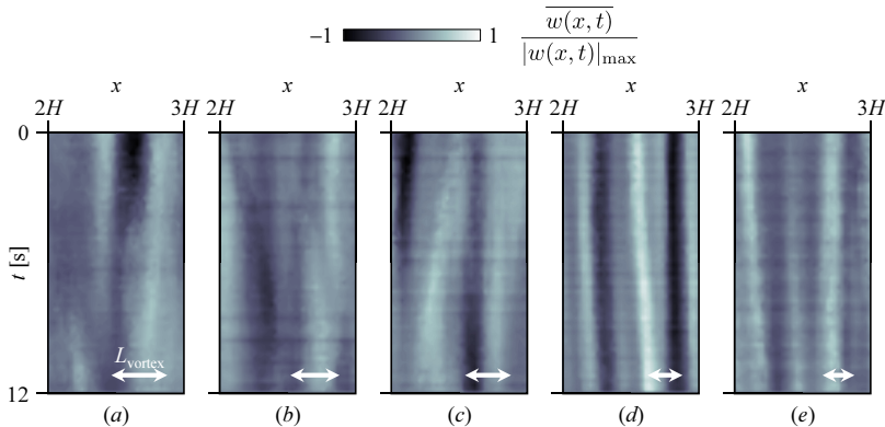
FIGURE 6. Time series of averaged vertical velocities at horizontal positions 2H < x < 3H : (a) Ta = 1.0 \times 10^6 ( Ro = 1.20 ), (b) Ta = 6.0 \times 10^6 (0.49), (c) 1.0 \times 10^7 (0.38), (d) 6.0 \times 10^7 (0.15), and (e) 1.0 \times 10^8 (0.12). Two-headed arrows indicate the theoretically predicted diameter of the columnar vortices L_{\text{vortex}} derived by Sakai (1997).
