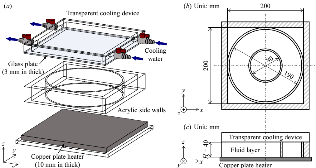
FIGURE 1. Schematic diagram of the fluid vessel: (a) Overview of the vessel with the acrylic walls, cooling device, and copper plate heater. The cylinder inside the square walled vessel is that of L = 190 mm. (b) Horizontal cross-section of the vessel, where two different cylinders ( L = 80 or 190 mm) are alternatively placed. (c) Vertical cross-section of the vessel.
