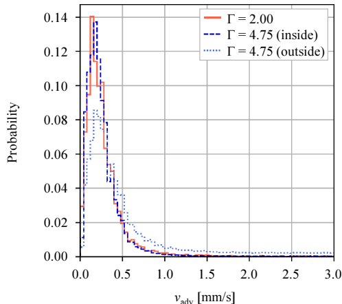
FIGURE 11. Probability distribution at Ta = 1.0 \times 10^8 with \Gamma = 2.00 (solid line) and separated plots of \Gamma = 4.75 from different regions; (inside) r \leq 40 mm (dashed line) and (outside) r > 40 mm (dotted line).
