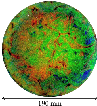
FIGURE 3. An example of a horizontal temperature field visualized using the encapsulated TLC at z = 0.75H for Ra = 1.0 \times 10^7 , and Ta = 0 recorded in the \Gamma = 4.75 vessel.
