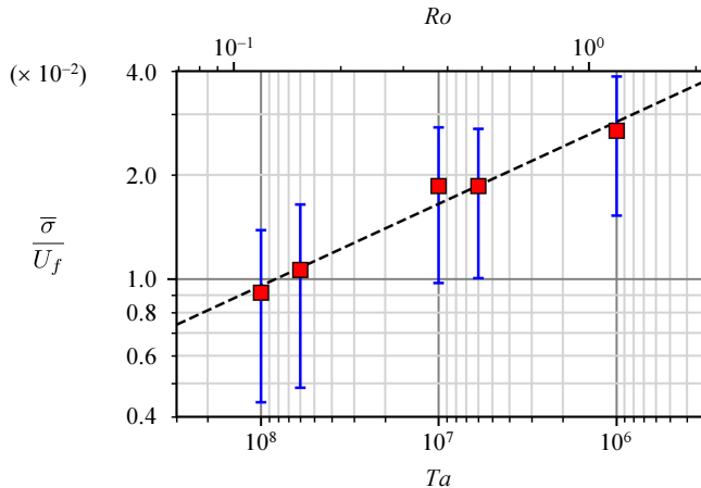
FIGURE 8. Variation of local duration characteristics \bar{\sigma} plotted with error bars giving the standard deviation. Here, \bar{\sigma} is normalized by the free-fall velocity U_f . The dashed line is a least-squares fit of \bar{\sigma}/U_f = 0.026 Ro^{0.47}
