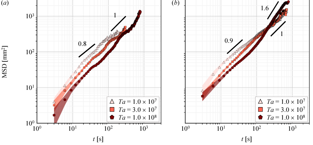
FIGURE 17. Mean squared displacement (MSD) \langle \delta \mathbf{r}(t)^2 \rangle of the horizontal motion of columnar vortices for different Ta values with (a) \Gamma = 2.00 , and (b) \Gamma = 4.75 . The numbers accompanying the black solid lines are the \gamma values. Faded-colour areas behind each plot indicate the standard deviation of the MSD.
