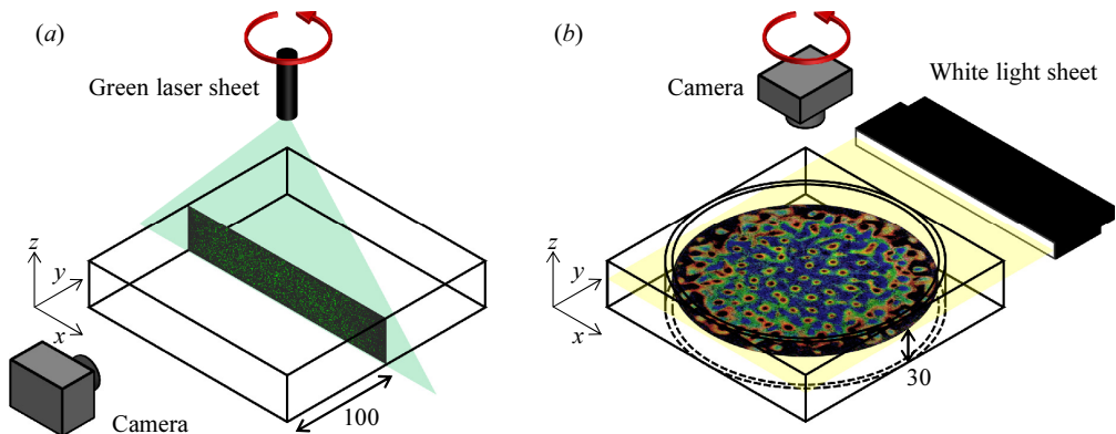
FIGURE 2. Optical arrangements for (a) the vertical velocity field measurements by PIV and (b) the horizontal temperature field measurements by TLC particles. Images embedded in each panel are examples obtained by these two different visualization methods. For the experiments the fluid vessel and optical equipment was placed on a platform and rotated as suggested by the red arrows.
