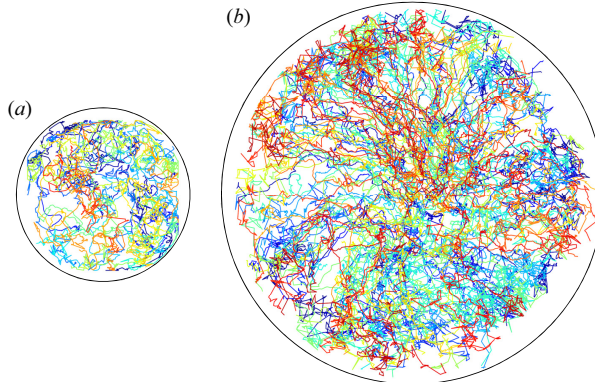
FIGURE 16. Examples of path lines of columnar vortices persisting over 450 s with Ta = 1.0 \times 10^8 ; (a) \Gamma = 2.00 , and (b) \Gamma = 4.75 . Path lines are individually colour coded.
