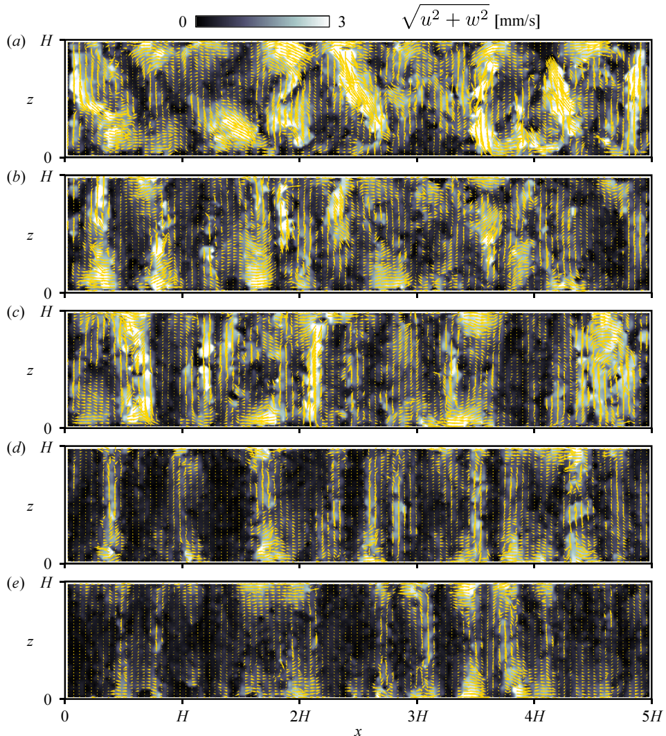
FIGURE 4. Snapshots of the velocity vector distributions of vertical cross-sections measured in PIV at y = 2.5H : (a) Ta = 1.0 \times 10^6 ( Ro = 1.20 ), (b) Ta = 6.0 \times 10^6 (0.49), (c) 1.0 \times 10^7 (0.38), (d) 6.0 \times 10^7 (0.15), and (e) 1.0 \times 10^8 (0.12). Only every second vector (the slanted yellow line) is plotted for clearer visibility.
