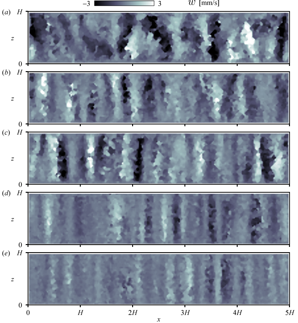
FIGURE 5. Vertical velocity distributions w(x, z) in vertical cross-sections at the same moment to that of figure 4 measured by PIV at y = 2.5H : (a) Ta = 1.0 \times 10^6 (Ro = 1.20) , (b) Ta = 6.0 \times 10^6 (0.49) , (c) 1.0 \times 10^7 (0.38) , (d) 6.0 \times 10^7 (0.15) , and (e) 1.0 \times 10^8 (0.12) .
