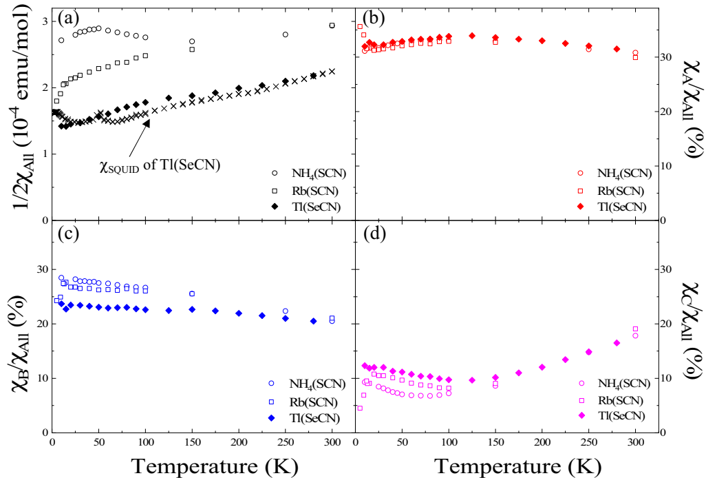
FIG. 6. Temperature dependence of (a) total spin susceptibilities ( \chi_{\text{All}} = 2\chi_A + \chi_B + \chi_C ) and (b)–(d) ratios of local spin susceptibilities ( \chi_i/\chi_{\text{All}} ; i = A, B , and C ). The black stars denote the spin susceptibility of \text{Tl}(\text{SeCN}) evaluated by SQUID measurements ( \chi_{\text{SQUID}} ). The results of \text{NH}_4(\text{SCN}) and \text{Rb}(\text{SCN}) were calculated using the temperature dependence of NMR shifts in the literature [16,17].
