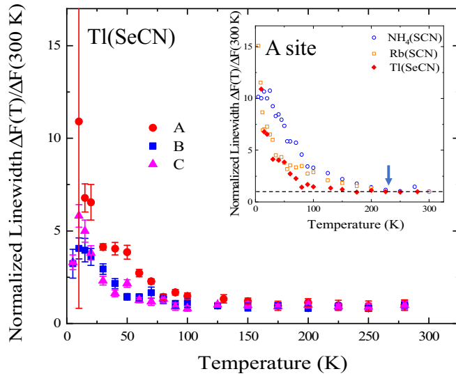
FIG. 7. Temperature dependence of the line width of the NMR shifts of the A, B, and C sites in Tl(SeCN) normalized relative to those at 300 K. The error bars indicate the uncertainty of the fits. The inset shows the temperature dependence of the line widths of the A sites in \text{NH}_4(\text{SCN}) [17], \text{Rb}(\text{SCN}) [16], and \text{Tl}(\text{SeCN}) .
