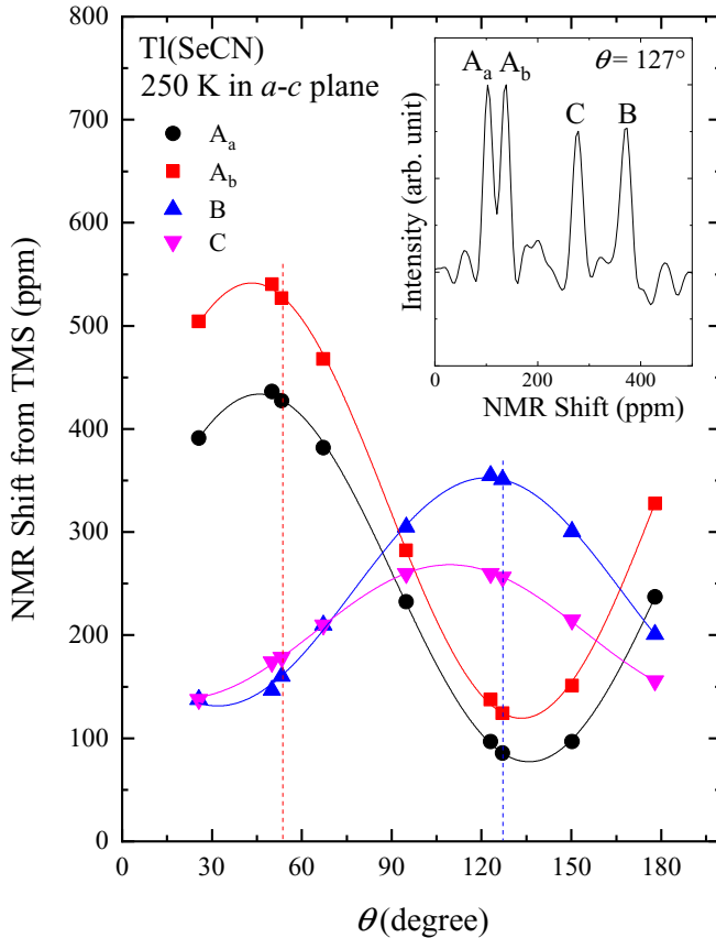
FIG. 3. Angular dependence of the NMR shift of the Tl(SeCN) around the b^* axis at 250 K. The dashed lines denote the field direction of the \theta = 54^\circ and 127^\circ . The inset shows the NMR peaks of each nonequivalent 13 C site, A_a , A_b , B, and C at \theta = 127^\circ .
