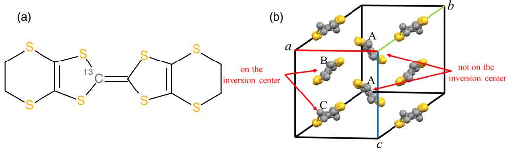
FIG. 2. (a) Molecular structure of BEDT-TTF. The molecule was selectively enriched in 13 C to prevent the Pake doublet effect. (b) Donor layer of \alpha -type salts viewed along the b axis.
