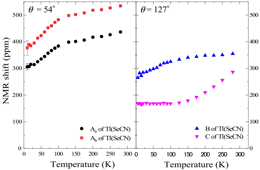
FIG. 5. Temperature dependence of the NMR shift of Tl(SeCN). The NMR shift of the A_a and A_b sites were measured at \theta = 54^\circ and those of the B and C sites at \theta = 127^\circ . The error bars indicate the uncertainty of the fits.
