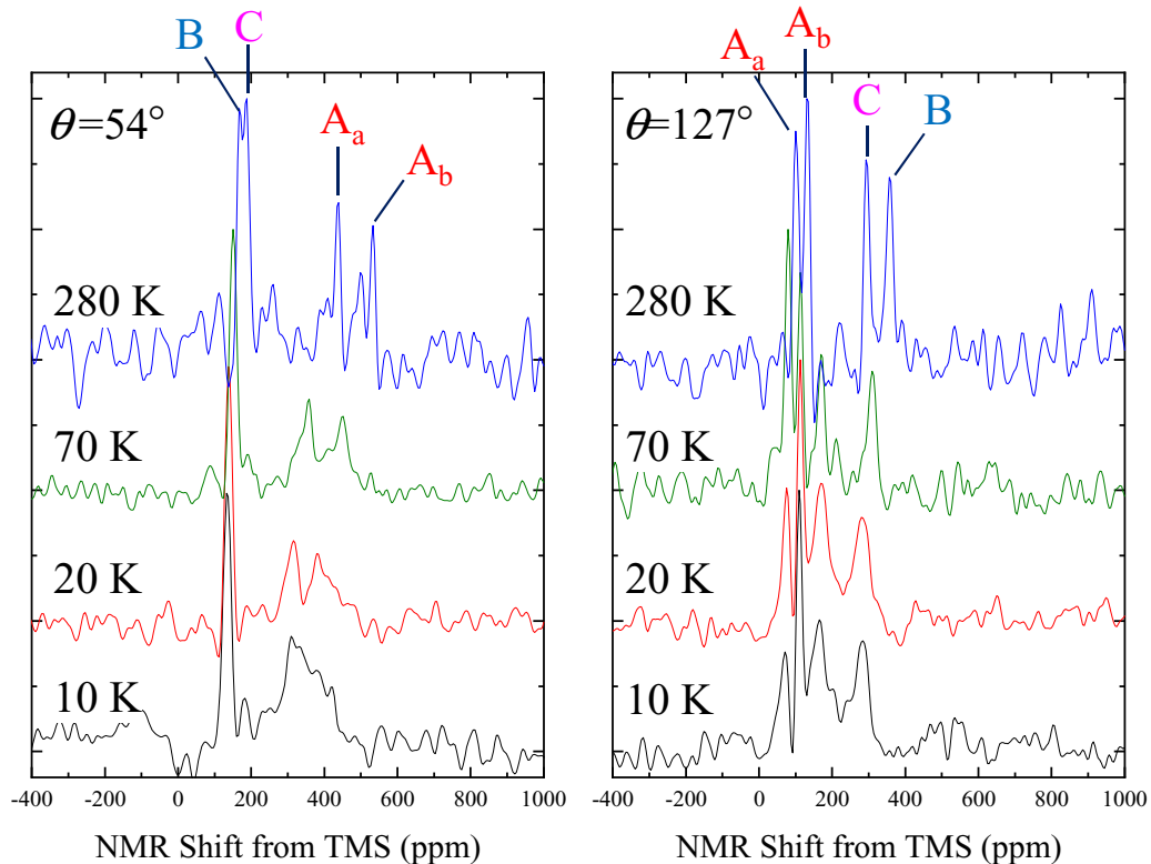
FIG. 4. NMR spectrum of Tl(SeCN) with \theta = 54^\circ and 127^\circ at several temperatures.
