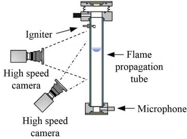
Fig. 1 Schematic representation of the experimental apparatus.
