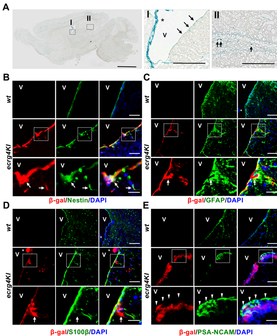
Fig. 1. Increased Ecrg4 promoter activity in the ventricular zone/subventricular zone, the ependymal cell layer and hippocampus. (A) X-gal staining (blue) of frozen brain sections of 6-month-old Ecrg4KI mice. High-magnification images are on the right: I, VZ/SVZ; II, DG. Arrows indicate X-gal + cells. Asterisk indicates the choroid plexus. (B-E) Immunostaining of brain sections of 6-month-old wild-type and Ecrg4KI mice for \beta -gal (red), which represents Ecrg4 expression, and the neural markers (green) nestin (B), GFAP (C), S100 \beta (D) and PSA-NCAM (E). Bottom row shows higher-magnification images of the boxed regions. Arrows show the cells leaving the VZ. Arrowheads show the developing neuronal precursor cells. Stars show the choroid plexus. All nuclei are counterstained with DAPI (blue). V, lateral ventricle. Scale bars: 2 mm in A; 200 \mu m and 50 \mu m (bottom row) in B-E.
