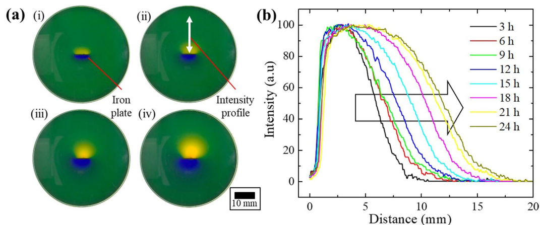
Figure 4. (a) Image of BTB agar gel with Fe plate inserted for 24 hours (i) 0.5 hours (ii) 3 hours (iii) 12 hours (iv) 24 hours. (b) The colour intensity spectra for 3–24 hours.
