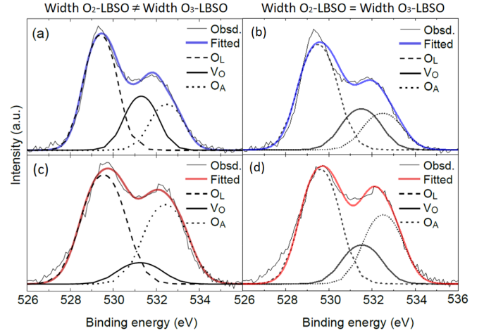
FIG. 2. Oxygen 1s XPS spectrum of (a) and (b) 126-nm-thick O_2 -LBSO and (c) and (d) 140-nm-thick O_3 -LBSO films. The peaks are deconvoluted into lattice oxygen ( O_L ), oxygen vacancy ( V_O ), and adsorbed oxygen ( O_A ). The oxygen vacancy peak is attributed to the oxygen atoms adjacent to oxygen vacancies, and the adsorption peak is attributed to surface contaminations by organic molecules (i.e., oxidized hydrocarbon, adsorbed water). If O_2 LBSO and O_3 LBSO are fitted independently (a) and (c), the oxygen vacancy peak is significantly reduced. If the peak widths of O_2 LBSO and O_3 LBSO are constrained to be the same, the difference in the oxygen vacancy peak is suppressed, but the O_3 -LBSO film still exhibits a smaller V_O/O_L ratio (Table I).
