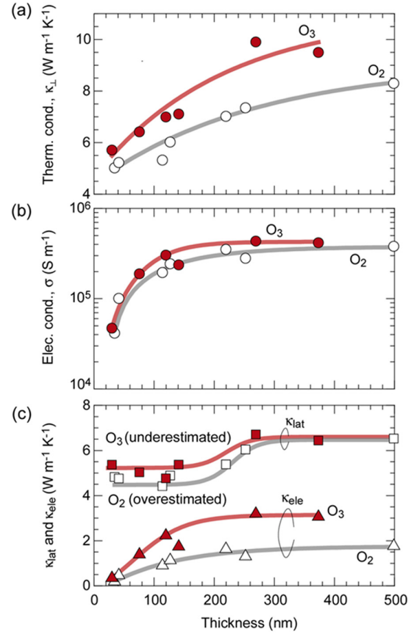
FIG. 6. (a) Observed through-plane thermal conductivity ( \kappa_{\perp} ) at RT. The \kappa_{\perp} of the O_3 -LBSO films are always greater than that of O_2 -LBSO films. (b) Electrical conductivity ( \sigma ) of the LBSO films at RT. (c) Estimated electron and lattice thermal conductivities of LBSO films. The electron thermal conductivities for O_2 -LBSO films were underestimated ( L = 1.5 \times 10^{-8} \text{ W}^{-1} \Omega^{-1} \text{ K}^2 ) whereas those for O_3 -LBSO films were overestimated ( L = 2.45 \times 10^{-8} \text{ W}^{-1} \Omega^{-1} \text{ K}^2 ). Although a higher Lorenz number was chosen for O_3 -LBSO films, they still show higher \kappa_{\text{lat}} compared to O_2 -LBSO films.
