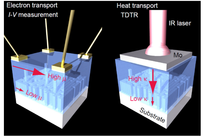
FIG. 1. The thickness dependence of the transport properties observed in this paper. All transport properties of LBSO films near the film/substrate interface are lower than those away from the interfaces. Studies on the point defect formations in LBSO films [17,18,22] suggest oxygen vacancies can also be related to the transport properties of LBSO films, and this paper, indeed, showed that the thickness gradient can be affected by the oxidation condition during the film deposition process.
