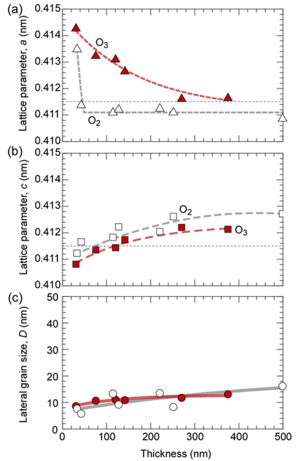
FIG. 4. Lattice characteristics of the LBSO films. (a) In-plane ( a -axis) lattice constants of LBSO films. (b) Out-of-plane ( c -axis) lattice constants of LBSO films. (c) The lateral grain sizes of the LBSO films calculated by Scherrer's equation, which represent the threading dislocation densities. The uncertainty in the lattice parameters is 0.0005 nm, which comes from the bin size of the RSMs (bin size \times 10 ). At small thicknesses, O_2 -LBSO films have lower lattice strains compared to O_3 -LBSO films. However, as the films become thicker, the lattice strains in O_3 -LBSO films become smaller than those in O_2 -LBSO films.
