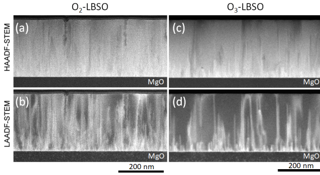
FIG. 3. STEM micrographs of the LBSO films. (a) HAADF-STEM and (b) LAADF-STEM micrographs of a 250-nm O_2 -LBSO film. (c) HAADF-STEM and (d) LAADF-STEM micrographs of a 270-nm O_3 -LBSO film. Near the film/substrate interface, the LAADF contrast of O_3 -LBSO films is slightly lower than that of O_2 -LBSO films. However, the LAADF contrast away from the interface is drastically lower in the O_3 -LBSO films. This shows that highly oxidative atmospheres greatly reduced the lattice strains in the film.
