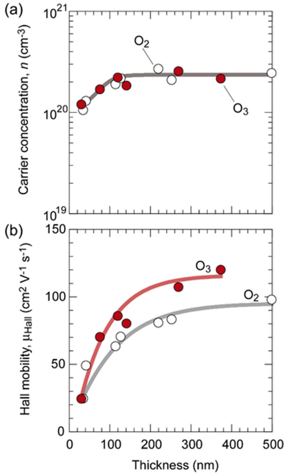
FIG. 5. Electron transport properties of LBSO films fabricated in O_2 and O_3 atmospheres. (a) Carrier concentration n against the film thickness. (b) Hall mobility \mu_{\text{Hall}} (= \mu_e) against the film thickness. The \mu_{\text{Hall}} of the O_3 -LBSO films are always greater than that of the O_2 -LBSO films.
