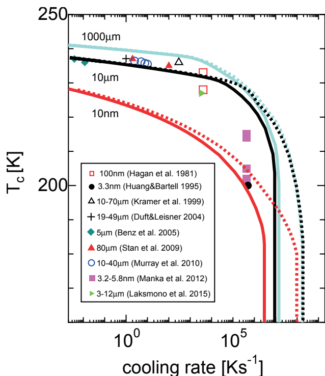
Fig. 8 The crystallization temperatures at various cooling rates obtained by our model in the ASW and SCL diffusivity scenarios (solid and dotted curves, respectively) and in the previous experiments of homogeneous ice nucleation (symbols). The particle size is varied as 10 nm, 10 \mu\text{m} , and 1000 \mu\text{m} . The critical cooling rates for vitrification are respectively 2.9 \times 10^6 \text{ Ks}^{-1} , 8.9 \times 10^6 \text{ Ks}^{-1} , and 1.4 \times 10^7 \text{ Ks}^{-1} , for 10 nm, 10 \mu\text{m} , and 1000 \mu\text{m} in the ASW diffusivity, and 9.6 \times 10^7 \text{ Ks}^{-1} , 1.8 \times 10^8 \text{ Ks}^{-1} , and 1.8 \times 10^8 \text{ Ks}^{-1} , for 10 nm, 10 \mu\text{m} , and 1000 \mu\text{m} in the SCL diffusivity.
