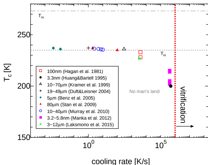
Fig. 1 Crystallization temperature versus cooling rate in various experiments of homogeneous ice nucleation of water droplets shown in Table 1. T_H (= 235 \text{ K}) is called the homogeneous nucleation temperature. The water droplets vitrify at extremely large cooling rates \gtrsim 10^6 - 10^7 \text{ Ks}^{-1} .
