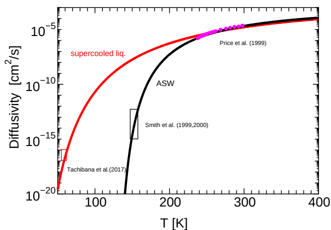
Fig. 2 Diffusion coefficients of amorphous ice (ASW, black) given by Eq.(14) 25,26 and supercooled liquid water (SCL, red) given by Eq.(15) 27 as functions of temperature. The diffusivity at T = 60 \text{ K} obtained by 28 with the use of D = kT/(6\pi\eta r_0) with viscosity \eta , is also shown.
