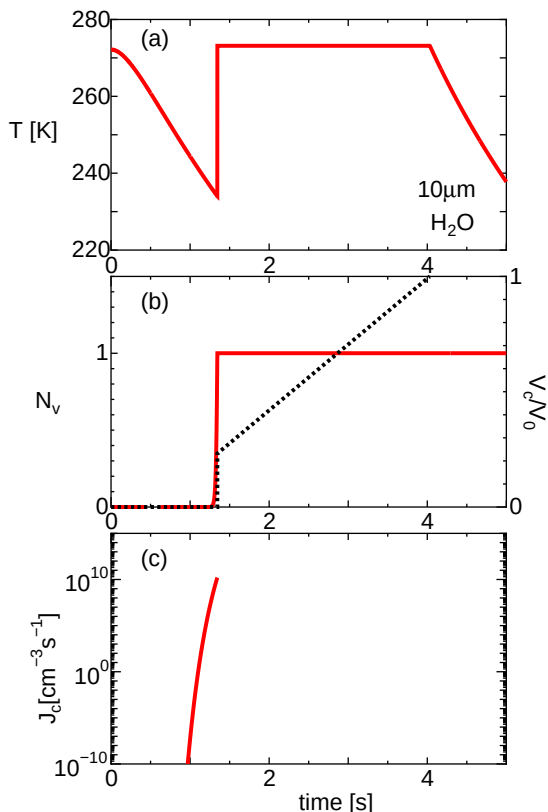
Fig. 3 (a) Time evolutions of droplet temperature, (b) number of critical nuclei in the droplet (left vertical axis, red solid line) and volume ratio between the crystal and initial volumes (right vertical axis, black dotted line), and (c) nucleation rate. The droplet is 10 \mu\text{m} in size, and the cooling rate is 30 \text{Ks}^{-1} .
