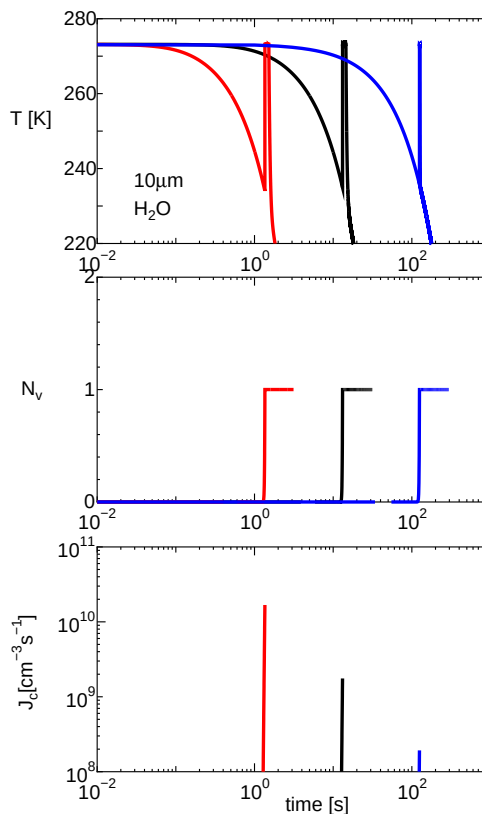
Fig. 4 Same as Fig. 3 but for various cooling rates (30 \text{Ks}^{-1} (red), 3 \text{Ks}^{-1} (black), and 0.3 \text{Ks}^{-1} (blue)). The crystallization temperatures are 234, 235, and 236 K for cooling rates of 30 \text{Ks}^{-1} , 3 \text{Ks}^{-1} , and 0.3 \text{Ks}^{-1} , respectively. In all cases, the particle contains unity number of nuclei.
