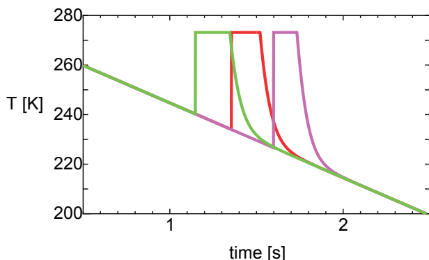
Fig. 7 Temperature evolution in the droplet particles with various interfacial tensions between the liquid and solid ( 0.9\sigma (green), \sigma , (red) and 1.1\sigma (purple)), where \sigma is given by Eq.(13). The droplet size is 10\text{ }\mu\text{m} and the cooling rate is fixed at 30\text{ K s}^{-1} .
