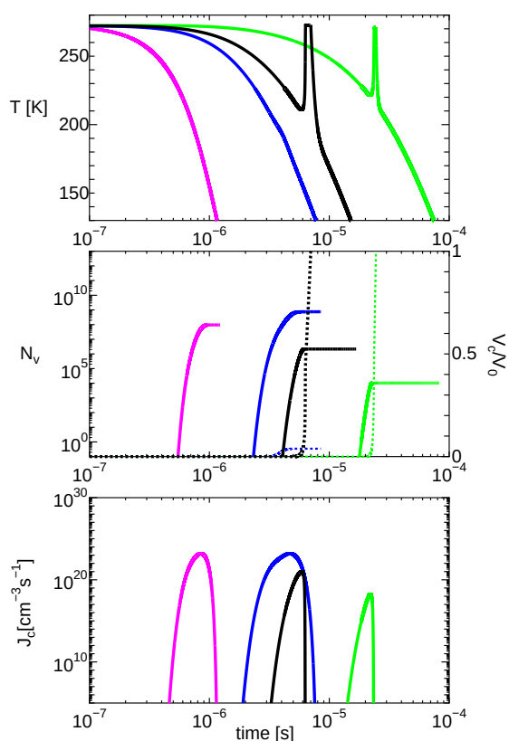
Fig. 5 Same as Fig. 3 but for various larger cooling rates. At cooling rates of 2.18 \times 10^6 \text{ Ks}^{-1} (green) and 1.07 \times 10^7 \text{ Ks}^{-1} (black), the crystallization temperatures are 221 K and 211 K, respectively, the numbers of critical nuclei are 1.03 \times 10^4 \text{ Ks}^{-1} and 2.16 \times 10^6 \text{ Ks}^{-1} , respectively, and the numbers of molecule included in a critical nucleus are 36 and 16, respectively. At much larger cooling rates (blue and pink curves correspond to the cooling rates of 2 \times 10^7 \text{ Ks}^{-1} and 1.3 \times 10^8 \text{ Ks}^{-1} , respectively), the crystallization hardly proceeds.
