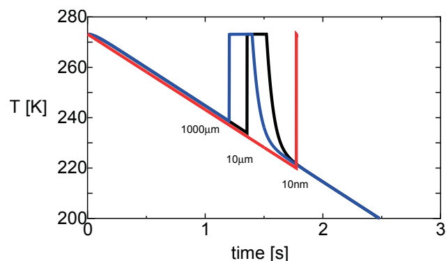
Fig. 6 Same as Fig. 3(a) but for various droplet sizes. The cooling rate is fixed at 30 \text{ Ks}^{-1} . The crystallization temperatures of 1000 \mu\text{m} , 10 \mu\text{m} , and 10 \text{ nm} particles are 242, 235, and 223 K for respectively.
