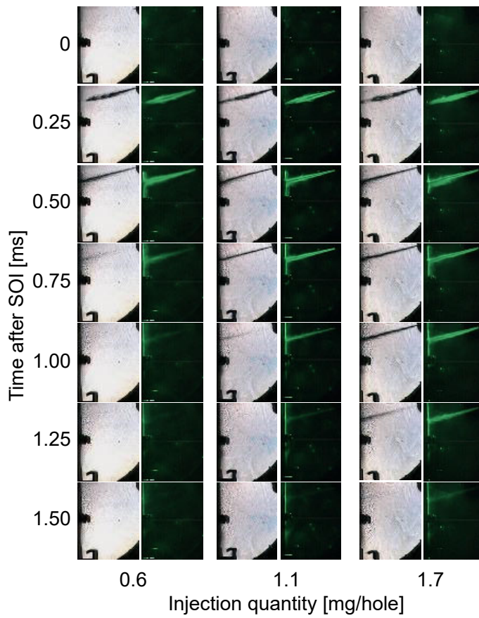
Figure 19. Observation of spray penetration and wall impingement at 90CA ATDC (left: shadowgraph, right: Mie scattering)
