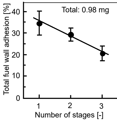
Figure 29. Total fuel wall adhesion percentage in multi stage fuel injection
