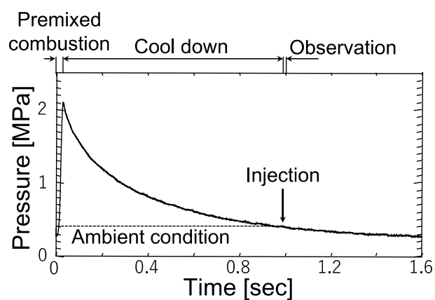
Figure 12. An example of the location of the target ambient atmosphere in the cooling process
