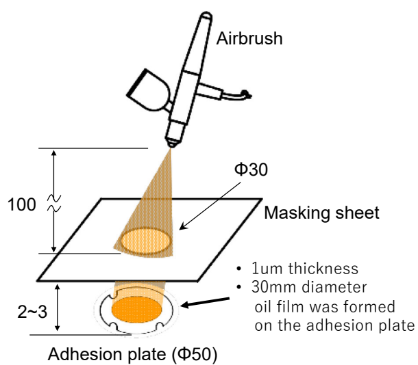
Figure 13. The method of applying lubricant oil film
