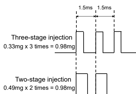
Figure 15. Time interval in multi-stage injections in Test 6
