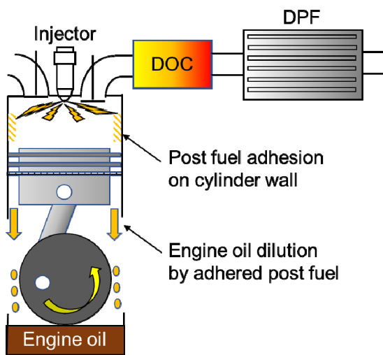
Figure 1. Image of DPF regeneration process
