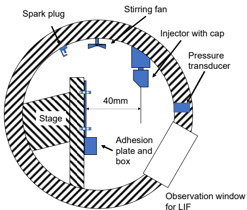
Figure 3. Internal structure of the constant volume chamber
