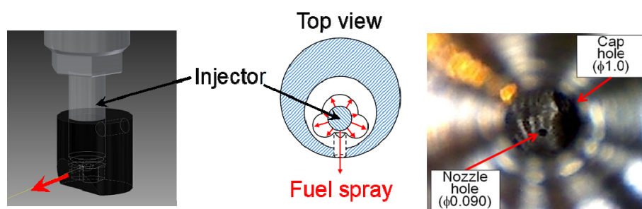
Figure 6. Outline of the injector cap (left and middle) and a microscope image of nozzle hole with injector cap (right)
