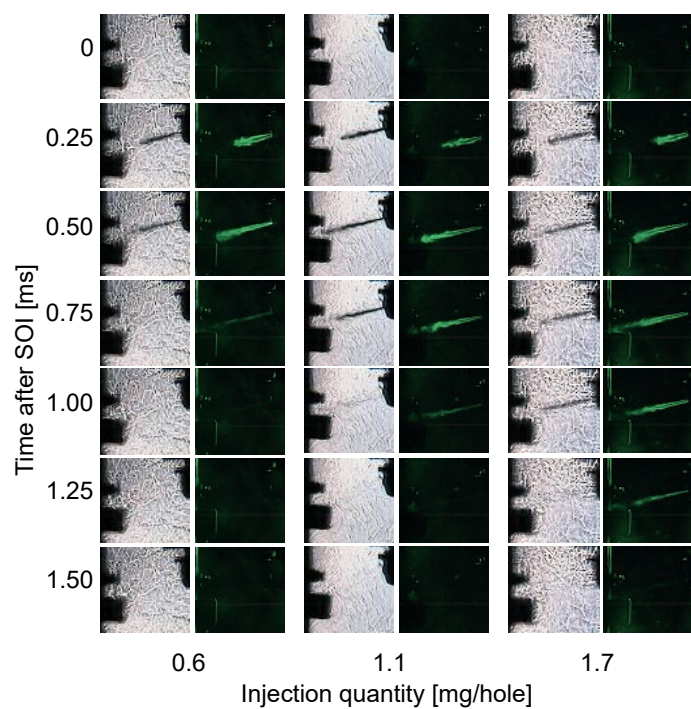
Figure 17. Observation of spray penetration and wall impingement at 30 CA ATDC (left: shadowgraph, right: Mie scattering)
