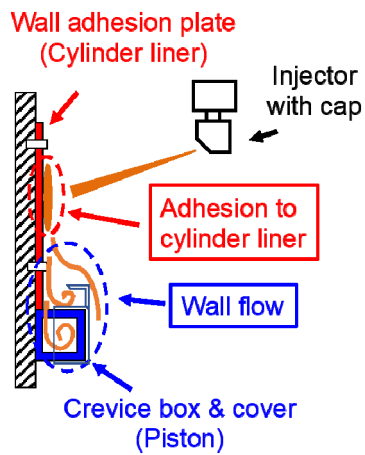
Figure 4. Outline of the fuel adhesion attachment used to measure fuel adhering to the wall and the fuel flow entering the crevice
