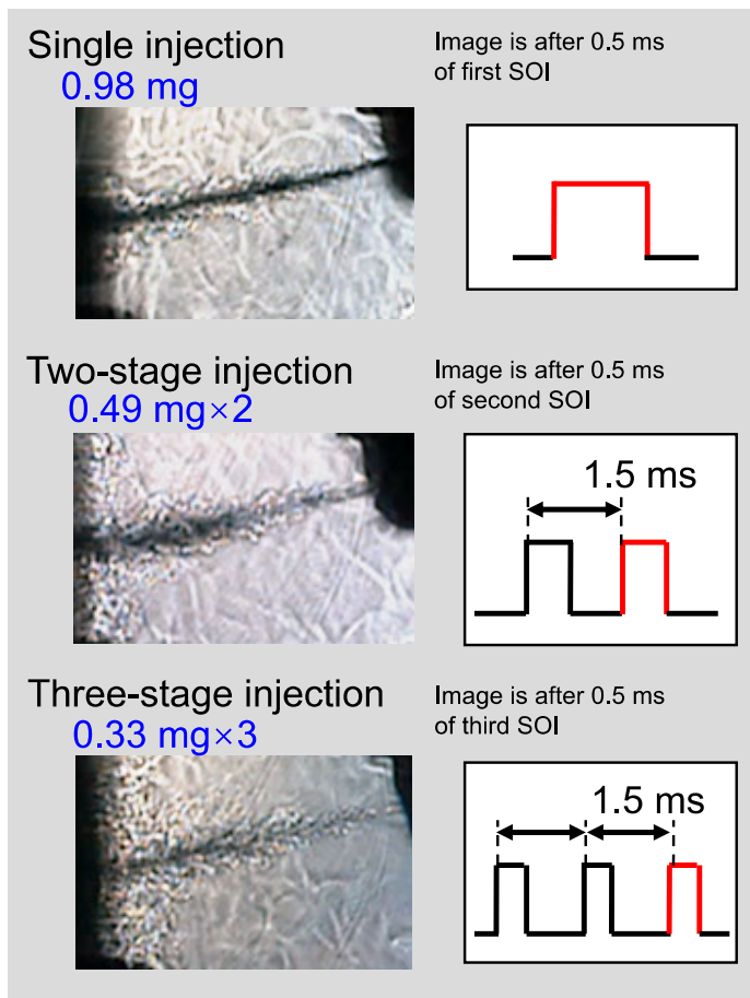
Figure 30. Images of single injection spray, second spray of two-stage injection, and third spray of three-stage injection 0.5ms after the start of injection (SOI)
