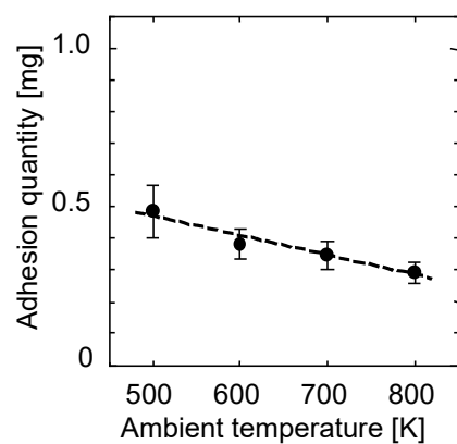
Figure 28. Effect of in-cylinder temperature on fuel wall adhesion
