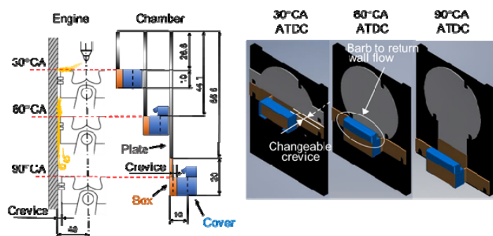
Figure 5. Different fuel adhesion attachments for different crank angles
