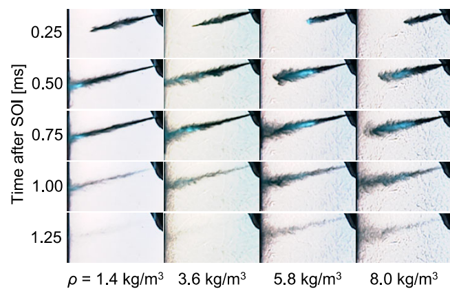
Figure 25. Effect of in-cylinder gas density on fuel spray behavior (test condition as in Table 5)
