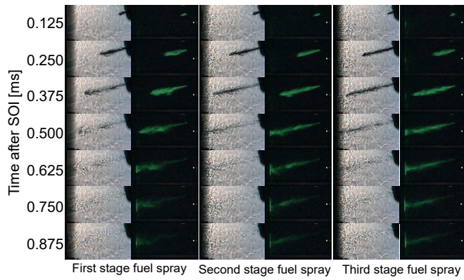
Figure 31. Shadowgraph and Mie scattering images of first, second, and third sprays of three-stage injections
