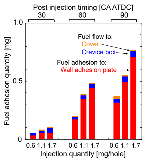
Figure 22. Mass of fuel adhering walls and fuel wall flow entering the crevice
