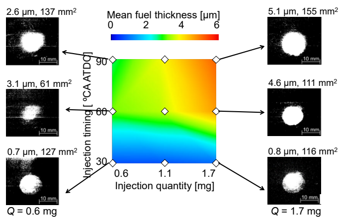
Figure 21. Fuel adhesion area and fuel film mean thickness (Wall adhesion)
