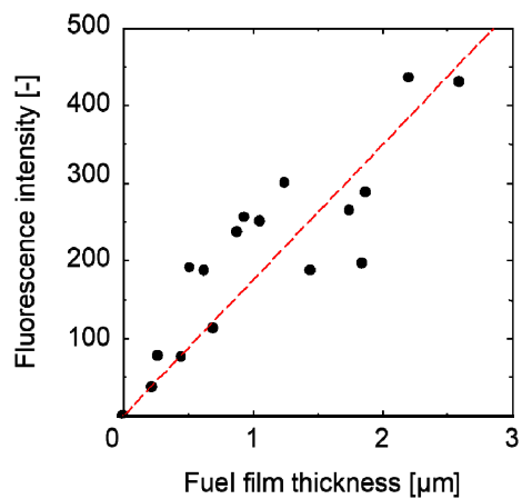
Figure 10. Calibration plot with curve of fluorescence intensity to fuel film thickness at room temperature
