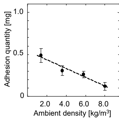
Figure 26. Effect of in-cylinder gas density on fuel wall adhesion (test condition as in Table 5)
