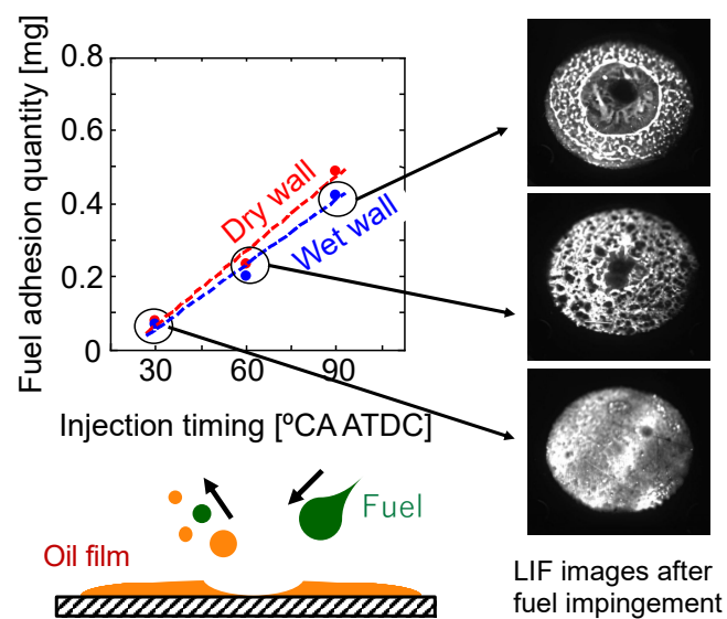
Figure 16. Fuel wall adhesion quantities with and without lubricant oil film (Fuel injection quantity: 1.1mg/hole)
