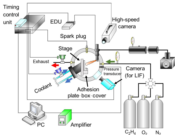
Figure 2. Experimental set-up
