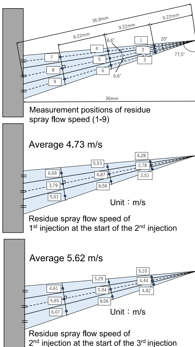
Figure 32. Residue spray flow speed of 1 st and 2 nd injections at the start of 2 nd and 3 rd injections
