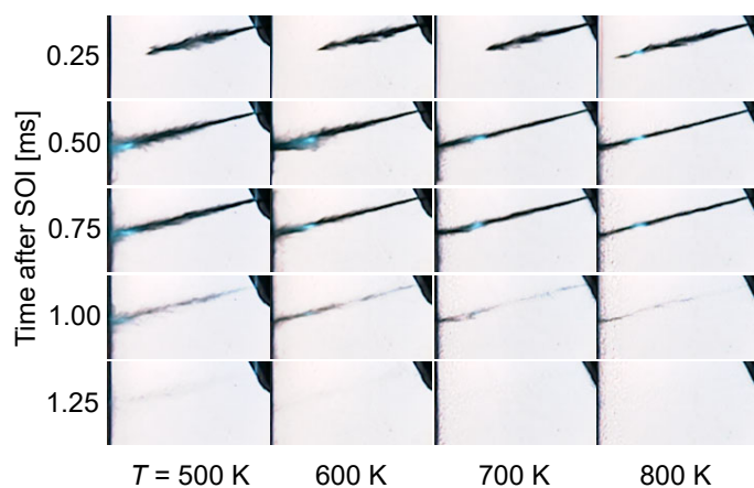
Figure 27. Effect of in-cylinder temperature on fuel spray behavior (test condition is shown in Table 5)
