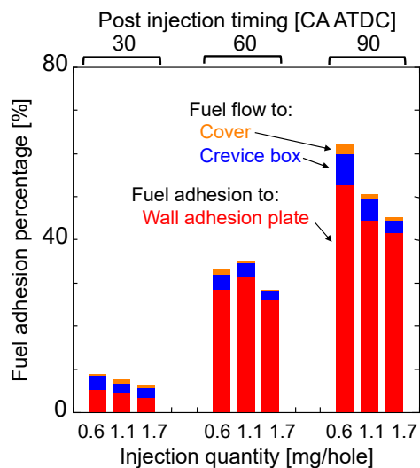
Figure 23. Percentage of fuel adhering walls and fuel wall flow entering the crevice
