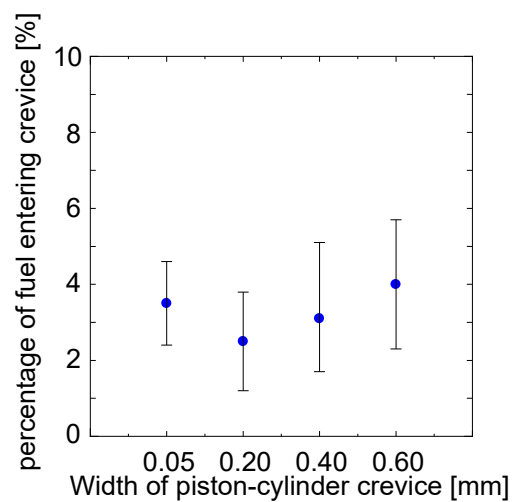
Figure 24. The percentage of fuel entering the piston-cylinder crevice at different crevice widths (injection quantity: 1.1 mg/hole, pressure: 0.4 MPa, temperature: 590 K, density: 2.4 kg/m 3 (60 CA ATDC condition))
