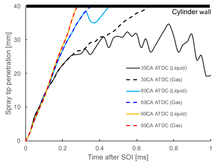
Figure 20. Plots of 1.1 mg fuel spray penetration at 30, 60, and 90CA ATDCs
