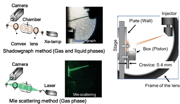
Figure 9. Outline of set-up and images of shadowgraph and Mie scattering observations
