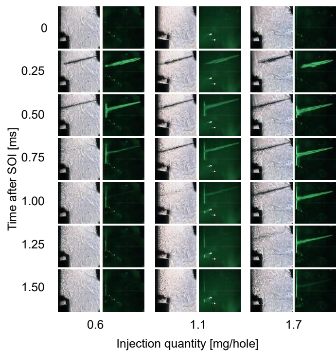
Figure 18. Observation of spray penetration and wall impingement at 60 CA ATDC (left: shadowgraph, right: Mie scattering)
