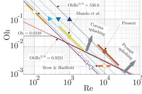
FIG. 5. Criteria for corona splashing at atmospheric conditions are plotted with the criteria for prompt splashing: Oh Re^{0.609} = 0.8458 [35] (· · ·); Oh Re^{5/8} = 0.207(\mu/\mu_g)^{3/8} [37] (—). Criteria for prompt splashing are plotted: Oh Re^{1.25} = K_p [12] with Eq. (2) for S_a = 1.0 \times 10^{-6} (—▲—), S_a = 1.0 \times 10^{-5} (—▼—), S_a = 1.0 \times 10^{-4} (—◆—), S_a = 1.0 \times 10^{-3} (—△—), S_a = 1.0 \times 10^{-2} (—▽—), and S_a = 1.0 \times 10^{-1} (—▷—). The ranges of our experimental results (Fig. 4) are plotted (—●—), with those of previous experimental results: Stow and Hadfield [11] (—○—); Mundo et al. [12] (—□—) and (—■—).
