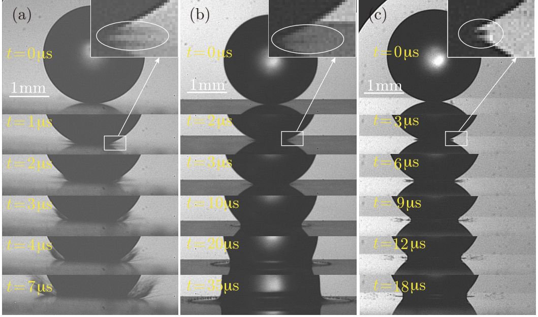
FIG. 2. Splashing after impact. (a) Type-I and type-III splashing: P = 75.1 kPa, V = 25.8 m/s, and D = 2.42 mm. (b) Type-II and type-III splashing: P = 64.5 kPa, V = 14.8 m/s, and D = 2.35 mm. (c) Type-III splashing with subsequent smooth liquid film flow: P = 0.8 kPa, V = 9.64 m/s, and D = 2.27 mm. A magnified image of type-III splashing is also shown in the rectangle in the upper right corner of each image. Movies 1, 2, and 3 in the Supplemental Material [22] correspond to (a), (b), and (c), respectively.
