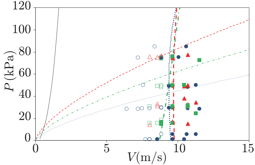
FIG. 1. Prompt splashing at P=1, 5, 15, 30, 50 , and 75 kPa in air (●, ○), He (▲, △) and \text{CO}_2 (■, □) with respect to V and P . The filled and open symbols indicate whether prompt splashing is observed or not, respectively. The criteria are shown by the blue dotted (···), red dashed (---), and green dot-dash (- · -) lines for air, He, and \text{CO}_2 , respectively. The Stokes number at V=10 m/s in air is 1.70 \times 10^{-6} . The condition where \epsilon=1 is shown with a black line and where \text{Kn}=1 are shown with thin dotted (···), thin dashed (---), and thin dot-dash (- · -) lines for air, He, and \text{CO}_2 , respectively.
