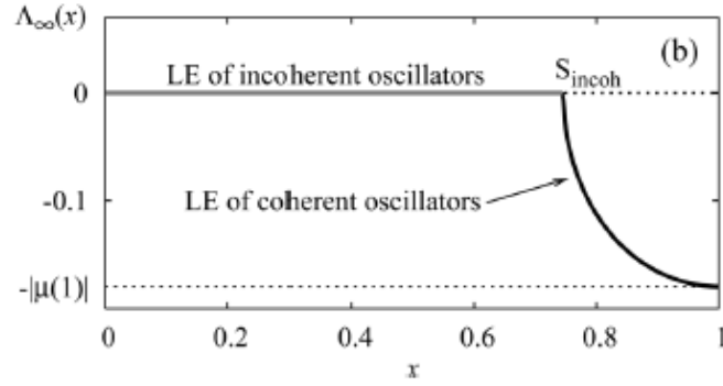
Figure 3.8: Lyapunov spectra \Lambda_\infty(x) of the chimera state in N \rightarrow \infty . Parameters are the same as those in Fig. (3.7) [9].
