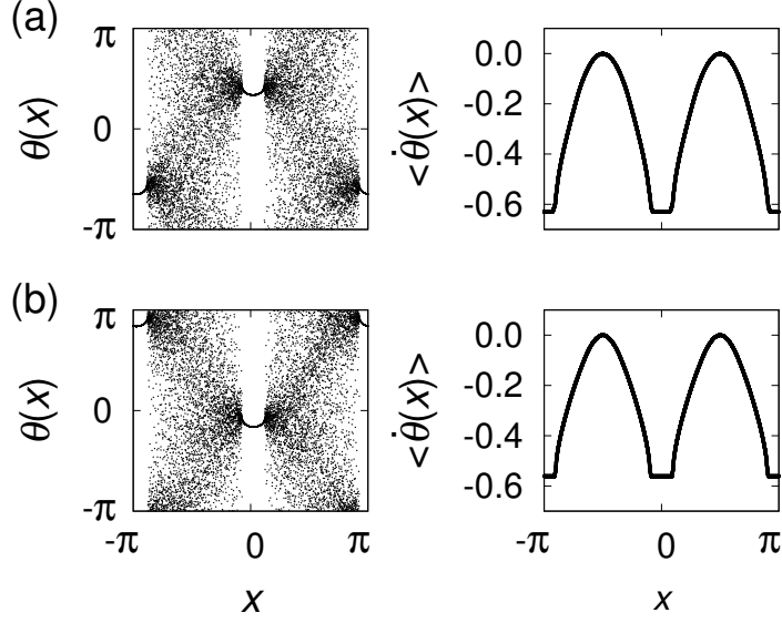
Figure 5.1: Multichimera state with two coherent and incoherent regions for Eq. (5.1) with N = 100000 and \alpha = 1.480 . In each row, the left panel shows the snapshot of the phase \theta(x, t) , and the right panel shows the profile of the average frequency \langle \dot{\theta}(x) \rangle with T = 2000 . (a) The breathing multichimera appears for s = 0.360 , while (b) the stationary multichimera appears for s = 0.440 . All figures are plotted once every 10 oscillators.
