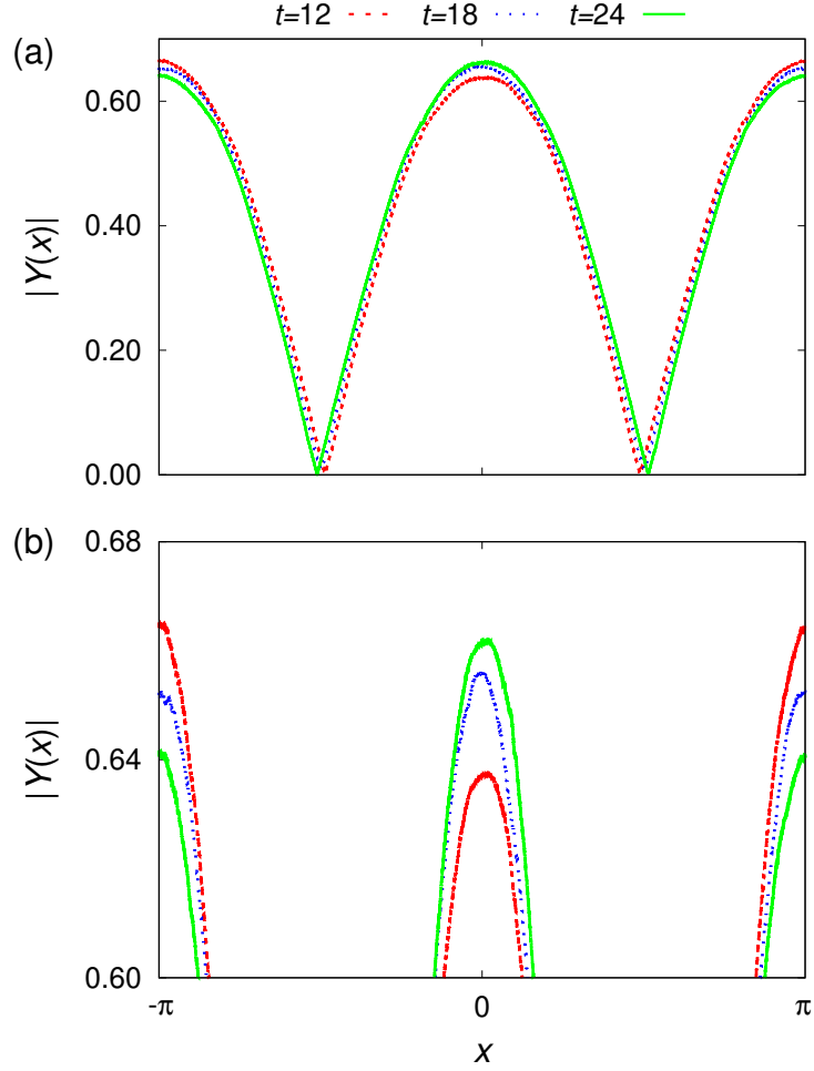
Figure 5.6: Snapshot of the local mean field |Y(x, t)| for the breathing multichimera in Fig. 5.1. (a) The global view of the snapshot; (b) the upper enlarged view. The red dashed line ( t = 12 ) and green solid line ( t = 24 ) approximately correspond to peaks of |Z(t)| , while the blue dotted line ( t = 18 ) approximately corresponds to a valley, as shown in Fig. 5.4 [22].
