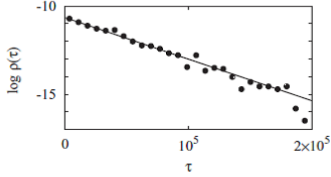
Figure 3.10: Histogram of lifetimes \tau of chimera states obtained by 2000 numerical simulations (circles). The data is plotted in logarithmic scale with fitted exponential distribution (solid line). Parameters are the same as those in Fig. (3.9) [10].
