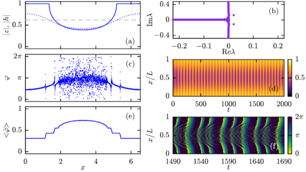
Figure 6.1: Breathing chimera state with phase lag parameter heterogeneity \alpha = \alpha_0 + \alpha_1|Y(x, t)|^2 with \alpha_0 = 0.3\pi and \alpha_1 = 0.65 . (b) All eigenvalues for the unstable stationary chimera state. (c) The snapshot of the phase \varphi(x, t) . (e) The profile of the average frequency \langle \dot{\varphi} \rangle . The details of figures (a), (d), and (f) are omitted [21].
