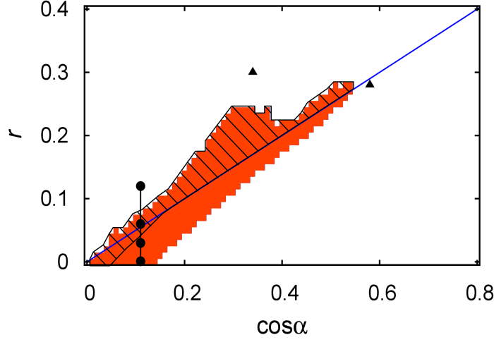
Figure 4.7: Stability region of the chimera state on the (\cos \alpha, r) plane for N = 2000 (red region). In the hatched region, there appear the persistent chimera state that is stable for N = 30 at least. The blue line denotes r = (\cos \alpha)/2 , and the completely synchronous solution is stable for r < (\cos \alpha)/2 . Black circles and triangles denote the parameter values of Fig. 4.2 and Fig. 4.9, respectively [16].
