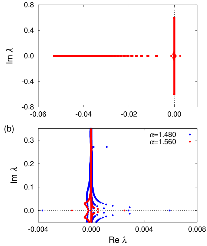
Figure 5.13: Complex eigenvalues \lambda of L_d with M = 5000 , s = 0.360 , and \alpha = 1.560 . Figure (a) shows all eigenvalues. Figure (b) is the enlarged view of (a), and the blue points denotes eigenvalues for \alpha = 1.480 corresponding to Fig. 5.10.
