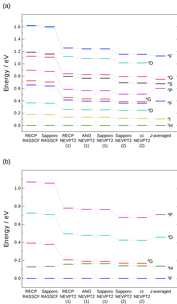
Figure 3-1. The calculated energy levels for the low-lying electronic states of \text{Ce}^+ that originate from (a) the ground-state configuration, [\text{Xe}]4f^1 5d^2 , and (b) the excited-state configuration, [\text{Xe}]4f^1 5d^1 6s^1 ; the correlated orbitals in NEVPT2 calculations are (1) 4f , 5sp , and 6s and (2) 4spdf , 5sp , and 6s . The available experimental J -averaged values [13] are also shown.
