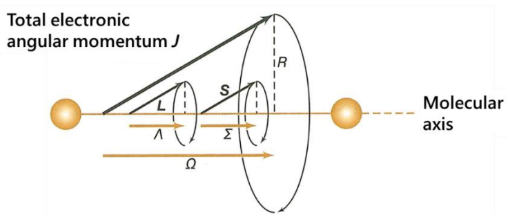
Figure 2-1. The schematic diagram of quantum number \Omega [5].
