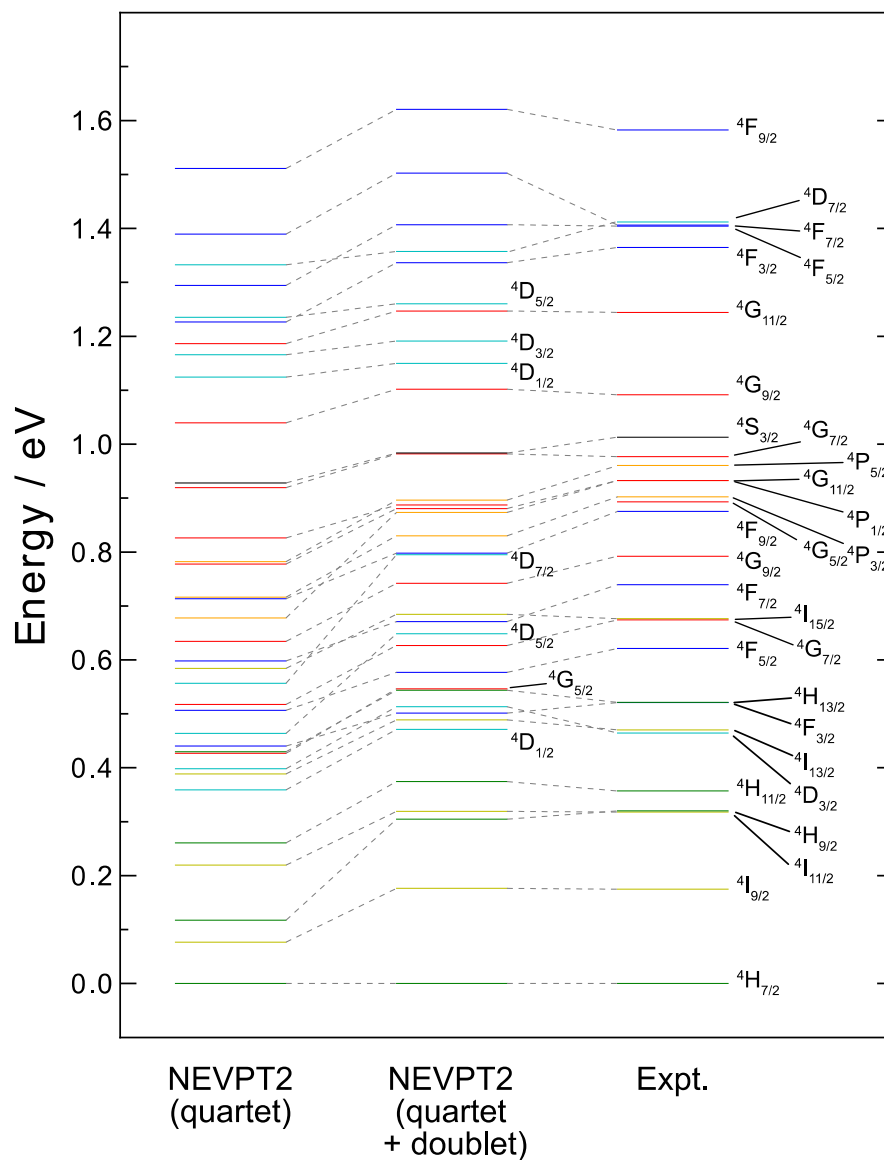
Figure 3-5. The NEVPT2 and experimental [13] energy levels of the ground and low-lying excited states of \text{Ce}^+ which originate from the ground-state configuration ([\text{Xe}]4f^1 5d^2) . As for NEVPT2 results, two different calculated results are shown (SA-RASSCF/NEVPT2 for quartet and SA-CASSCF/NEVPT2 for quartet and doublet) where the energy levels in the left (NEVPT2 (quartet)) are the same as those of the middle one in Figure 3-3.
