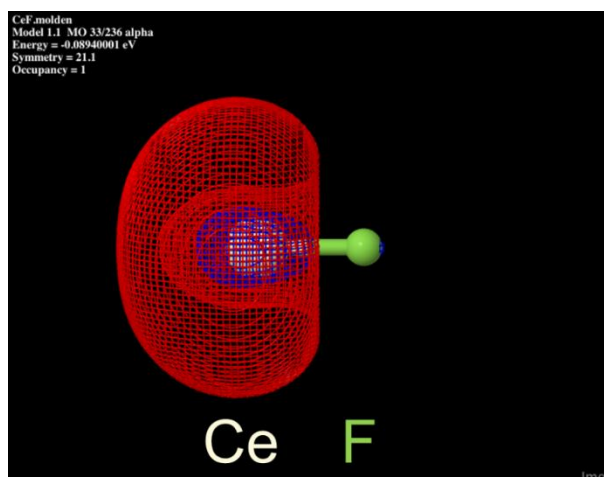
Figure 4-3. The molecular orbital for Ce-6s. The Coulomb repulsion from \text{F}^- can decrease by the 6s-6p hybridization where the electron in Ce-6s is able to extend to the other side of \text{F}^- .
