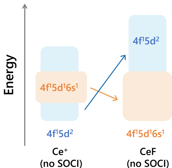
Figure 4-2. The schematic diagram for the change of the ground-state configuration in CeF, compared with \text{Ce}^+ .
