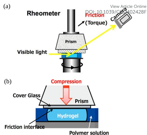
Fig. 1 Schematic illustration of the setup for the in-situ observation of the frictional interface between a gel and a glass during sliding friction measurement. (a) A parallel-plate rheometer was used. The trapezoidal prism was fixed to the upper plate of the rheometer, and a cover glass was fixed to the prism as the counter surface of friction. Hydrogel was bonded to the rotating lower plate of the rheometer. (b) The hydrogel was compressed in the polymer solution by the upper plate with a prism. The images of the frictional interface were recorded in situ by using a digital video camera set at an observation angle between the critical angles of polymer solution and gel.
