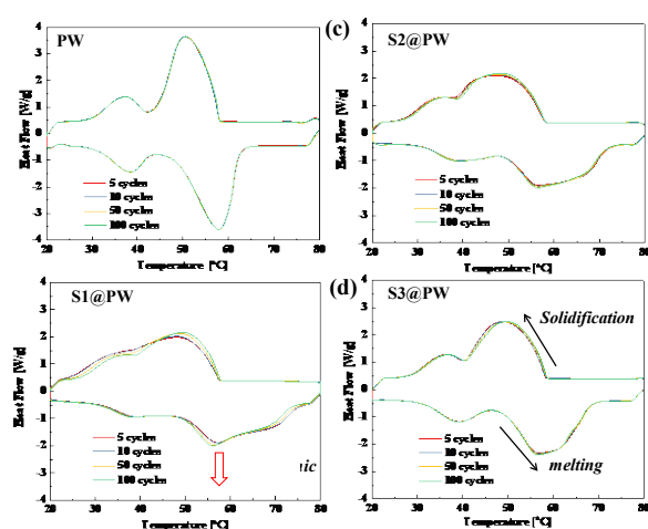
Figure 9. DSC curves of the heating and cooling process of PW and PCCs.
