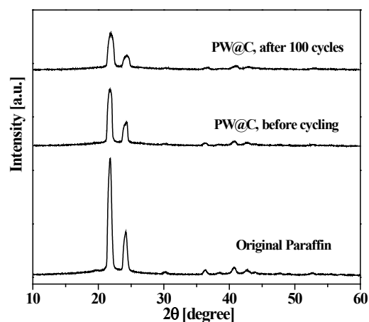
Figure 11. XRD patterns of PW and PW@C before/after cycling.
