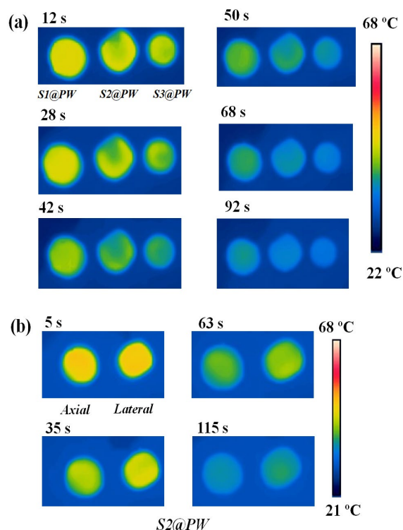
Figure 8. Thermal images of the samples during cooling. (a) Three composites from axial direction; (b) composite S2@PW from both axial and lateral directions.
