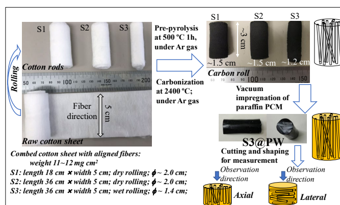
Figure 1. Schematic diagram for producing carbon fiber scaffolds and PCM/carbon composites.
