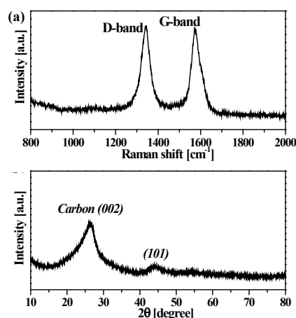
Figure 2. Raman spectrum (a) and XRD pattern (b) for the cotton-derived carbon at 2400 °C.
