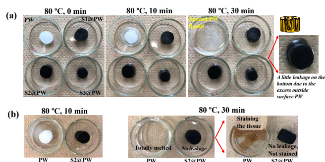
Figure 12. Leakage test of the PCCs and PW. The photographs for the samples heated at 80 °C to different durations are presented. (a) the PCCs were prepared with some excess surface PW, showing a little leakage on the bottom of PCCs after melting; (b) the PCC was prepared without excess surface PW, showing no leakage.
