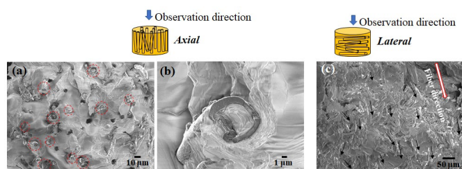
Figure 4. Typical SEM images of the paraffin/carbon composites observed from the axial block (a, b) and lateral block (c).
