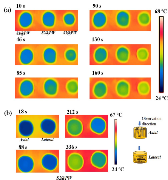
Figure 7. Thermal images of the samples during heating. (a) Three composites from axial direction; (b) composite S2@PW from both axial and lateral directions.
