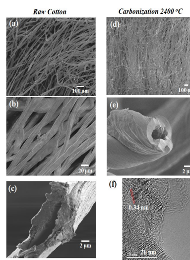
Figure 3. Morphology and structural analysis. SEM images of the original cotton fibers (a, b, c) and carbon obtained at 2400 °C (d, e). (f) is the high resolution TEM image of the carbon.
