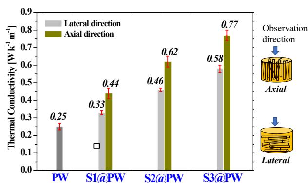
Figure 6. Thermal conductivity of the PCCs in comparison with PW. The thermal conductivity for the PCCs along the axial direction (fiber direction) and lateral direction were compared. Inset shows the average values for each sample.
