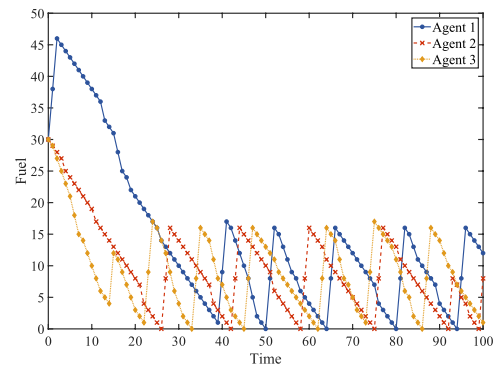
Fig. 6 Time response of the fuel in Case 2.
