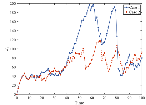
Fig. 7 Time response of J_s (the sum of penalties).
