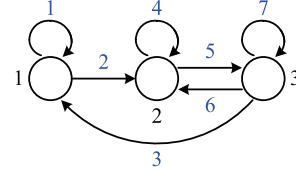
Fig. 2 Example of directed graphs. The number assigned to each arc represents the element in the arc set \{1, 2, \dots, |\mathcal{E}|\} .
