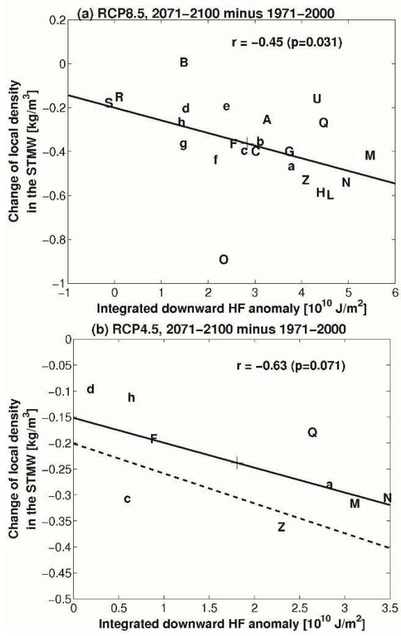
Figure 2.11. Scatter diagram of epoch differences of the local density averaged in the STMW region ( 145^{\circ} – 170^{\circ}\text{E} , 25^{\circ} – 35^{\circ}\text{N} , and depth 50–300 m) and integrated downward net heat flux averaged south of the KE ( 130^{\circ} – 160^{\circ}\text{E} , 25^{\circ} – 35^{\circ}\text{N} ) among climate models between 1971–2000 and 2071–2100 periods. The scenarios are (a) RCP8.5 and (c) RCP4.5. The plus symbols (+) and alphabetical letters denote MME and the models (Table 1), respectively. Correlation coefficients and p -values are shown. Solid lines indicate the regression line from the data points. The dashed line in (b) is the regression line from (a).
