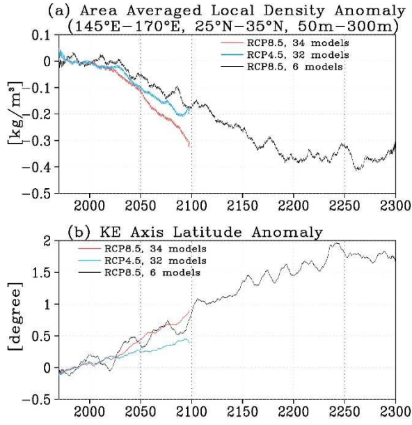
Figure 2.5. Time series of (a) local density anomaly averaged in the STMW region (145°–170°E, 25°–35°N, and depth 50–300 m) and (b) the KE-axis latitude anomaly smoothed by applying an 11-year running mean for 34-model MME under RCP8.5 (red), 32-model MME under RCP4.5 (blue), and 6-model MME under RCP8.5 (black).
