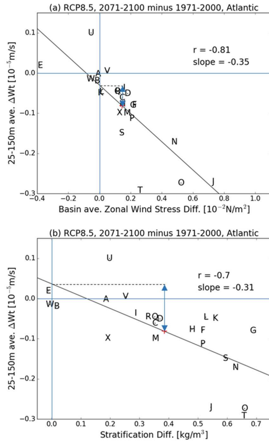
Figure 3.6. (a) Same as Fig. 3.4a, but for area-averaged total upwelling in the Atlantic (40°W–20°W at depths of 25–150 m along the equator) and Atlantic basin-averaged zonal wind stress (60°W–10°E). (b) Same as (a), but for area-averaged upwelling (40°W–20°W at 25–150 m depth along the equator) and basin-averaged stratification (60°W–10°E along the equator between the surface and a depth of 100 m).
