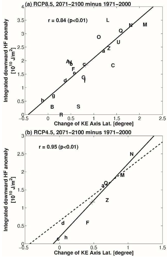
Figure 2.12. As in Fig. 2.11, but for epoch differences of the KE-axis latitude and integrated downward net heat flux averaged south of the KE ( 135^{\circ} – 145^{\circ} E, 30^{\circ} – 35^{\circ} N) among climate models. The dashed line in (b) is the regression line from (a).
