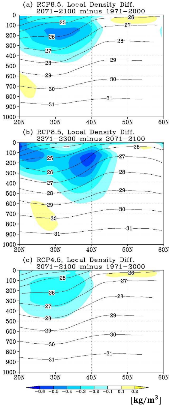
Figure 2.4. Zonally averaged ( 145^{\circ} – 170^{\circ} E) local density differences (color) (a) between 1971–2000 and 2071–2100 periods for 34-model MME under RCP8.5, (b) between 2071–2100 and 2271–2300 periods for 6-model MME under RCP8.5, and (c) between 1971–2000 and 2071–2100 periods for 32-model MME under RCP4.5. Local density is defined as the deviation from global mean density at each level (see text). Contours indicate the mean \sigma for the periods (a,c) 1971–2000 and (b) 2071–2100.
