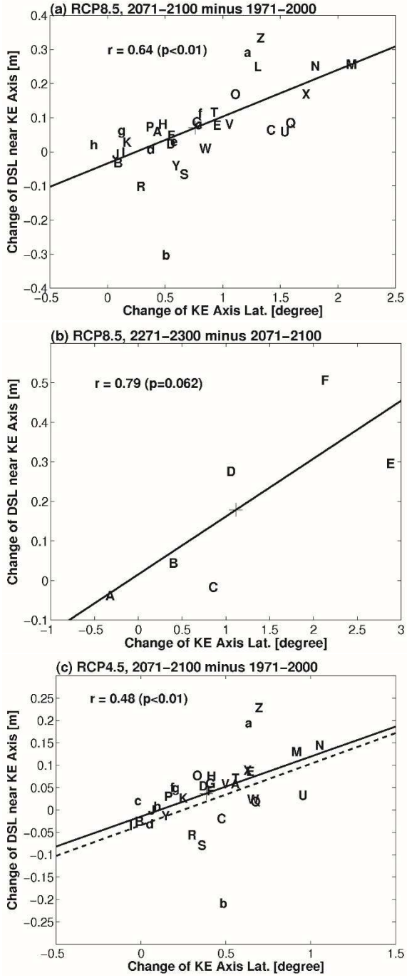
Figure 2.7. As in Fig. 2.6, but for epoch differences of KE axis latitude and DSL around the KE axis ( 145^{\circ} – 170^{\circ} E, 35^{\circ} – 40^{\circ} N) among climate models. The dashed line in (c) is the regression line from (a).
