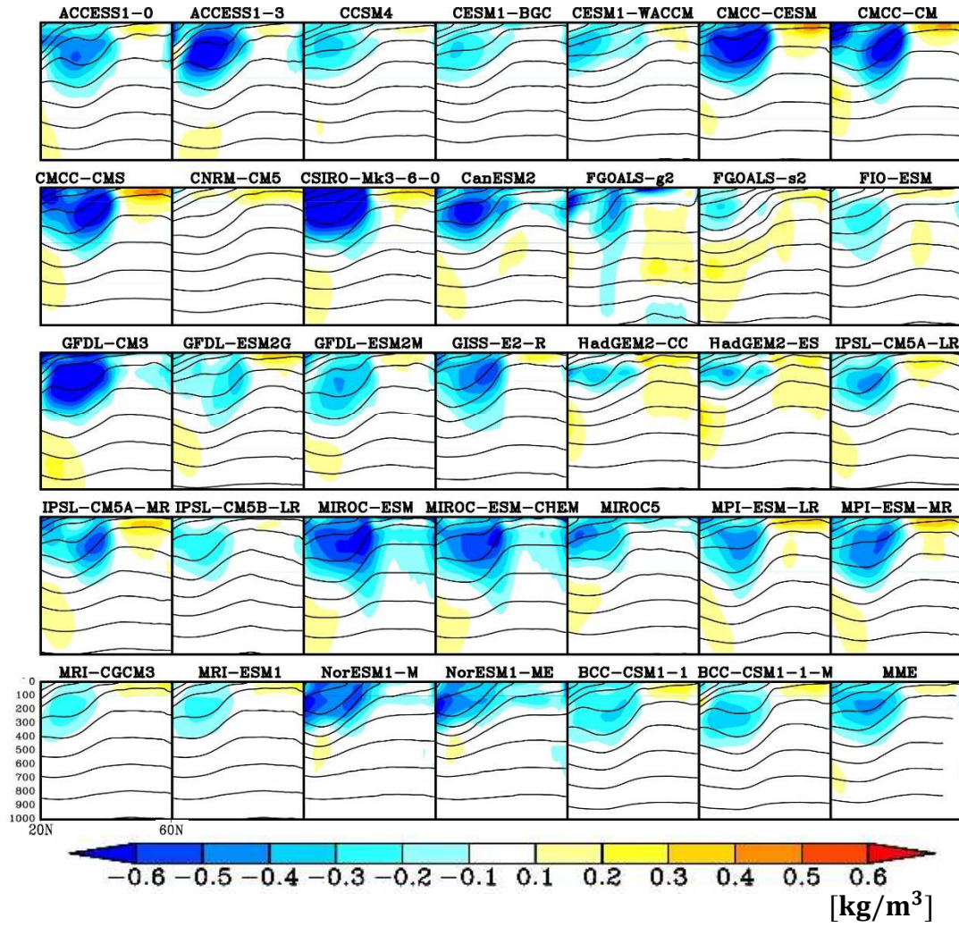
Figure 2.17. Zonally averaged (145°–170°E) local density differences between 1971–2000 and 2071–2100 periods under RCP8.5 for each model (color). Contours indicate the mean \sigma for the period 1971–2000. MME indicates the MME mean.
