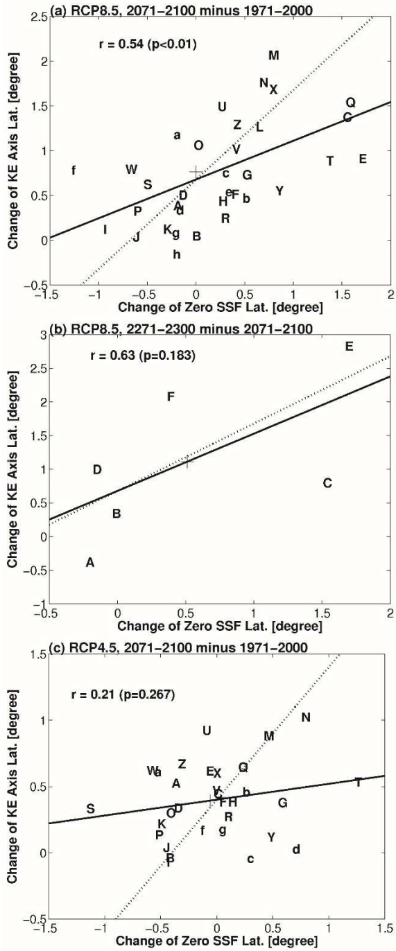
Figure 2.14. As in Fig. 2.6, but for epoch differences of the KE-axis latitude and the latitude of zero SSF at 150°E among climate models. Dotted lines indicate slope 1.
