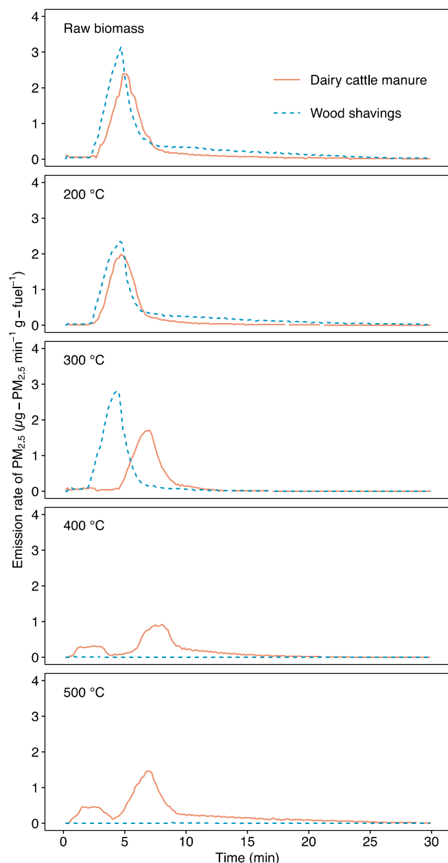
Fig. 2. Rates of PM_{2.5} emission from raw biomass and biochar at a combustion temperature of 850 °C. The temperature values indicated in the figure represent the pyrolysis temperature.
