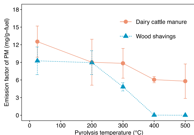
Fig. 3. Total PM emission factors for raw biomass (25 °C) and biochar at a combustion temperature of 850 °C.
