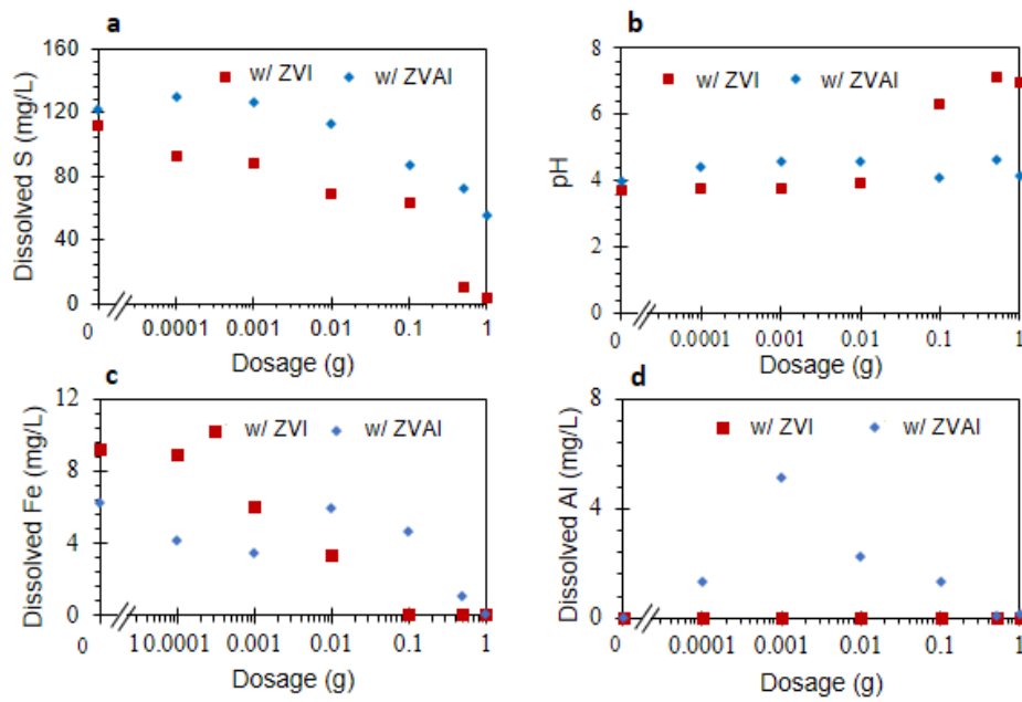
Fig. 2.2 Leaching of pyrite with various dosage of ZVAl or ZVI: (a) dissolved S concentration after leaching, (b) pH of the solution after leaching, (c) dissolved Fe concentration after leaching, and (d) dissolved Al concentration after leaching.
