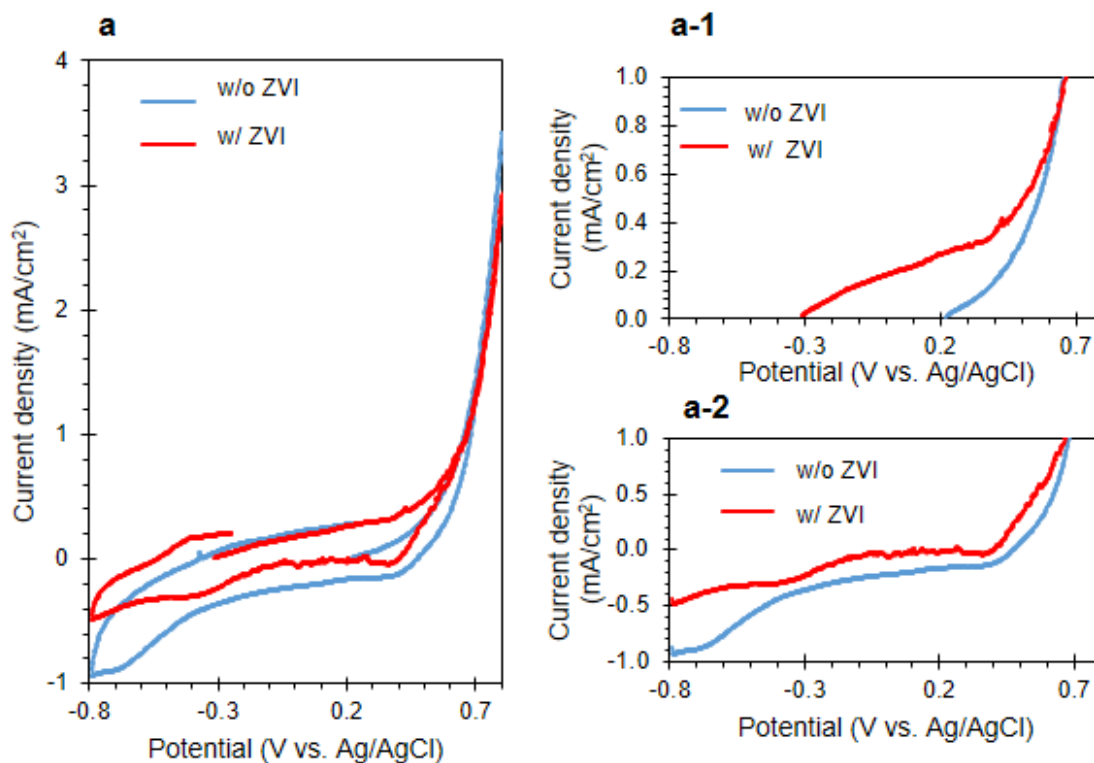
Fig. 2.9 Cyclic voltammetry of pyrite with and without attached with ZVI: (a-1) anodic sweep of the first cycle, and (a-2) cathodic sweep of the first cycle.
