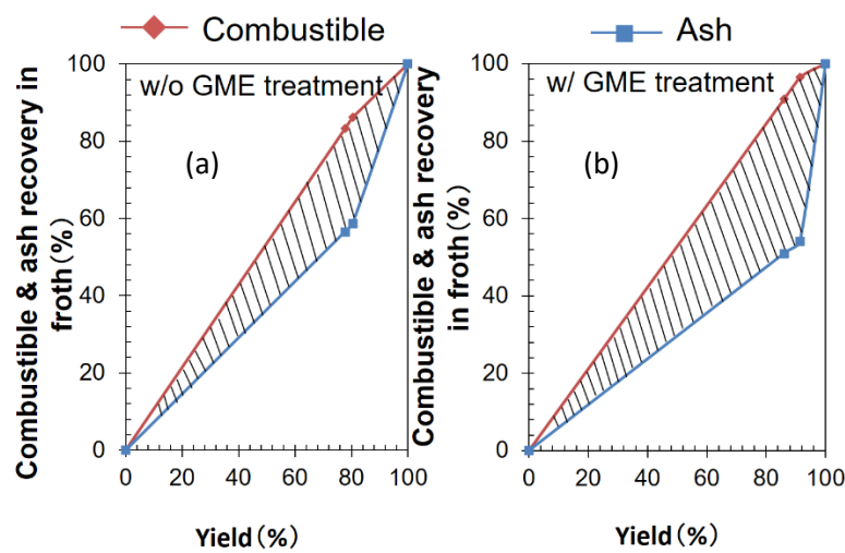
Fig. 4. 4 Combustible and ash recovery of coal (a) without and (b) with GME treatment.
