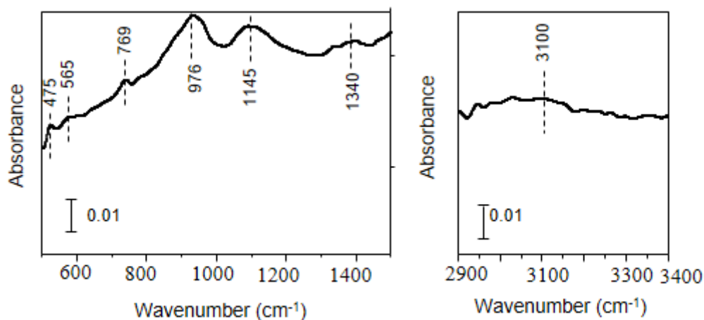
Fig. 2.7 ATR-FTIR spectrum of ZVAI used in the experiment.
