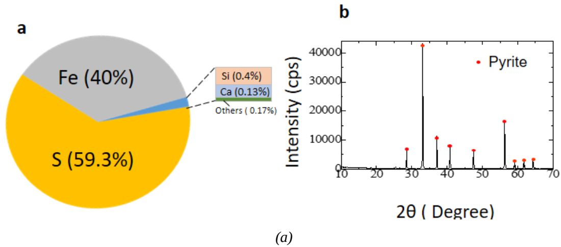
Fig. 3. 1 (a) The chemical composition and, (b) XRD pattern of pyrite sample.
