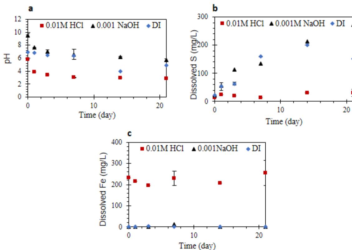
Fig. 2.6 Evolution of leachate chemistry in deionized (DI) water, 0.01M HCl, and 0.001M NaOH as well as the zeta-potential distributions of pyrite and ZVI with pH: (a) pH change with time (b) dissolved S concentration change with time, and (c) dissolved Fe concentration change with time.
