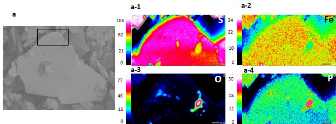
Fig. 4. 3 SEM-EDX photomicrograph of pyrite after leaching for 1 day with DI water and the corresponding elemental maps of (a-1) S, (a-2) Fe, (a-3) O, and (a-4) P.
