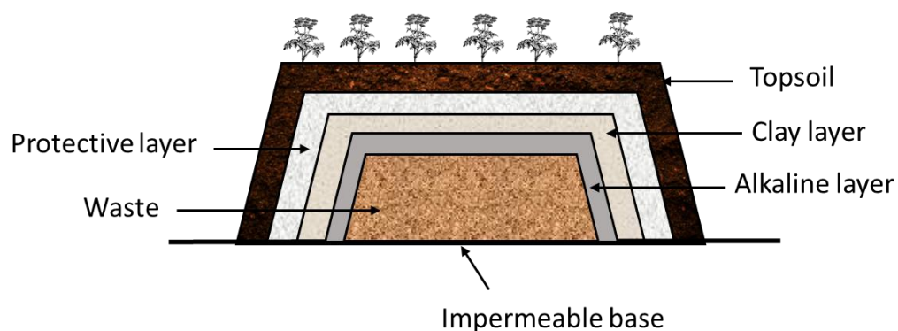
Fig. 1.1 Layout of a dry cover.
