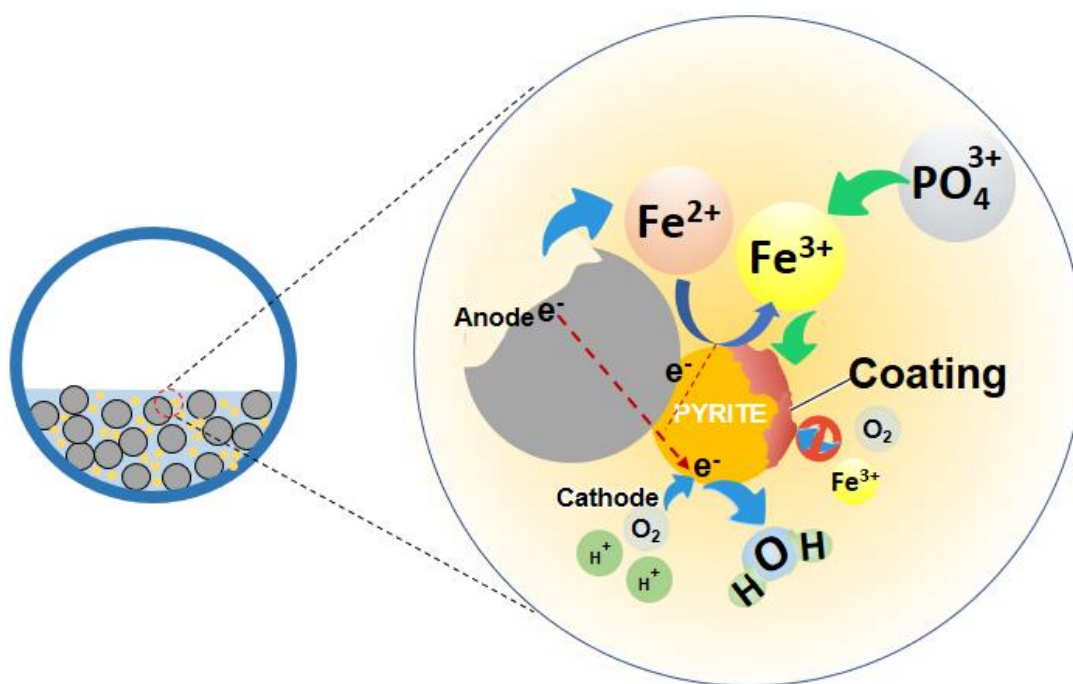
Fig. 4.1 A schematic diagram of galvanic interaction between steel balls and pyrite inside the ball mill.
