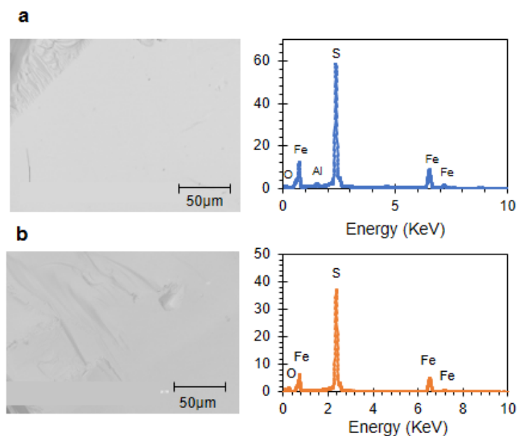
Fig. 2.5 SEM-EDX of pyrite after leaching with ZVAl or ZVI: (a) leaching with ZVAl for 3 days, and (b) leaching with ZVI for 3 days.
