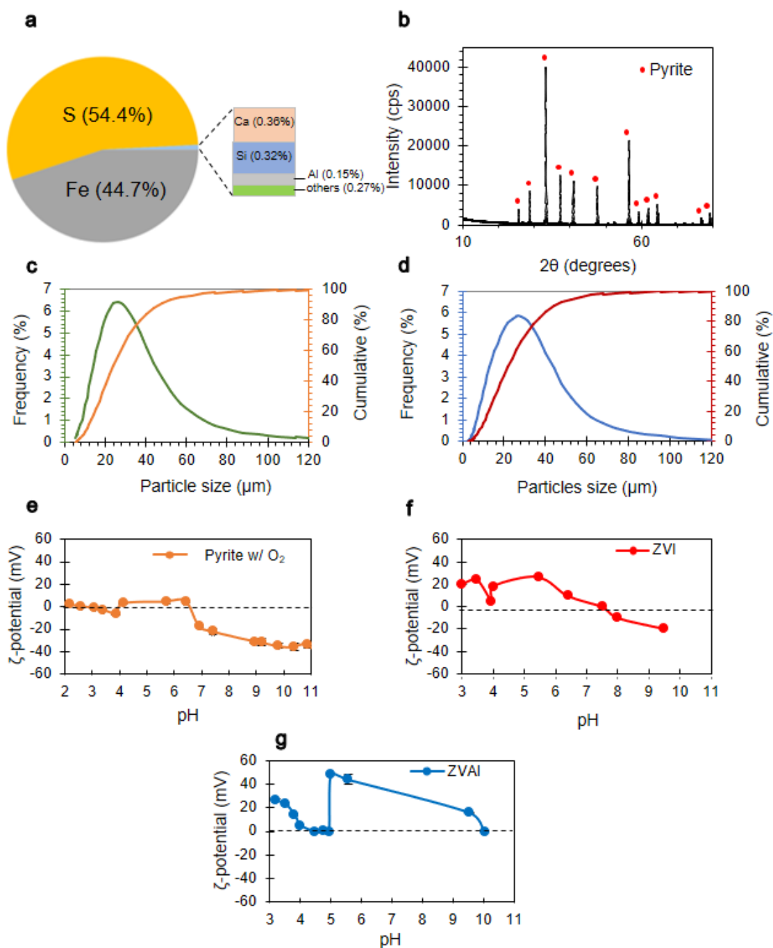
Fig. 2.1 (a) Chemical composition of pyrite sample, (b) XRD pattern of pyrite sample, (c) particle size distribution of ZVAl, (d) particle size distribution of ZVI, (e) zeta potential distribution of pyrite with pH under oxidic (with \text{O}_2 ) condition, and (f) & (g) zeta potential distribution of ZVI and ZVAl with pH under oxidic (with \text{O}_2 ) condition, respectively.
