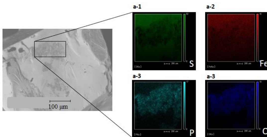
Fig. 3.6 SEM-EDX photomicrograph of pyrite residue.
