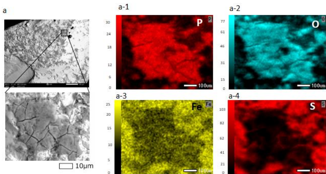
Fig. 3.3 SEM-EDX photomicrograph of pyrite after leaching for 7 days with phosphate solution and the corresponding elemental maps of (a-1) P, (a-2) O, (a-3) Fe, and (a-4) S.
