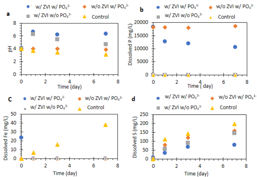
Fig. 3.2 Changes of (a) pH, (b) dissolved P, (c) dissolved Fe, and (d) dissolved S.
