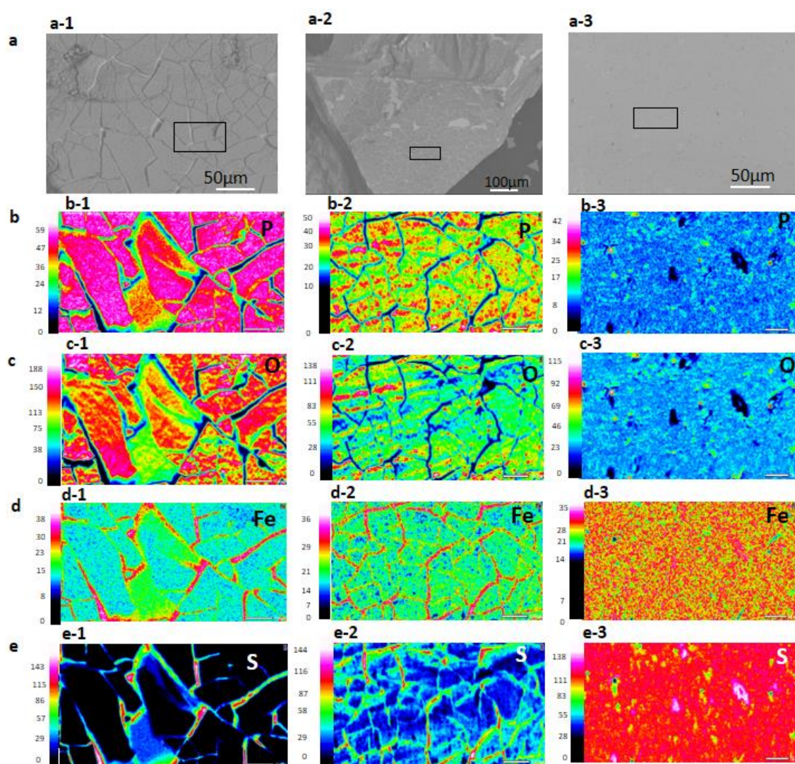
Fig. 3.5 SEM-EDX photomicrograph of pyrite residue in pH (a-1) 1.5 , (a-2) 3, and (a-3) 4, (b) elemental mapping of P in (b-1) pH 1.5, (b-2) pH 3, and (b-3) pH 4, (c) elemental mapping of O in (c-1) pH 1.5, (c-2) pH 3, and (c-3) pH 4, (d) elemental mapping of Fe in (d-1) pH 1.5, (d-2) pH 3, and (d-3) pH 4, and (e) elemental mapping of S in (e-1) pH 1.5, (e-2) pH 3, and (e-3) pH 4.
