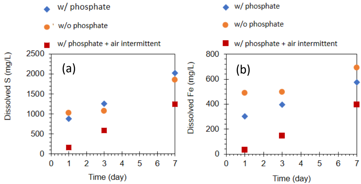
Fig. 4. 2 Change of (a) dissolved S, and (b) final Fe.
