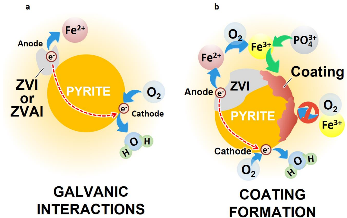
Fig. 1.4 Schematic diagram of (a) galvanic interaction, and (b) coating formation.
