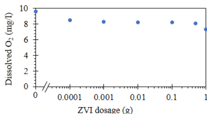
Fig. 2.3 Dissolved O 2 with various ZVI dosages.
