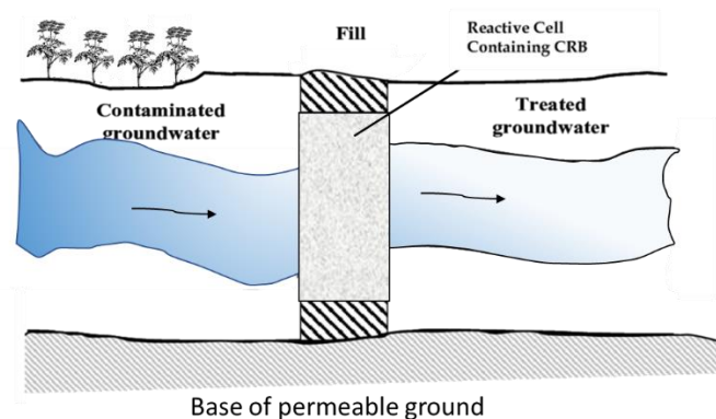
Fig. 1.3 Schematic cross-section of permeable reactive barrier (PBR). (Younger, 2000)
