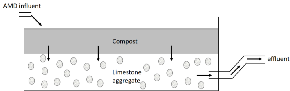
Fig. 1.2 Schematic layout of a reducing and alkalinity producing system (RAPS). (Younger et al., 2003)/
