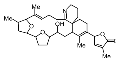
gymnodimine D ( 1-30 )
