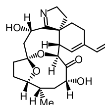
portimine ( 1-32 )
