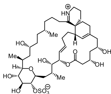
spiro-prorocentrimine ( 1-31 )
